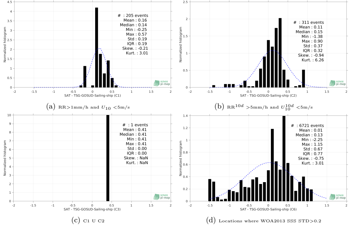
Figure 13: Normalized histogram of \Delta SSS (SMOS-L4-CATDS-CECOS-IFREMER-V2-WEEKLY-0.5DEG - TSG-GOSUD-Sailing-ship) for 6 different subdatasets corresponding to: RR > 1\text{mm/h} and U_{10} < 5\text{m/s} (a), RR^{10d} > 5\text{mm/h} and U_{10}^{10d} < 5\text{m/s} (b), C1 U C2 (c), Locations where WOA2013 SSS STD > 0.2 (d).
