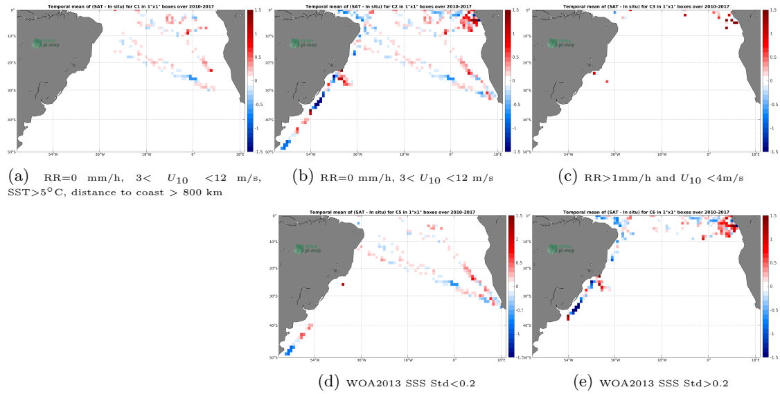
Figure 12: Temporal mean gridded over spatial boxes of size 1^\circ \times 1^\circ of \Delta SSS (SMOS L4 v2 Weekly (CATDS-CECOS-IFREMER) - TSG (GOSUD-Research-vessel)) for 5 different subdatasets corresponding to: RR=0 mm/h, 3 < U_{10} < 12 m/s, SST > 5^\circ C , distance to coast > 800 km (a), RR=0 mm/h, 3 < U_{10} < 12 m/s (b), RR > 1 mm/h and U_{10} < 4 m/s (c), WOA2013 SSS Std < 0.2 (d), WOA2013 SSS Std > 0.2 (e).
