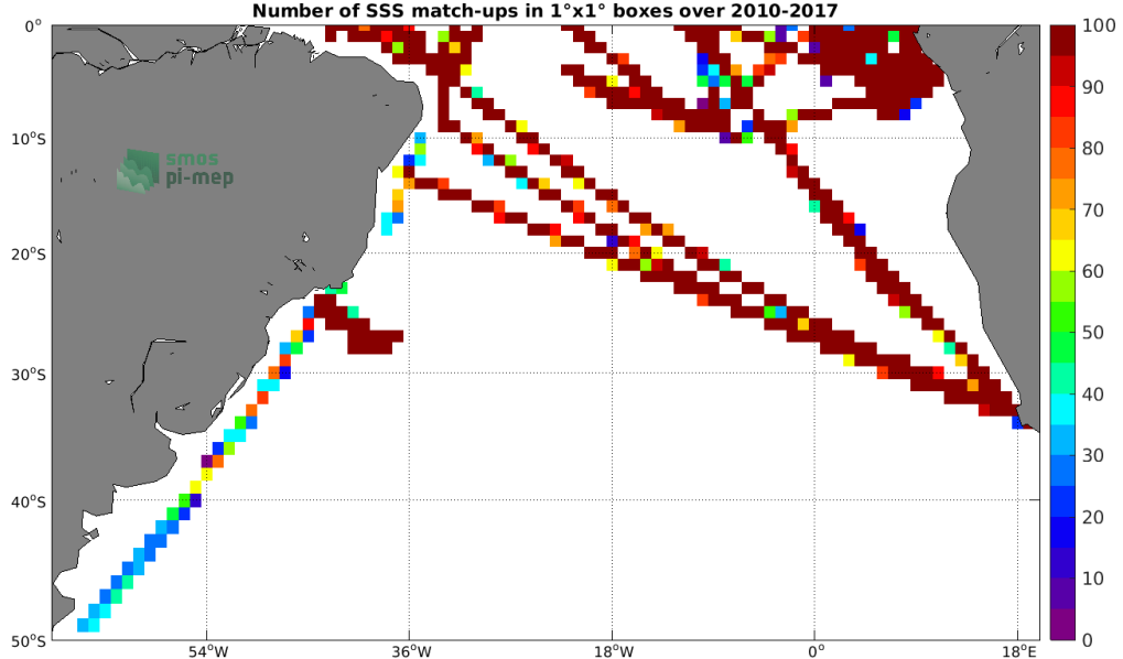
Figure 4: Number of SSS match-ups between TSG (GOSUD-Research-vessel) SSS and the SMOS L4 v2 Weekly (CATDS-CECOS-IFREMER) SSS product for the South Atlantic Ocean Pi-MEP region over 1^\circ \times 1^\circ boxes and for the full satellite product period.
