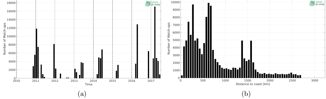
Figure 1: Number of match-ups between TSG (GOSUD-Research-vessel) and SMOS L4 v2 Weekly (CATDS-CECOS-IFREMER) SSS as a function of time (a) and as function of the distance to coast (b) over the South Atlantic Ocean Pi-MEP region and for the full satellite product period.
