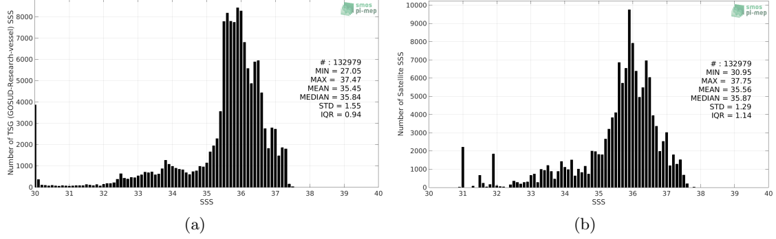
Figure 2: Histograms of SSS from TSG (GOSUD-Research-vessel) (a) and SMOS L4 v2 Weekly (CATDS-CECOS-IFREMER) (b) considering all match-up pairs per bins of 0.1 over the South Atlantic Ocean Pi-MEP region and for the full satellite product period.
