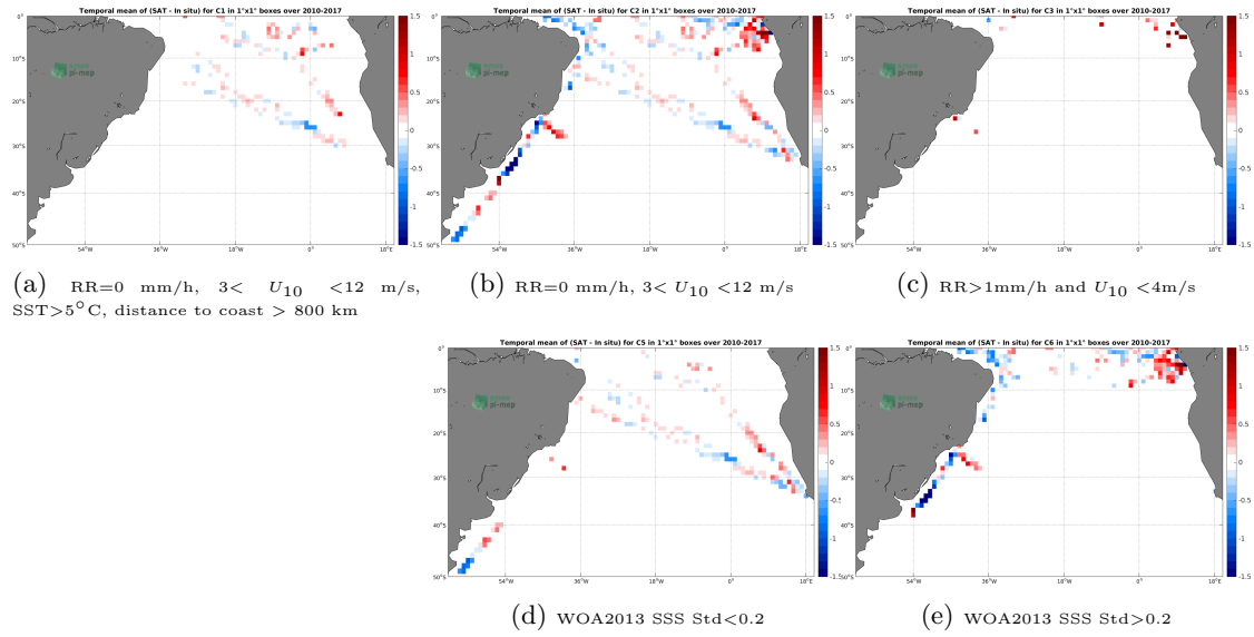
Figure 12: Temporal mean gridded over spatial boxes of size 1^\circ \times 1^\circ of \Delta SSS (SMOS-L4-CATDS-CECOS-IFREMER-V2-WEEKLY-0.5DEG - TSG-GOSUD-Research-vessel) for 5 different sub-datasets corresponding to: RR=0 mm/h, 3 < U_{10} < 12 m/s, SST > 5^\circ C , distance to coast > 800 km (a), RR=0 mm/h, 3 < U_{10} < 12 m/s (b), RR > 1 mm/h and U_{10} < 4 m/s (c), WOA2013 SSS Std < 0.2 (d), WOA2013 SSS Std > 0.2 (e).
