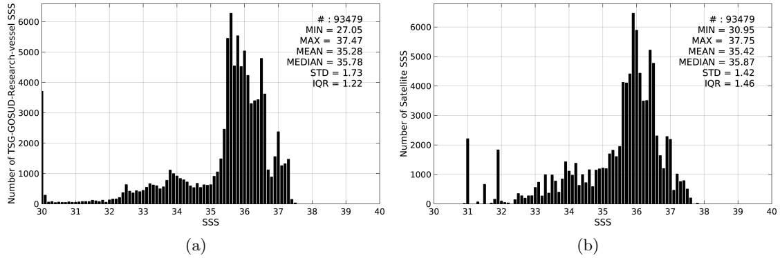
Figure 2: Histograms of SSS from TSG-GOSUD-Research-vessel (a) and SMOS-L4-CATDS-CECOS-IFREMER-V2-WEEKLY-0.5DEG (b) considering all match-up pairs per bins of 0.1 over the South Atlantic Ocean Pi-MEP region and for the full satellite product period.
