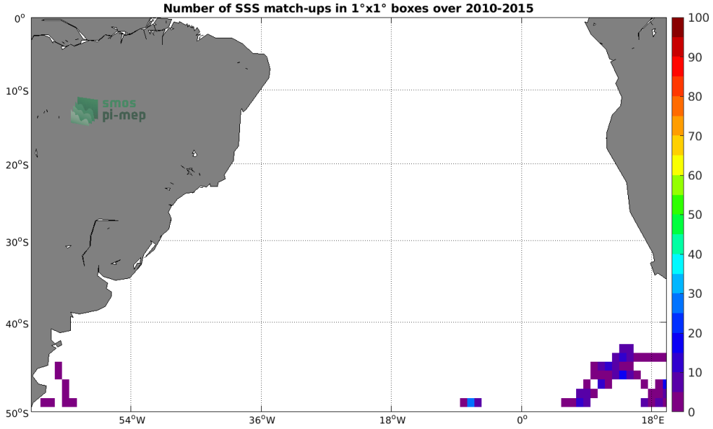
Figure 4: Number of SSS match-ups between Sea mammals SSS and the SMOS L4 v2 Weekly (CATDS-CECOS-IFREMER) SSS product for the South Atlantic Ocean Pi-MEP region over 1^{\circ} \times 1^{\circ} boxes and for the full satellite product period.
