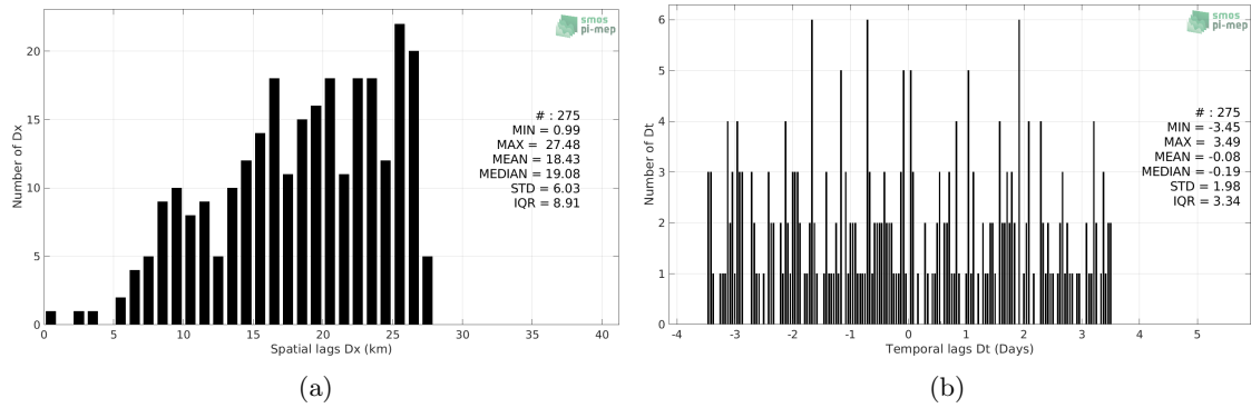
Figure 5: Histograms of the spatial (a) and temporal (b) lags between the location/time of the Sea mammals measurement and the date of the corresponding SMOS L4 v2 Weekly (CATDS-CECOS-IFREMER) SSS pixel.
