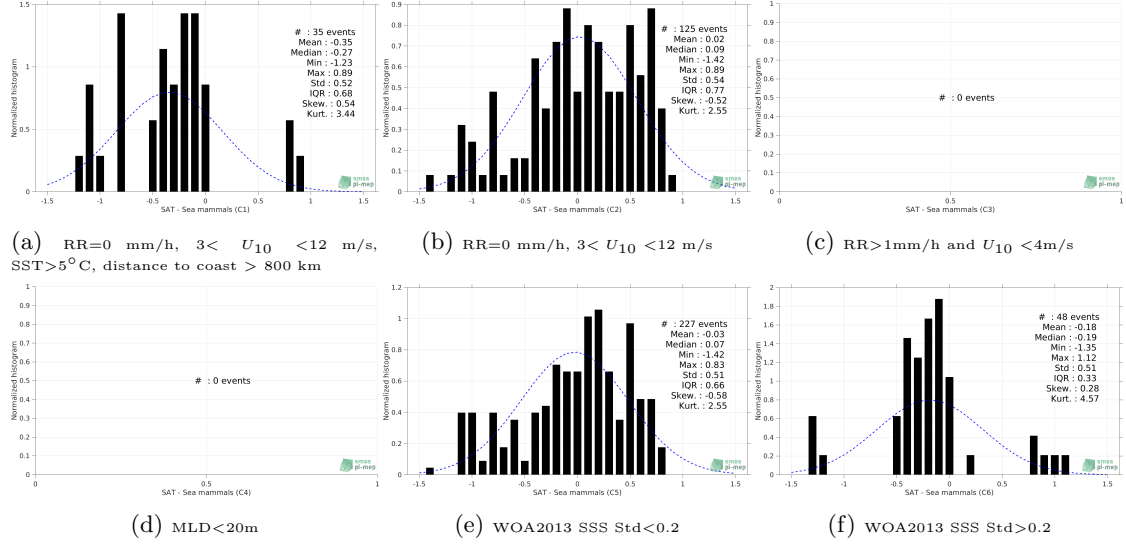
Figure 13: Normalized histogram of \Delta\text{SSS} (SMOS L4 v2 Weekly (CATDS-CECOS-IFREMER) - Sea mammals) for 6 different subdatasets corresponding to: RR=0 mm/h, 3 < U_{10} < 12 m/s, SST > 5^\circ\text{C} , distance to coast > 800 km (a), RR=0 mm/h, 3 < U_{10} < 12 m/s (b), RR > 1\text{mm/h} and U_{10} < 4\text{m/s} (c), MLD < 20\text{m} (d), WOA2013 SSS Std < 0.2 (e), WOA2013 SSS Std > 0.2 (f).
