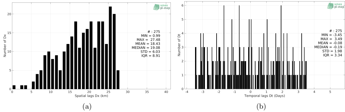
Figure 5: Histograms of the spatial (a) and temporal (b) lags between the time of the Sea mammals measurements and the date of the corresponding SMOS L4 v2 Weekly (CATDS-CECOS-IFREMER) SSS product.
