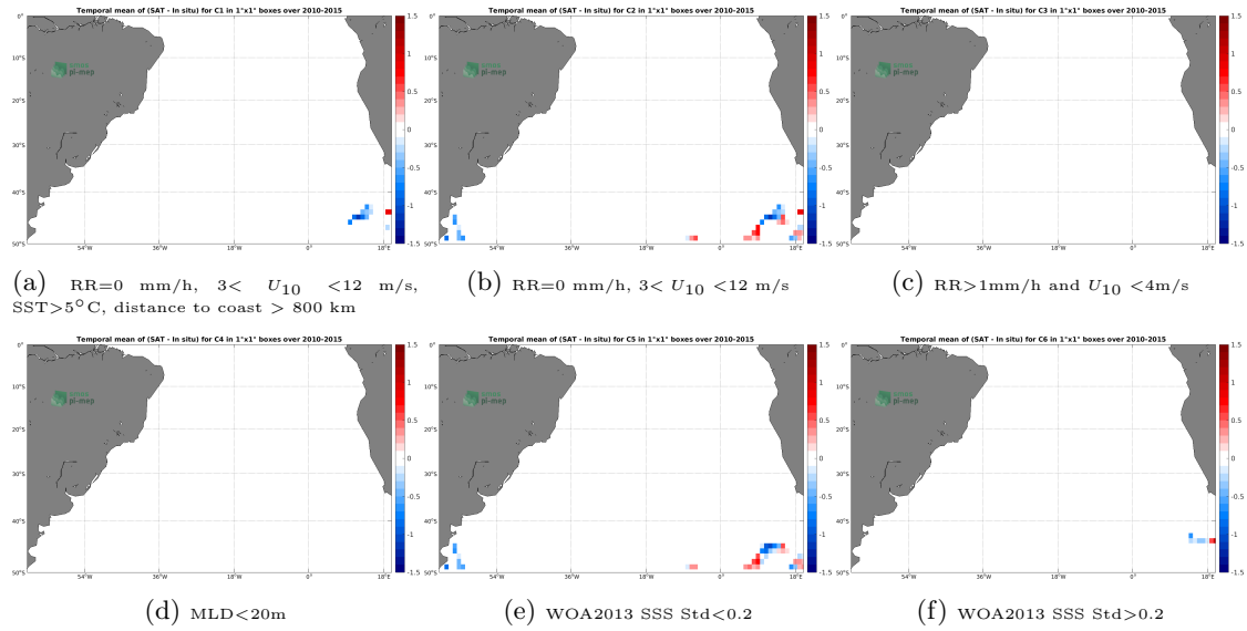
Figure 12: Temporal mean gridded over spatial boxes of size 1^{\circ}\times 1^{\circ} of \Delta\text{SSS} (SMOS L4 v2 Weekly (CATDS-CECOS-IFREMER) - Sea mammals) for 6 different subdatasets corresponding to:RR=0 mm/h, 3 < U_{10} < 12 m/s, SST >5^{\circ}\text{C} , distance to coast > 800 km (a), RR=0 mm/h, 3 < U_{10} < 12 m/s (b), RR >1\text{mm/h} and U_{10} < 4\text{m/s} (c),MLD <20\text{m} (d),WOA2013 SSS Std <0.2 (e),WOA2013 SSS Std >0.2 (f).
