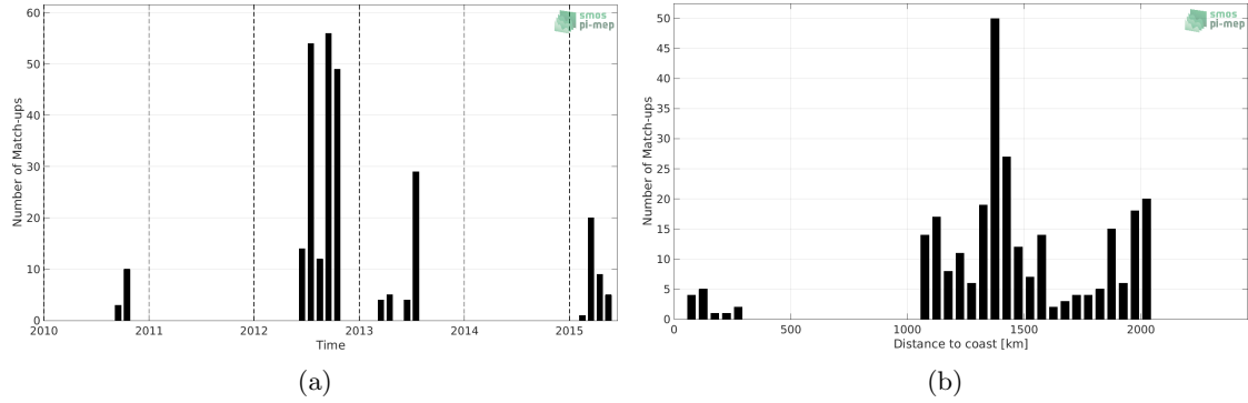
Figure 1: Number of match-ups between Sea mammals and SMOS L4 v2 Weekly (CATDS-CECOS-IFREMER) SSS as a function of time (a) and as function of the distance to coast (b) over the South Atlantic Ocean Pi-MEP region and for the full satellite product period.
