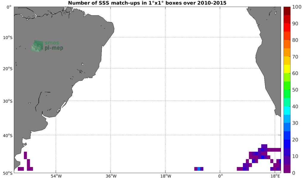
Figure 4: Number of SSS match-ups between Sea mammals SSS and the SMOS L4 v2 Weekly (CATDS-CECOS-IFREMER) SSS product for the South Atlantic Ocean Pi-MEP region over 1^\circ \times 1^\circ boxes and for the full satellite product period.
