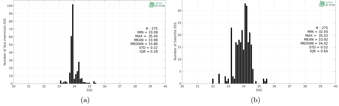
Figure 2: Histograms of SSS from Sea mammals (a) and SMOS L4 v2 Weekly (CATDS-CECOS-IFREMER) (b) considering all match-up pairs per bins of 0.1 over the South Atlantic Ocean Pi-MEP region and for the full satellite product period.
