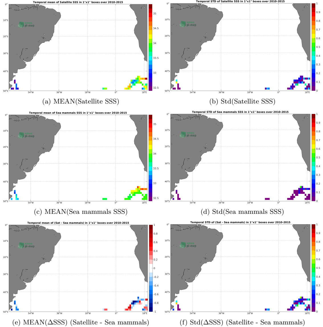
Figure 6: Temporal mean (left) and Std (right) of SSS from SMOS L4 v2 Weekly (CATDS-CECOS-IFREMER) (top), Sea mammals (middle), and of \Delta SSS (Satellite - Sea mammals). Only match-up pairs are used to generate these maps.
