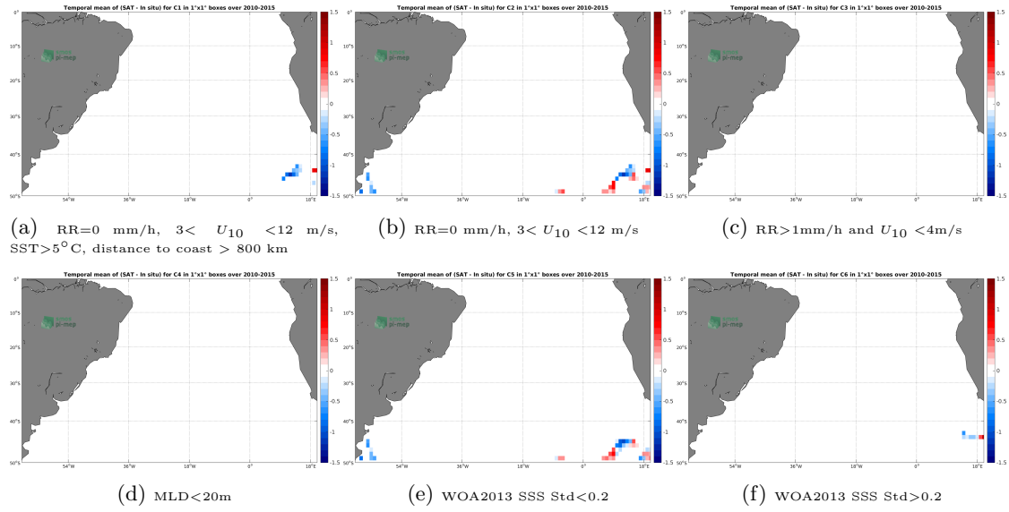
Figure 12: Temporal mean gridded over spatial boxes of size 1^\circ \times 1^\circ of \Delta SSS (SMOS-L4-CATDS-CECOS-IFREMER-V2-WEEKLY-0.5DEG - Sea mammals) for 6 different subdatasets corresponding to: RR=0 mm/h, 3 < U_{10} < 12 m/s, SST > 5^\circ C , distance to coast > 800 km (a), RR=0 mm/h, 3 < U_{10} < 12 m/s (b), RR > 1 mm/h and U_{10} < 4 m/s (c), MLD < 20 m (d), WOA2013 SSS Std < 0.2 (e), WOA2013 SSS Std > 0.2 (f).
