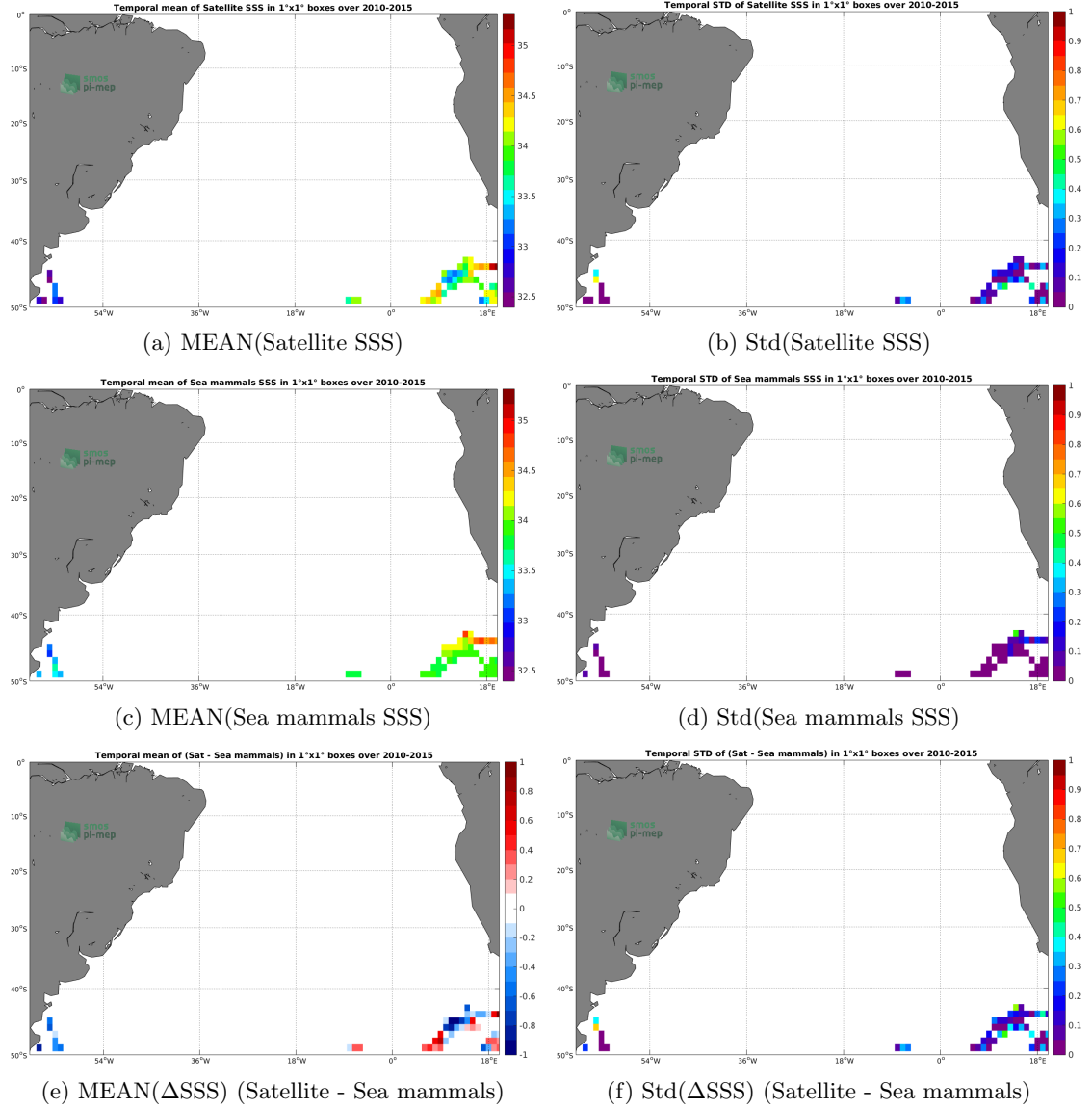
Figure 6: Temporal mean (left) and Std (right) of SSS from SMOS-L4-CATDS-CECOS-IFREMER-V2-WEEKLY-0.5DEG (top), Sea mammals (middle), and of \Delta SSS (Satellite - Sea mammals). Only match-up pairs are used to generate these maps.
