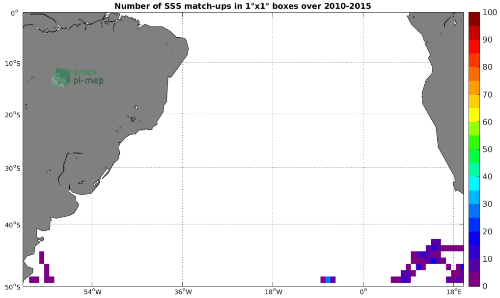
Figure 4: Number of SSS match-ups between Sea mammals SSS and the SMOS-L4-CATDS-CECOS-IFREMER-V2-WEEKLY-0.5DEG SSS product for the South Atlantic Ocean Pi-MEP region over 1^\circ \times 1^\circ boxes and for the full satellite product period.
