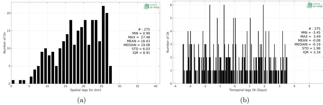
Figure 5: Histograms of the spatial (a) and temporal (b) lags between the time of the Sea mammals measurements and the date of the corresponding SMOS-L4-CATDS-CECOS-IFREMER-V2-WEEKLY-0.5DEG SSS product.
