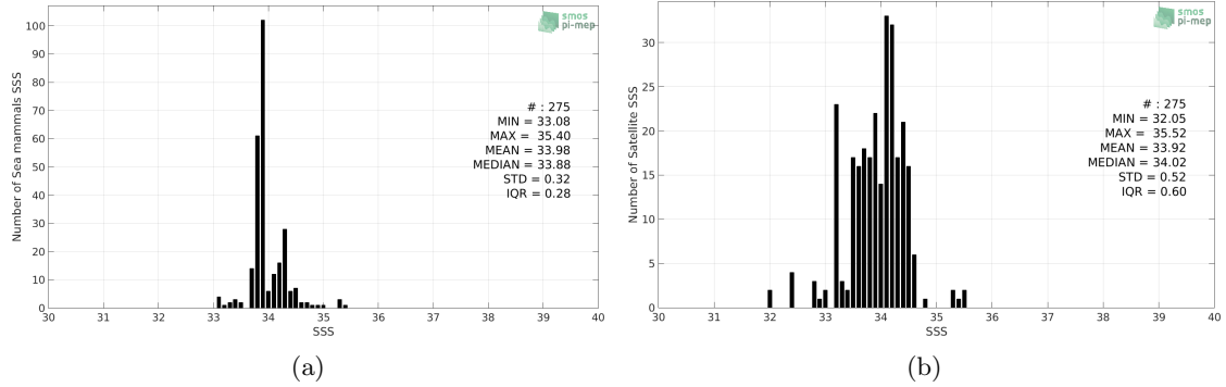
Figure 2: Histograms of SSS from Sea mammals (a) and SMOS-L4-CATDS-CECOS-IFREMER-V2-WEEKLY-0.5DEG (b) considering all match-up pairs per bins of 0.1 over the South Atlantic Ocean Pi-MEP region and for the full satellite product period.
