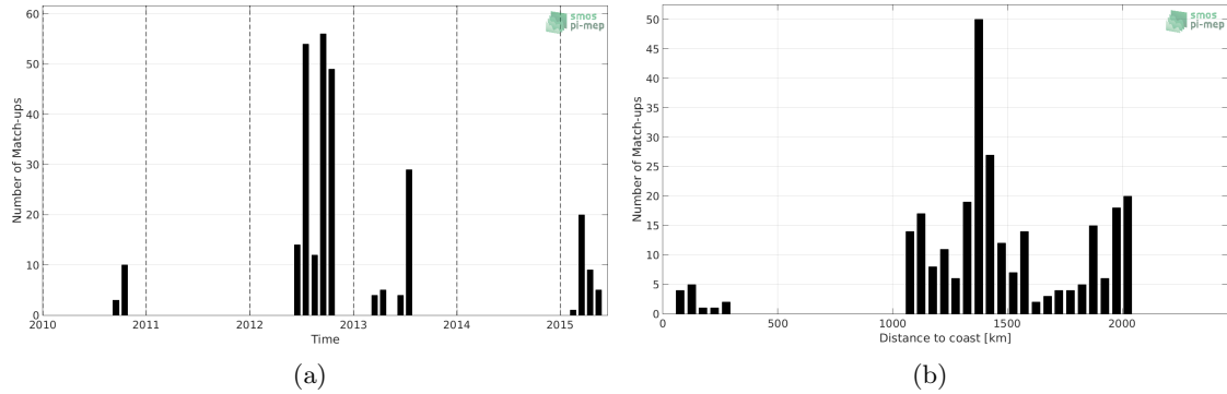
Figure 1: Number of match-ups between Sea mammals and SMOS-L4-CATDS-CECOS-IFREMER-V2-WEEKLY-0.5DEG SSS as a function of time (a) and as function of the distance to coast (b) over the South Atlantic Ocean Pi-MEP region and for the full satellite product period.
