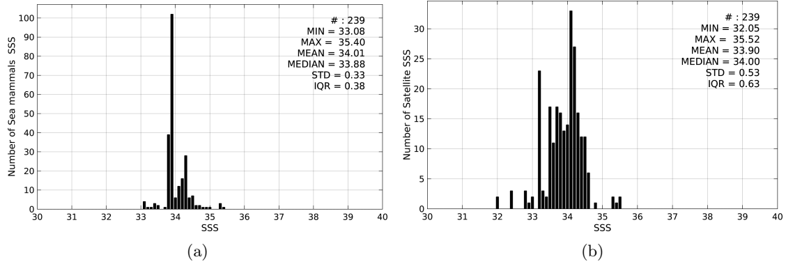
Figure 2: Histograms of SSS from Sea mammals (a) and SMOS-L4-CATDS-CECOS-IFREMER-V2-WEEKLY-0.5DEG (b) considering all match-up pairs per bins of 0.1 over the South Atlantic Ocean Pi-MEP region and for the full satellite product period.
