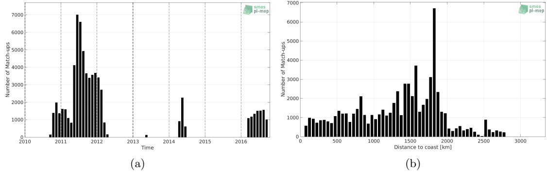
Figure 1: Number of match-ups between Surface drifters and SMOS L4 v2 Weekly (CATDS-CECOS-IFREMER) SSS as a function of time (a) and as function of the distance to coast (b) over the South Atlantic Ocean Pi-MEP region and for the full satellite product period.
