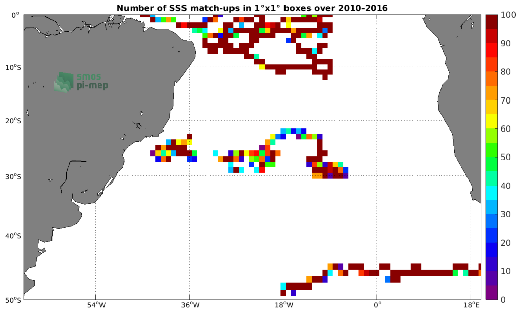
Figure 3: Number of SSS match-ups between Surface drifters SSS and the SMOS L4 v2 Weekly (CATDS-CECOS-IFREMER) SSS product for the South Atlantic Ocean Pi-MEP region over 1°x1° boxes and for the full satellite product period.
