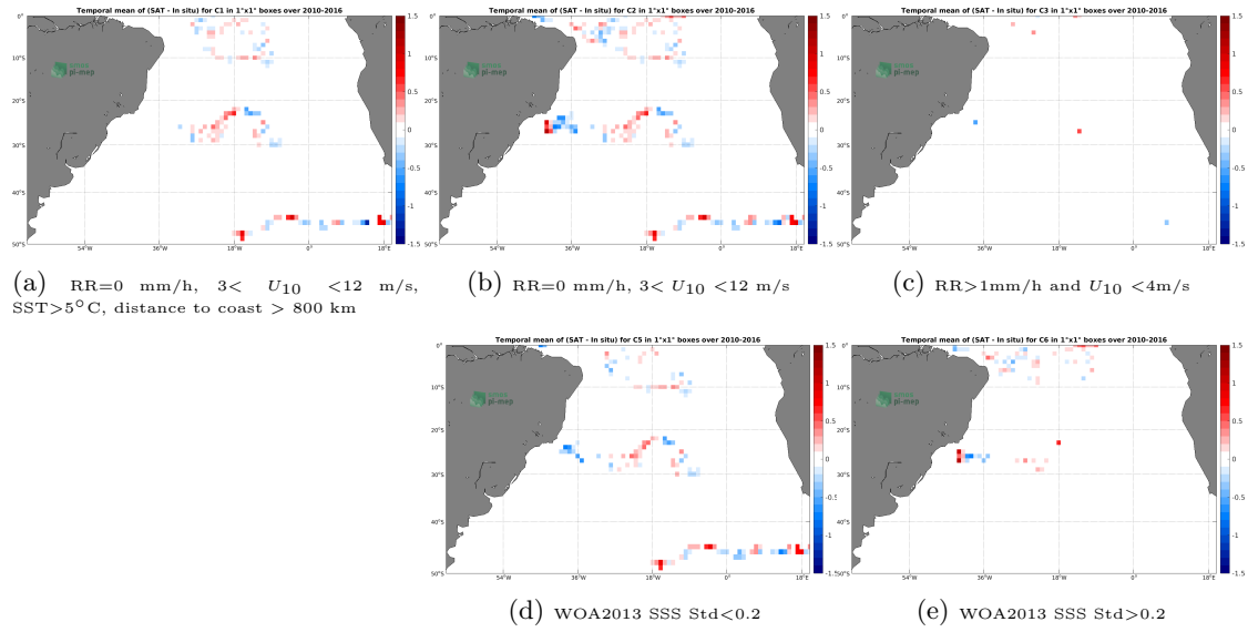
Figure 11: Temporal mean gridded over spatial boxes of size 1^\circ \times 1^\circ of \Delta SSS (SMOS L4 v2 Weekly (CATDS-CECOS-IFREMER) - Surface drifters) for 5 different subdatasets corresponding to: RR=0 mm/h, 3 < U_{10} < 12 m/s, SST > 5^\circ C , distance to coast > 800 km (a), RR=0 mm/h, 3 < U_{10} < 12 m/s (b), RR > 1 mm/h and U_{10} < 4 m/s (c), WOA2013 SSS Std < 0.2 (d), WOA2013 SSS Std > 0.2 (e).
