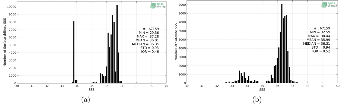
Figure 2: Histograms of SSS from Surface drifters (a) and SMOS L4 v2 Weekly (CATDS-CECOS-IFREMER) (b) considering all match-up pairs per bins of 0.1 over the South Atlantic Ocean Pi-MEP region and for the full satellite product period.
