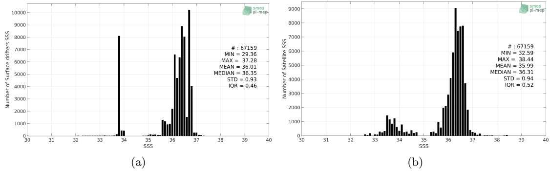
Figure 2: Histograms of SSS from Surface drifters (a) and SMOS-L4-CATDS-CECOS-IFREMER-V2-WEEKLY-0.5DEG (b) considering all match-up pairs per bins of 0.1 over the South Atlantic Ocean Pi-MEP region and for the full satellite product period.
