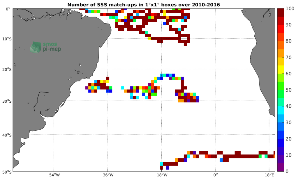
Figure 3: Number of SSS match-ups between Surface drifters SSS and the SMOS-L4-CATDS-CECOS-IFREMER-V2-WEEKLY-0.5DEG SSS product for the South Atlantic Ocean Pi-MEP region over 1°x1° boxes and for the full satellite product period.
