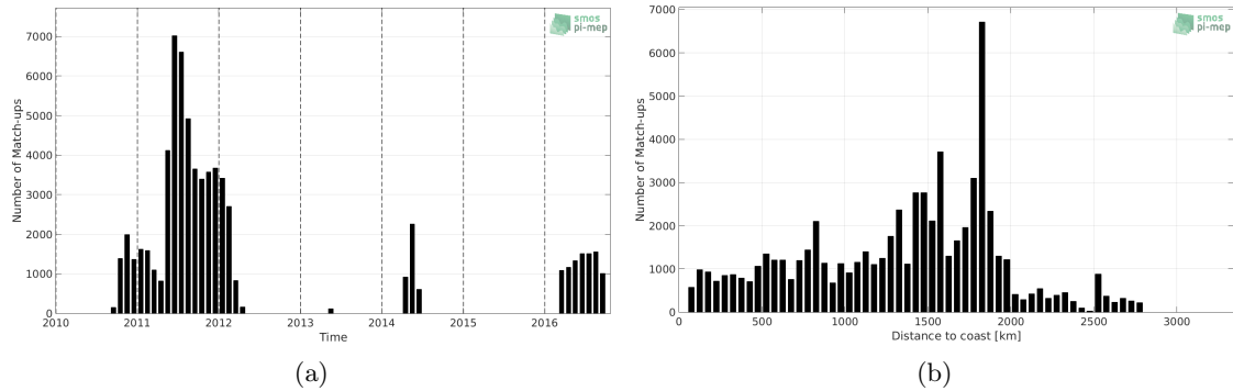
Figure 1: Number of match-ups between Surface drifters and SMOS-L4-CATDS-CECOS-IFREMER-V2-WEEKLY-0.5DEG SSS as a function of time (a) and as function of the distance to coast (b) over the South Atlantic Ocean Pi-MEP region and for the full satellite product period.
