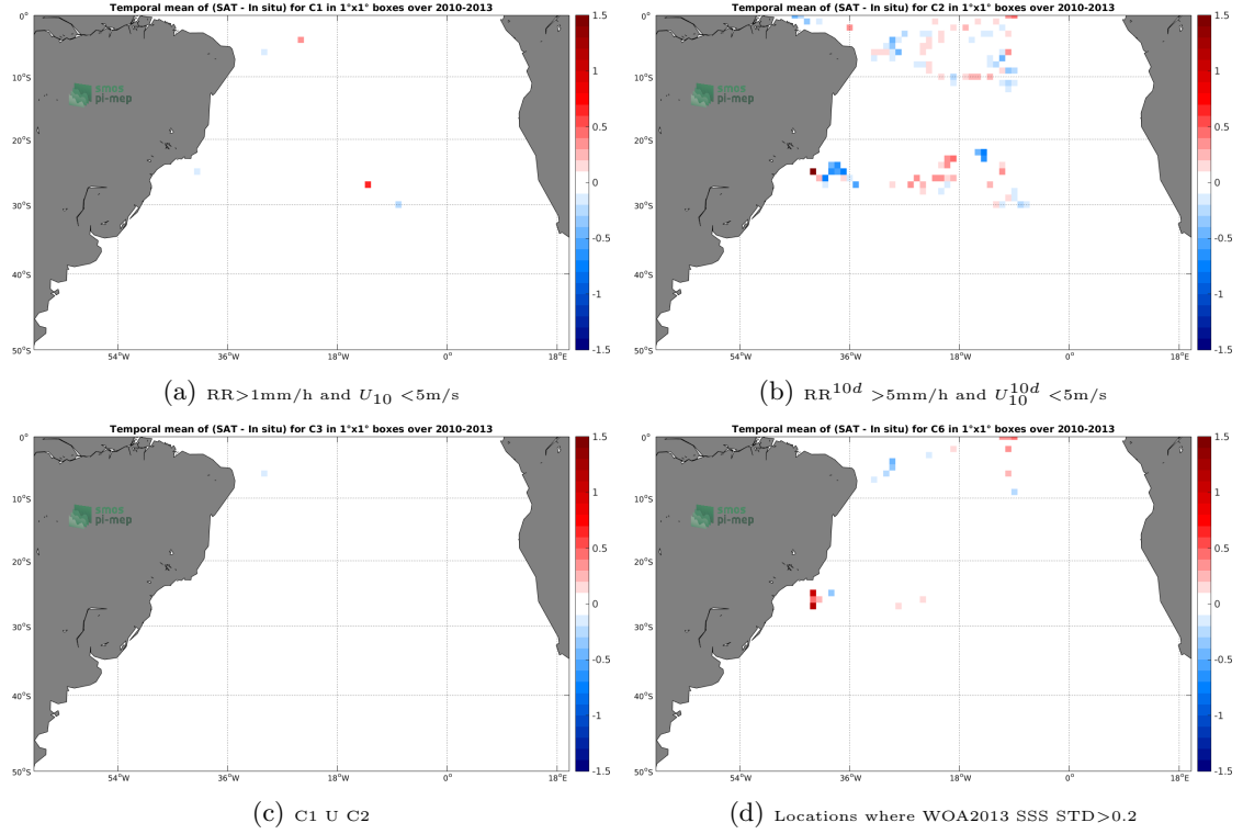
Figure 11: Temporal mean gridded over spatial boxes of size 1^\circ \times 1^\circ of \Delta SSS (SMOS-L4-CATDS-CECOS-IFREMER-V2-WEEKLY-0.5DEG - Surface drifters) for 4 different subdatasets corresponding to: RR > 1mm/h and U_{10} < 5\text{m/s} (a), RR^{10d} > 5\text{mm/h} and U_{10}^{10d} < 5\text{m/s} (b), C1 U C2 (c), Locations where WOA2013 SSS STD > 0.2 (d).
