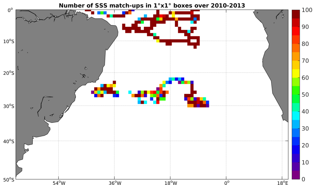
Figure 3: Number of SSS match-ups between Surface drifters SSS and the SMOS-L4-CATDS-CECOS-IFREMER-V2-WEEKLY-0.5DEG SSS product for the South Atlantic Ocean Pi-MEP region over 1°x1° boxes and for the full satellite product period.
