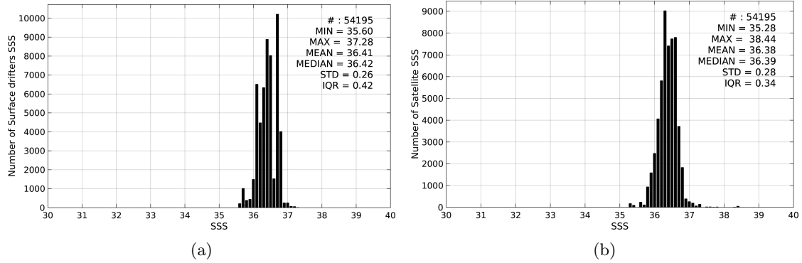
Figure 2: Histograms of SSS from Surface drifters (a) and SMOS-L4-CATDS-CECOS-IFREMER-V2-WEEKLY-0.5DEG (b) considering all match-up pairs per bins of 0.1 over the South Atlantic Ocean Pi-MEP region and for the full satellite product period.
