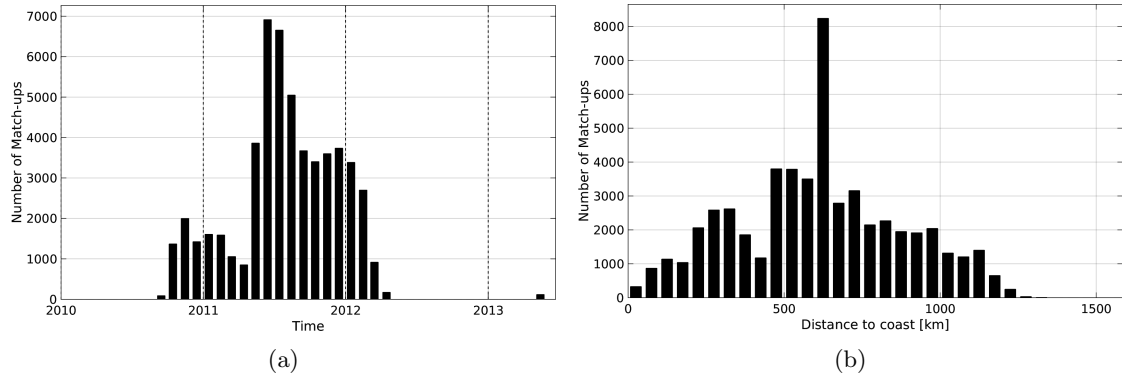
Figure 1: Number of match-ups between Surface drifters and SMOS-L4-CATDS-CECOS-IFREMER-V2-WEEKLY-0.5DEG SSS as a function of time (a) and as function of the distance to coast (b) over the South Atlantic Ocean Pi-MEP region and for the full satellite product period.
