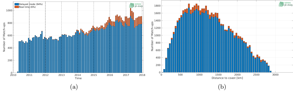
Figure 1: Number of match-ups between Argo and SMOS L4 v2 Weekly (CATDS-CECOS-IFREMER) SSS as a function of time (a) and as function of the distance to coast (b) over the South Atlantic Ocean Pi-MEP region and for the full satellite product period.
