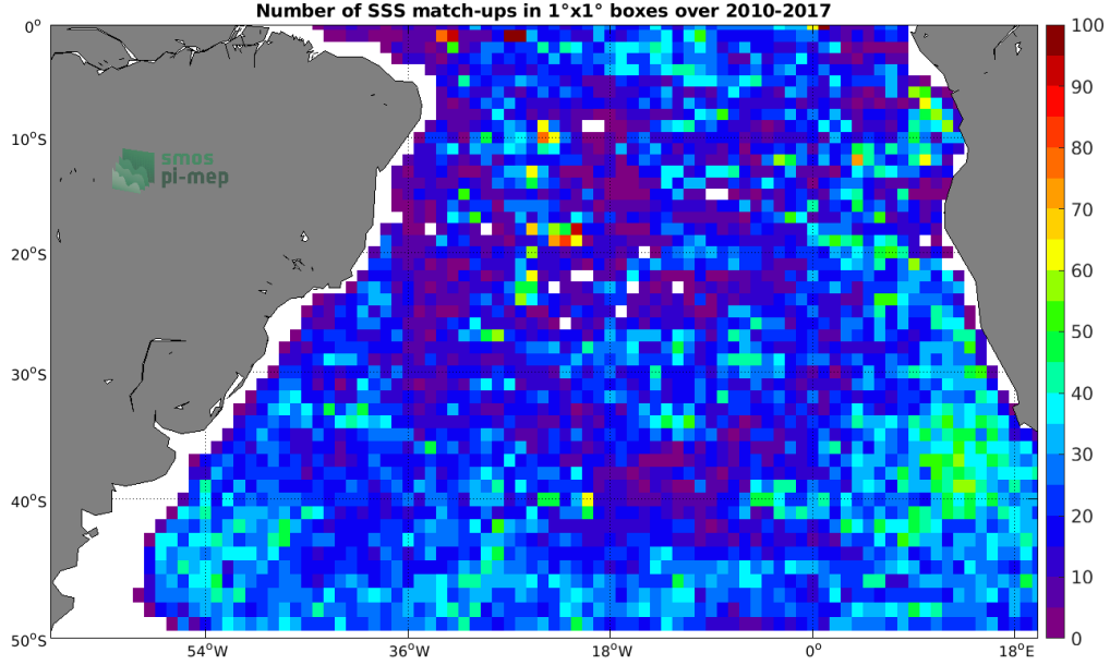
Figure 4: Number of SSS match-ups between Argo SSS and the SMOS L4 v2 Weekly (CATDS-CECOS-IFREMER) SSS product for the South Atlantic Ocean Pi-MEP region over 1^\circ \times 1^\circ boxes and for the full satellite product period.
