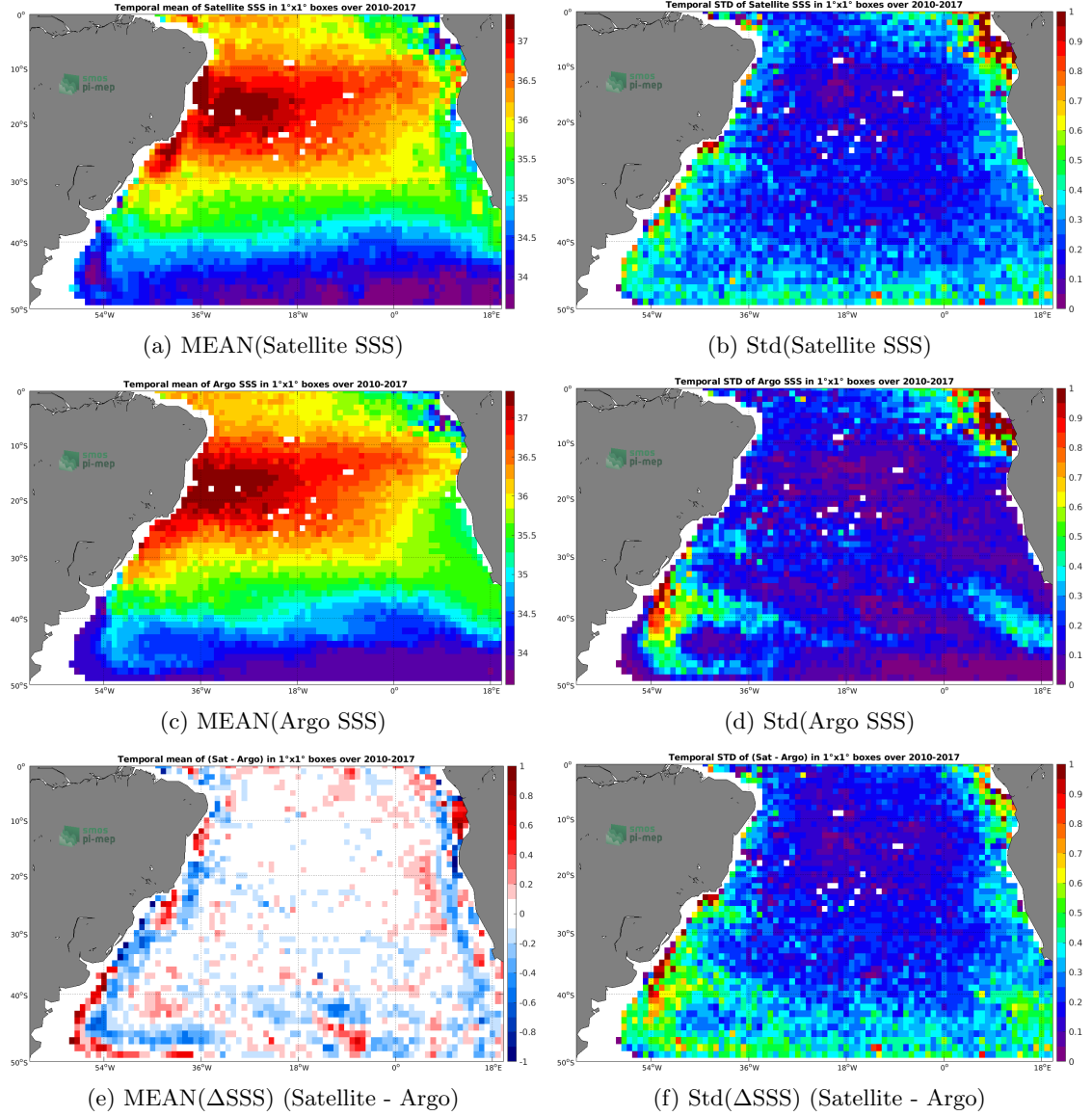
Figure 6: Temporal mean (left) and Std (right) of SSS from SMOS L4 v2 Weekly (CATDS-CECOS-IFREMER) (top), Argo (middle), and of \Delta SSS (Satellite - Argo). Only match-up pairs are used to generate these maps.
