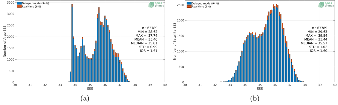
Figure 2: Histograms of SSS from Argo (a) and SMOS L4 v2 Weekly (CATDS-CECOS-IFREMER) (b) considering all match-up pairs per bins of 0.1 over the South Atlantic Ocean Pi-MEP region and for the full satellite product period.
