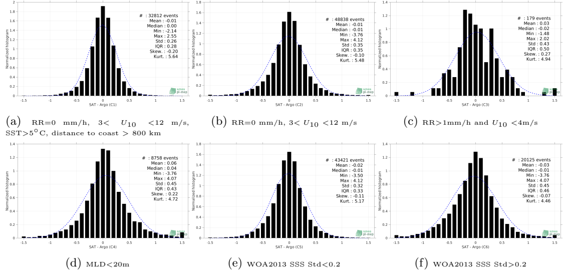
Figure 13: Normalized histogram of \Delta SSS (SMOS L4 v2 Weekly (CATDS-CECOS-IFREMER) - Argo) for 6 different subdatasets corresponding to: RR=0 mm/h, 3 < U_{10} < 12 m/s, SST>5°C, distance to coast > 800 km (a), RR=0 mm/h, 3 < U_{10} < 12 m/s (b), RR>1mm/h and U_{10} < 4 m/s (c), MLD<20m (d), WOA2013 SSS Std<0.2 (e), WOA2013 SSS Std>0.2 (f).
