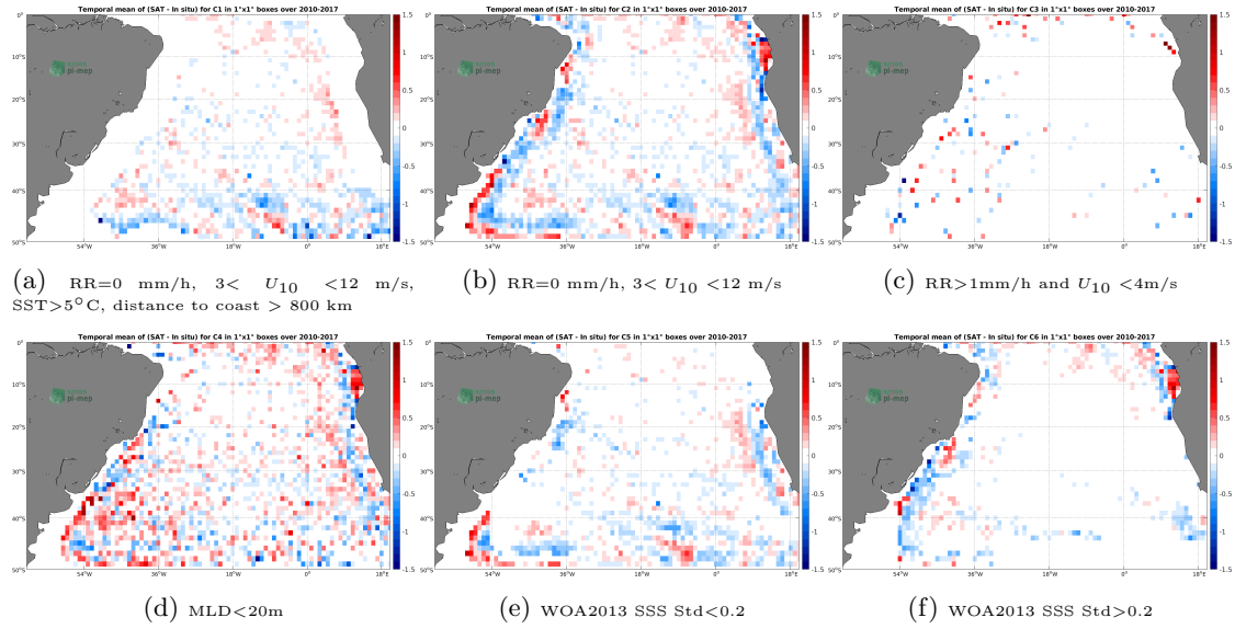
Figure 12: Temporal mean gridded over spatial boxes of size 1^\circ \times 1^\circ of \Delta SSS (SMOS L4 v2 Weekly (CATDS-CECOS-IFREMER) - Argo) for 6 different subdatasets corresponding to: RR=0 mm/h, 3 < U_{10} < 12 m/s, SST > 5^\circ C , distance to coast > 800 km (a), RR=0 mm/h, 3 < U_{10} < 12 m/s (b), RR > 1 mm/h and U_{10} < 4 m/s (c), MLD < 20 m (d), WOA2013 SSS Std < 0.2 (e), WOA2013 SSS Std > 0.2 (f).
