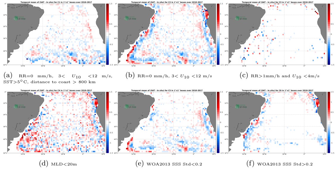
Figure 12: Temporal mean gridded over spatial boxes of size 1^\circ \times 1^\circ of \Delta SSS (SMOS L4 v2 Weekly (CATDS-CECOS-IFREMER) - Argo) for 6 different subdatasets corresponding to: RR=0 mm/h, 3 < U_{10} < 12 m/s, SST > 5^\circ C , distance to coast > 800 km (a), RR=0 mm/h, 3 < U_{10} < 12 m/s (b), RR > 1 mm/h and U_{10} < 4 m/s (c), MLD < 20 m (d), WOA2013 SSS Std < 0.2 (e), WOA2013 SSS Std > 0.2 (f).
