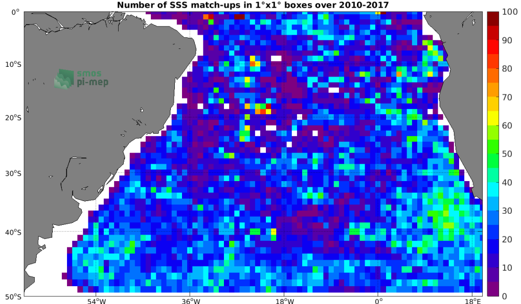
Figure 4: Number of SSS match-ups between Argo SSS and the SMOS L4 v2 Weekly (CATDS-CECOS-IFREMER) SSS product for the South Atlantic Ocean Pi-MEP region over 1^\circ \times 1^\circ boxes and for the full satellite product period.
