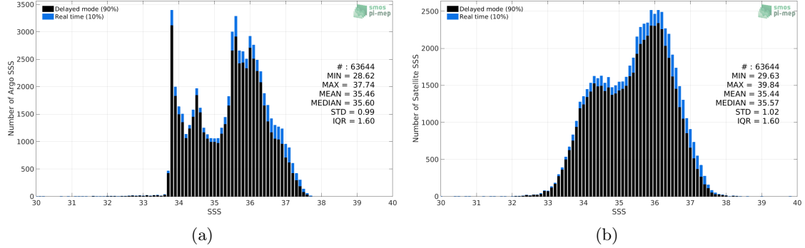
Figure 2: Histograms of SSS from Argo (a) and SMOS L4 v2 Weekly (CATDS-CECOS-IFREMER) (b) considering all match-up pairs per bins of 0.1 over the South Atlantic Ocean Pi-MEP region and for the full satellite product period.
