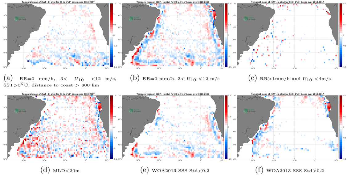
Figure 12: Temporal mean gridded over spatial boxes of size 1^\circ \times 1^\circ of \Delta SSS (SMOS-L4-CATDS-CECOS-IFREMER-V2-WEEKLY-0.5DEG - Argo) for 6 different subdatasets corresponding to: RR=0 mm/h, 3 < U_{10} < 12 m/s, SST > 5^\circ\text{C} , distance to coast > 800 km (a), RR=0 mm/h, 3 < U_{10} < 12 m/s (b), RR > 1 mm/h and U_{10} < 4 m/s (c), MLD < 20 m (d), WOA2013 SSS Std < 0.2 (e), WOA2013 SSS Std > 0.2 (f).
