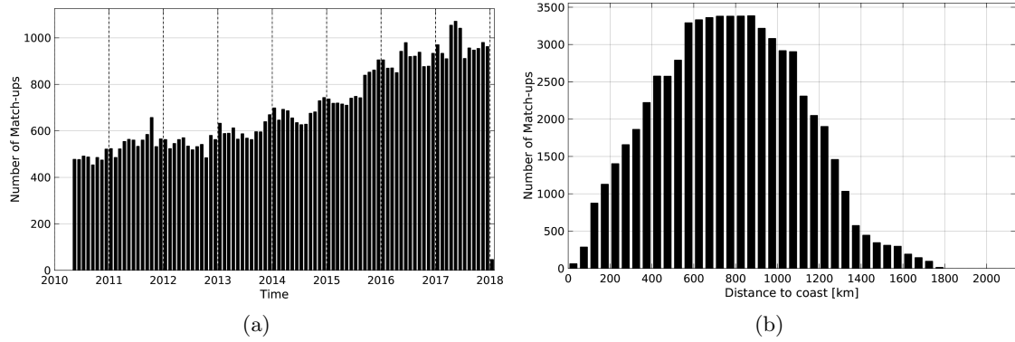
Figure 1: Number of match-ups between Argo and SMOS-L4-CATDS-CECOS-IFREMER-V2-WEEKLY-0.5DEG SSS as a function of time (a) and as function of the distance to coast (b) over the South Atlantic Ocean Pi-MEP region and for the full satellite product period.
