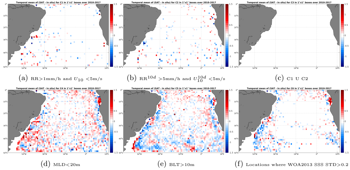
Figure 12: Temporal mean gridded over spatial boxes of size 1^\circ \times 1^\circ of \Delta SSS (SMOS-L4-CATDS-CECOS-IFREMER-V2-WEEKLY-0.5DEG - Argo) for 6 different subdatasets corresponding to:RR>1mm/h and U_{10} < 5 m/s (a), RR^{10d} > 5 mm/h and U_{10}^{10d} < 5 m/s (b), C1 U C2 (c),MLD<20m (d),BLT>10m (e),Locations where WOA2013 SSS STD>0.2 (f).
