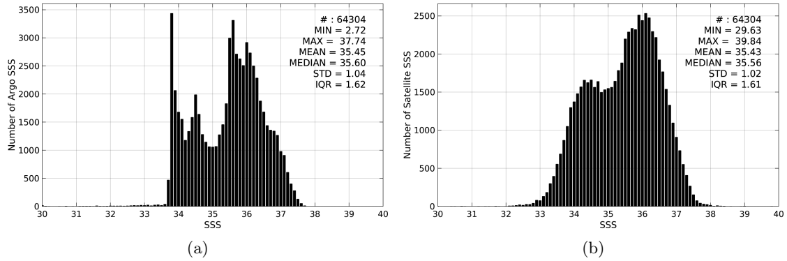
Figure 2: Histograms of SSS from Argo (a) and SMOS-L4-CATDS-CECOS-IFREMER-V2-WEEKLY-0.5DEG (b) considering all match-up pairs per bins of 0.1 over the South Atlantic Ocean Pi-MEP region and for the full satellite product period.
