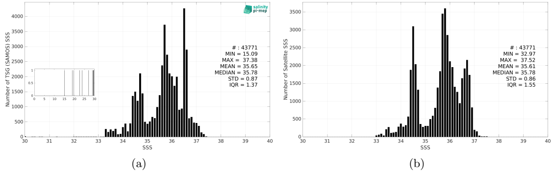
Figure 3: Histograms of SSS from TSG (SAMOS) (a) and SMOS SSS L4 v2 - Daily (BEC) (b) considering all match-up pairs per bins of 0.1 over the South Atlantic Ocean Pi-MEP region and for the full satellite product period.
