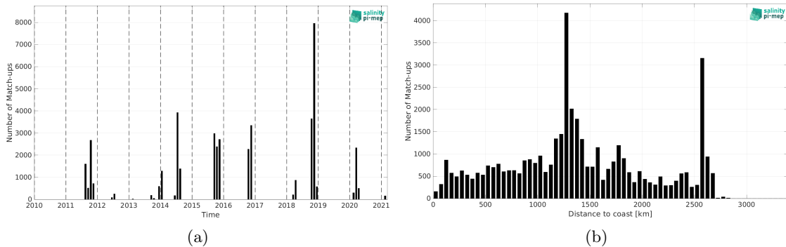
Figure 2: Number of match-ups between TSG (SAMOS) and SMOS SSS L4 v2 - Daily (BEC) SSS as a function of time (a) and as function of the distance to coast (b) over the South Atlantic Ocean Pi-MEP region and for the full satellite product period.
