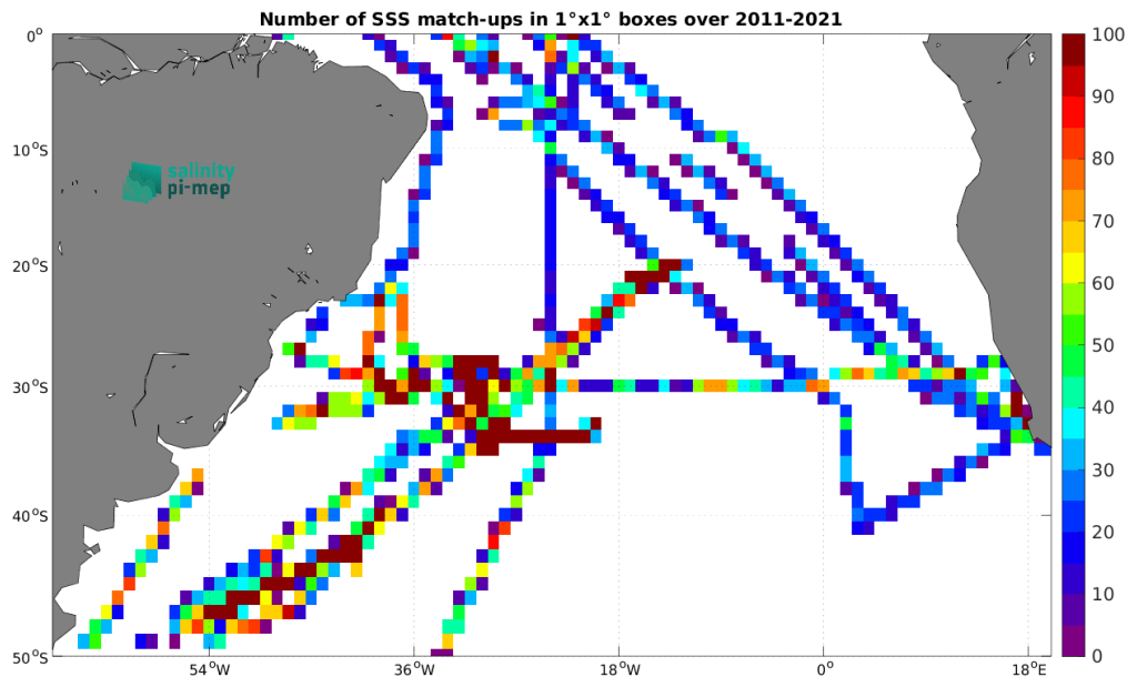
Figure 5: Number of SSS match-ups between TSG (SAMOS) SSS and the SMOS SSS L4 v2 - Daily (BEC) SSS product for the South Atlantic Ocean Pi-MEP region over 1^\circ \times 1^\circ boxes and for the full satellite product period.
