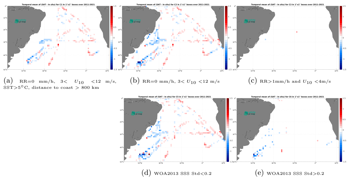
Figure 14: Temporal mean gridded over spatial boxes of size 1^\circ \times 1^\circ of \Delta\text{SSS} (SMOS SSS L4 v2 - Daily (BEC) - TSG (SAMOS)) for 5 different subdatasets corresponding to:RR=0 mm/h, 3 < U_{10} < 12 m/s, SST >5^\circ\text{C} , distance to coast > 800 km (a), RR=0 mm/h, 3 < U_{10} < 12 m/s (b), RR >1 mm/h and U_{10} < 4 m/s (c), WOA2013 SSS Std <0.2 (d), WOA2013 SSS Std >0.2 (e).
