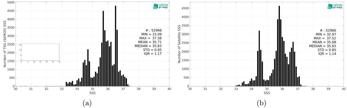
Figure 2: Histograms of SSS from TSG (SAMOS) (a) and SMOS SSS L4 v2 - Daily (BEC) (b) considering all match-up pairs per bins of 0.1 over the South Atlantic Ocean Pi-MEP region and for the full satellite product period.
