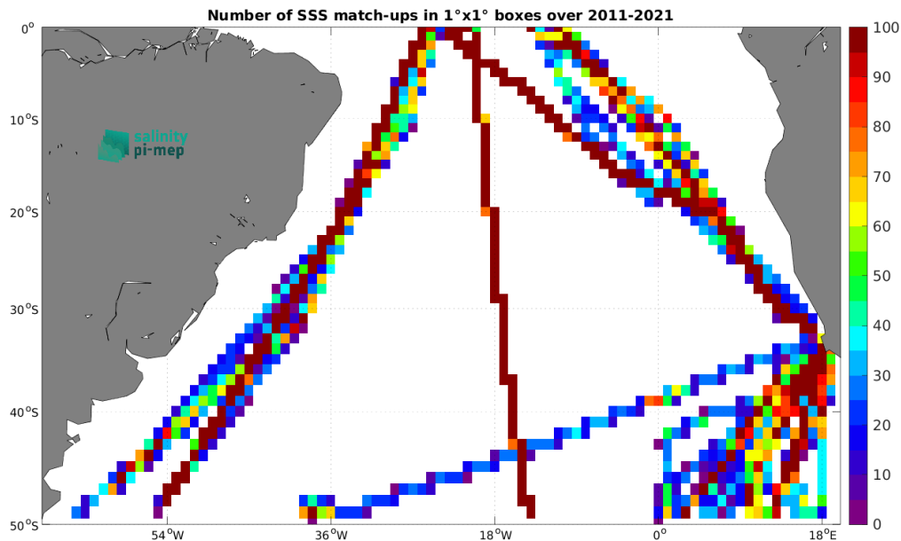
Figure 5: Number of SSS match-ups between TSG (Polarstern) SSS and the SMOS SSS L4 v2 - Daily (BEC) SSS product for the South Atlantic Ocean Pi-MEP region over 1^\circ \times 1^\circ boxes and for the full satellite product period.
