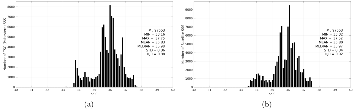
Figure 3: Histograms of SSS from TSG (Polarstern) (a) and SMOS SSS L4 v2 - Daily (BEC) (b) considering all match-up pairs per bins of 0.1 over the South Atlantic Ocean Pi-MEP region and for the full satellite product period.
