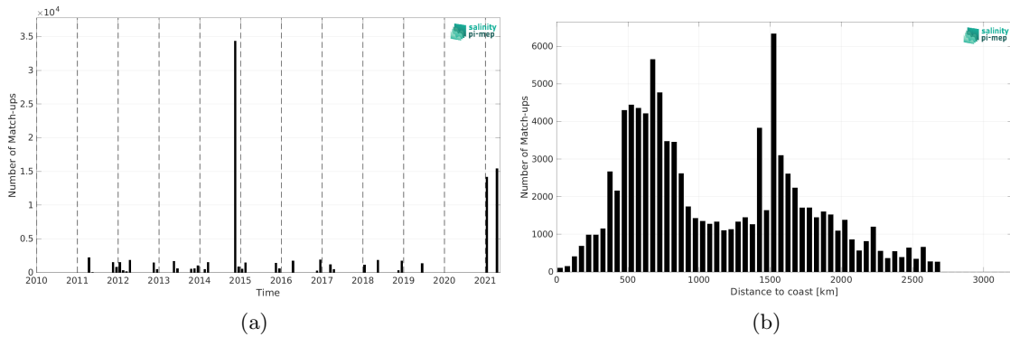
Figure 2: Number of match-ups between TSG (Polarstern) and SMOS SSS L4 v2 - Daily (BEC) SSS as a function of time (a) and as function of the distance to coast (b) over the South Atlantic Ocean Pi-MEP region and for the full satellite product period.
