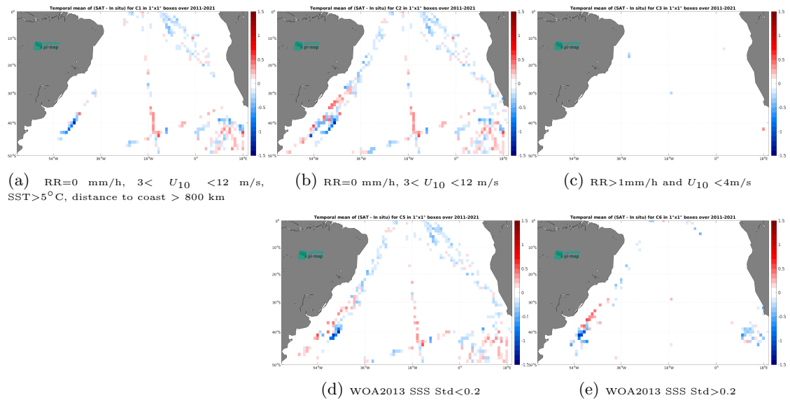
Figure 12: Temporal mean gridded over spatial boxes of size 1^\circ \times 1^\circ of \Delta SSS (SMOS SSS L4 v2 - Daily (BEC) - TSG (Polarstern)) for 5 different subdatasets corresponding to:RR=0 mm/h, 3 < U_{10} < 12 m/s, SST >5^\circ\text{C} , distance to coast > 800 km (a), RR=0 mm/h, 3 < U_{10} < 12 m/s (b), RR >1 mm/h and U_{10} < 4 m/s (c), WOA2013 SSS Std <0.2 (d), WOA2013 SSS Std >0.2 (e).
