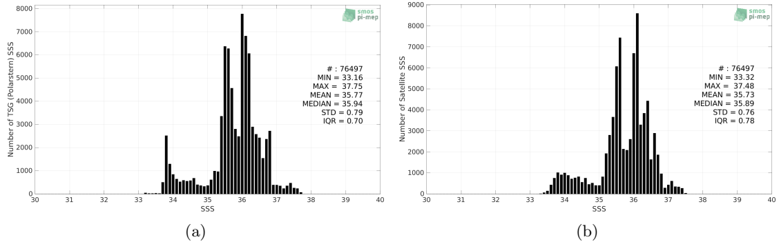
Figure 2: Histograms of SSS from TSG (Polarstern) (a) and SMOS SSS L4 v2 - Daily (BEC) (b) considering all match-up pairs per bins of 0.1 over the South Atlantic Ocean Pi-MEP region and for the full satellite product period.
