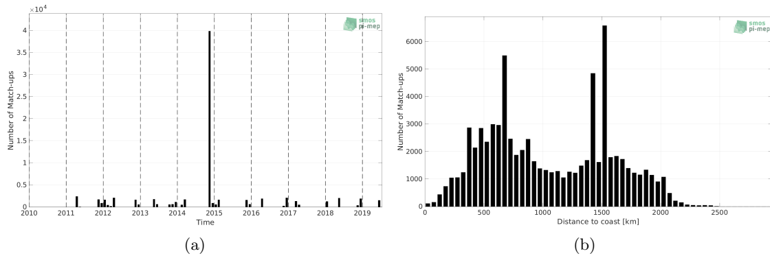
Figure 1: Number of match-ups between TSG (Polarstern) and SMOS SSS L4 v2 - Daily (BEC) SSS as a function of time (a) and as function of the distance to coast (b) over the South Atlantic Ocean Pi-MEP region and for the full satellite product period.
