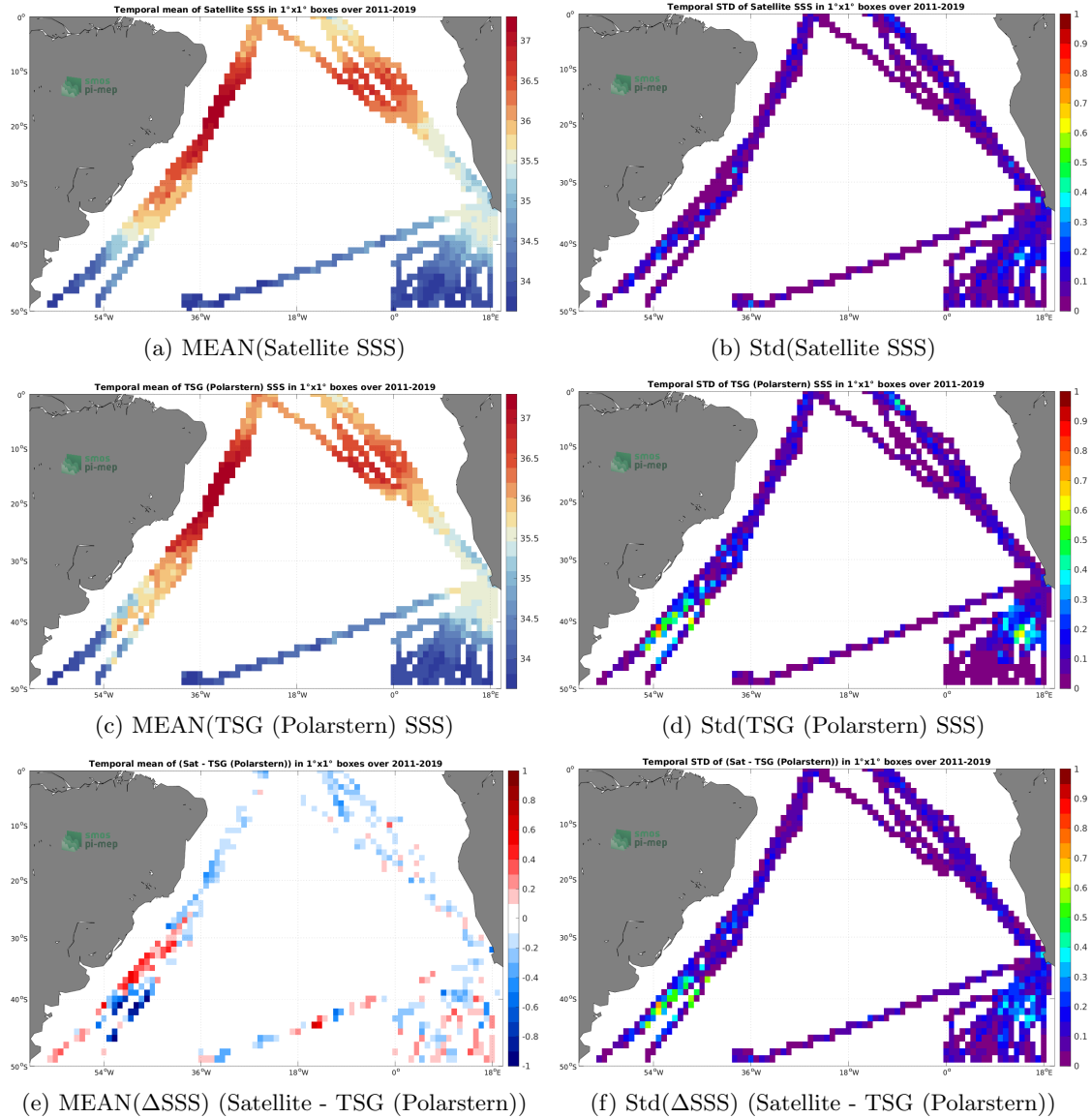
Figure 6: Temporal mean (left) and Std (right) of SSS from SMOS SSS L4 v2 - Daily (BEC) (top), TSG (Polarstern) (middle), and of \Delta SSS (Satellite - TSG (Polarstern)). Only match-up pairs are used to generate these maps.
