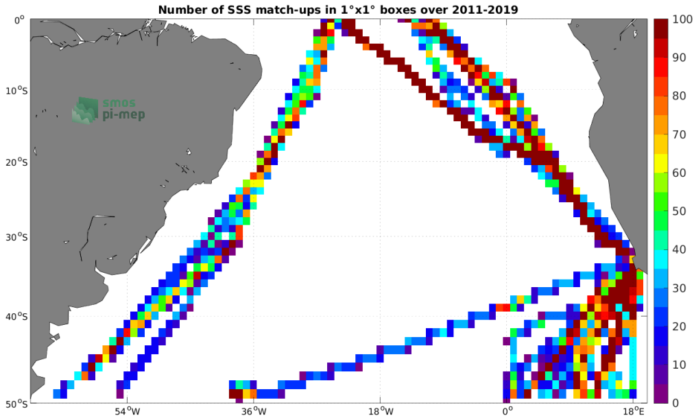
Figure 4: Number of SSS match-ups between TSG (Polarstern) SSS and the SMOS SSS L4 v2 - Daily (BEC) SSS product for the South Atlantic Ocean Pi-MEP region over 1^\circ \times 1^\circ boxes and for the full satellite product period.
