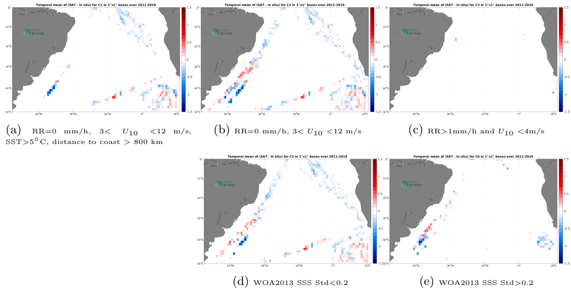
Figure 12: Temporal mean gridded over spatial boxes of size 1^\circ \times 1^\circ of \Delta\text{SSS} (SMOS SSS L4 v2 - Daily (BEC) - TSG (Polarstern)) for 5 different subdatasets corresponding to: \text{RR}=0 mm/h, 3 < U_{10} < 12 m/s, \text{SST} > 5^\circ\text{C} , distance to coast > 800 km (a), \text{RR}=0 mm/h, 3 < U_{10} < 12 m/s (b), \text{RR} > 1\text{mm/h} and U_{10} < 4\text{m/s} (c), WOA2013 SSS Std < 0.2 (d), WOA2013 SSS Std > 0.2 (e).
