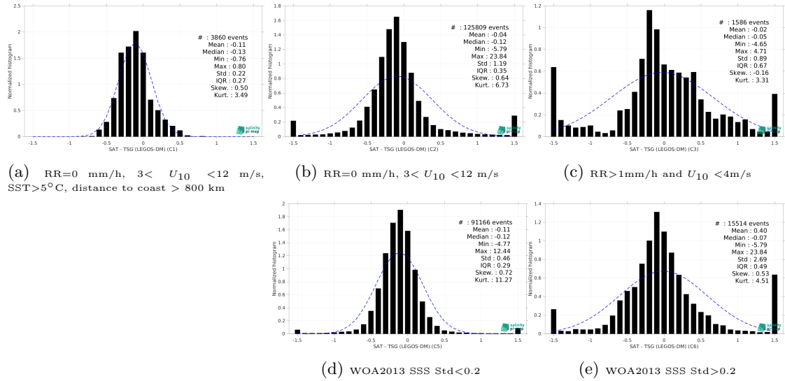
Figure 15: Normalized histogram of \Delta\text{SSS} (SMOS SSS L4 v2 - Daily (BEC) - TSG (LEGOS-DM)) for 5 different subdatasets corresponding to: RR=0 mm/h, 3 < U_{10} < 12 m/s, SST>5°C, distance to coast > 800 km (a), RR=0 mm/h, 3 < U_{10} < 12 m/s (b), RR>1mm/h and U_{10} < 4 m/s (c), WOA2013 SSS Std<0.2 (d), WOA2013 SSS Std>0.2 (e).
