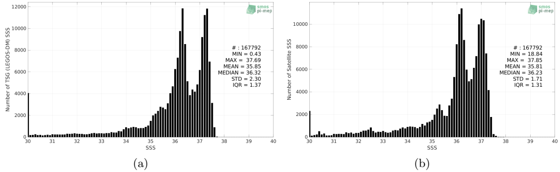
Figure 2: Histograms of SSS from TSG (LEGOS-DM) (a) and SMOS SSS L4 v2 - Daily (BEC) (b) considering all match-up pairs per bins of 0.1 over the South Atlantic Ocean Pi-MEP region and for the full satellite product period.
