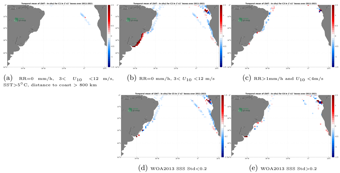
Figure 12: Temporal mean gridded over spatial boxes of size 1^\circ \times 1^\circ of \Delta SSS (SMOS SSS L4 v2 - Daily (BEC) - TSG (LEGOS-DM)) for 5 different subdatasets corresponding to:RR=0 mm/h, 3 < U_{10} < 12 m/s, SST >5^\circ\text{C} , distance to coast > 800 km (a), RR=0 mm/h, 3 < U_{10} < 12 m/s (b), RR >1 mm/h and U_{10} < 4 m/s (c), WOA2013 SSS Std <0.2 (d), WOA2013 SSS Std >0.2 (e).
