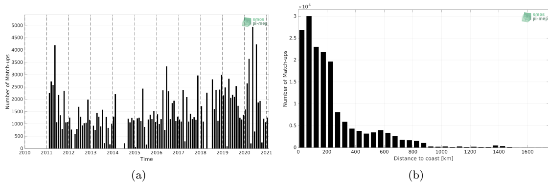
Figure 1: Number of match-ups between TSG (LEGOS-DM) and SMOS SSS L4 v2 - Daily (BEC) SSS as a function of time (a) and as function of the distance to coast (b) over the South Atlantic Ocean Pi-MEP region and for the full satellite product period.
