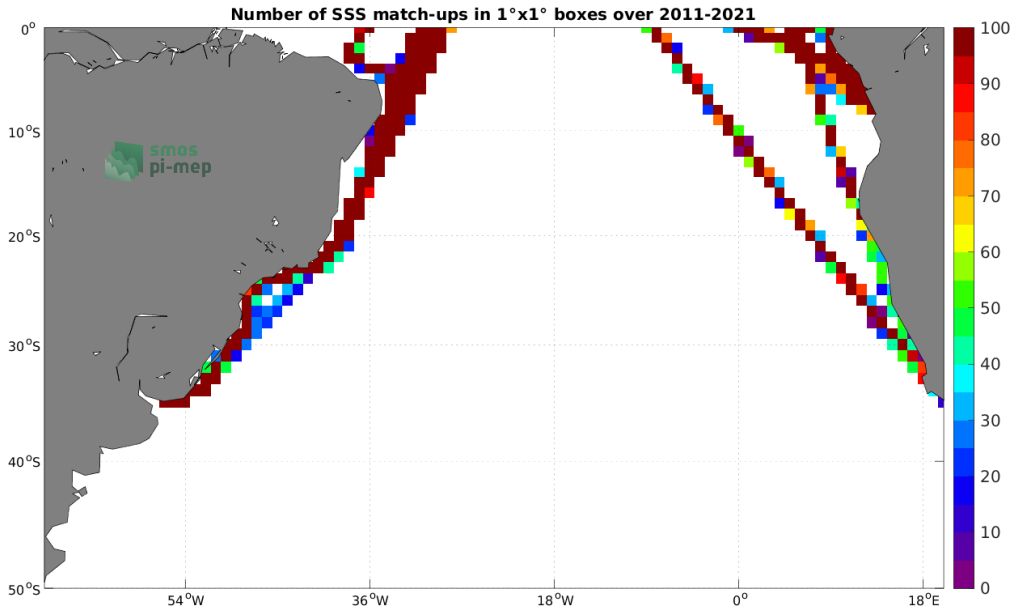
Figure 4: Number of SSS match-ups between TSG (LEGOS-DM) SSS and the SMOS SSS L4 v2 - Daily (BEC) SSS product for the South Atlantic Ocean Pi-MEP region over 1^\circ \times 1^\circ boxes and for the full satellite product period.
