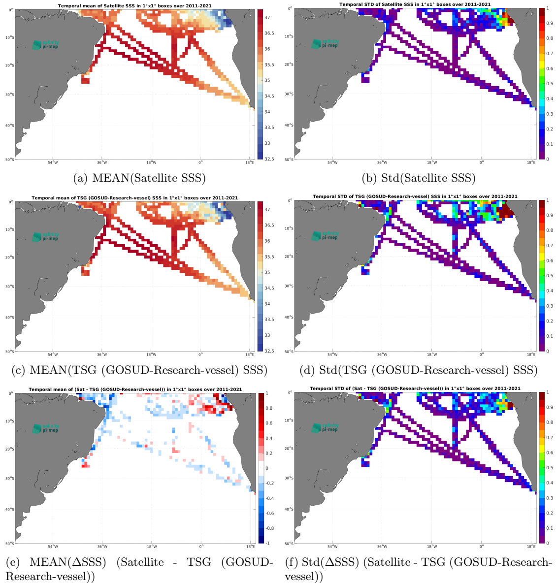
Figure 7: Temporal mean (left) and Std (right) of SSS from SMOS SSS L4 v2 - Daily (BEC) (top), TSG (GOSUD-Research-vessel) (middle), and of \Delta SSS (Satellite - TSG (GOSUD-Research-vessel)). Only match-up pairs are used to generate these maps.
