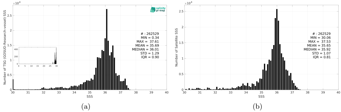
Figure 3: Histograms of SSS from TSG (GOSUD-Research-vessel) (a) and SMOS SSS L4 v2 - Daily (BEC) (b) considering all match-up pairs per bins of 0.1 over the South Atlantic Ocean Pi-MEP region and for the full satellite product period.
