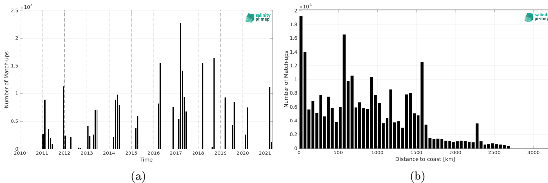
Figure 2: Number of match-ups between TSG (GOSUD-Research-vessel) and SMOS SSS L4 v2 - Daily (BEC) SSS as a function of time (a) and as function of the distance to coast (b) over the South Atlantic Ocean Pi-MEP region and for the full satellite product period.
