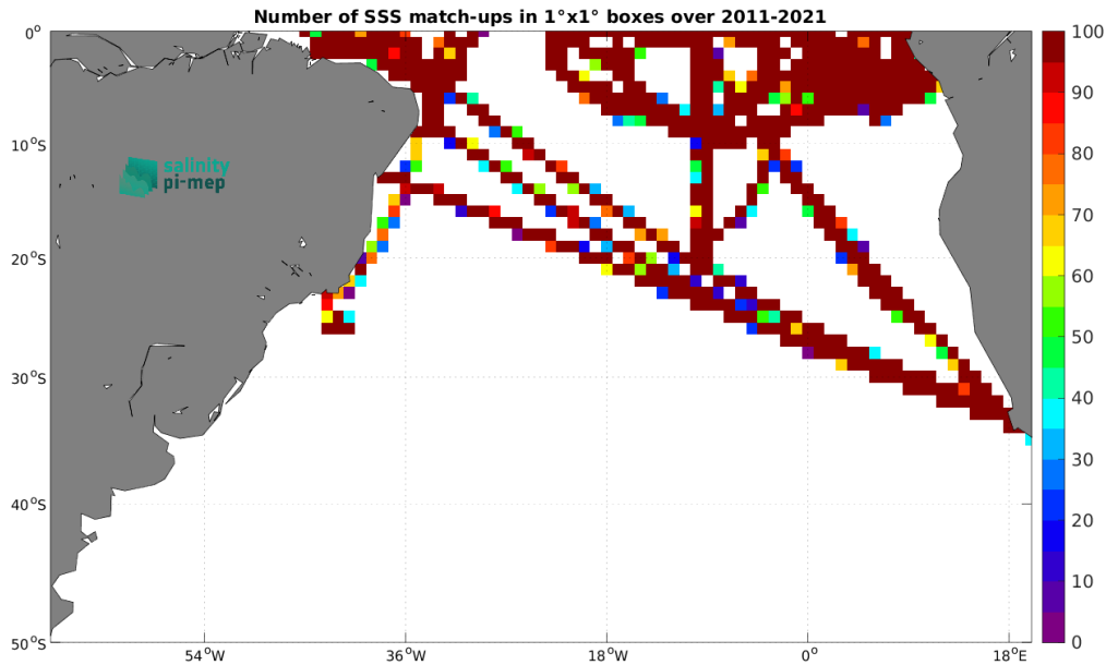
Figure 5: Number of SSS match-ups between TSG (GOSUD-Research-vessel) SSS and the SMOS SSS L4 v2 - Daily (BEC) SSS product for the South Atlantic Ocean Pi-MEP region over 1^\circ \times 1^\circ boxes and for the full satellite product period.
