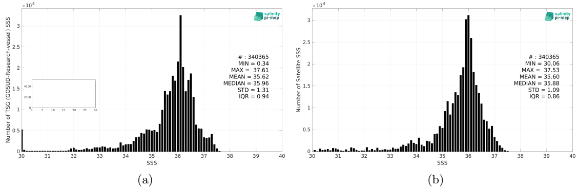
Figure 2: Histograms of SSS from TSG (GOSUD-Research-vessel) (a) and SMOS SSS L4 v2 - Daily (BEC) (b) considering all match-up pairs per bins of 0.1 over the South Atlantic Ocean Pi-MEP region and for the full satellite product period.
