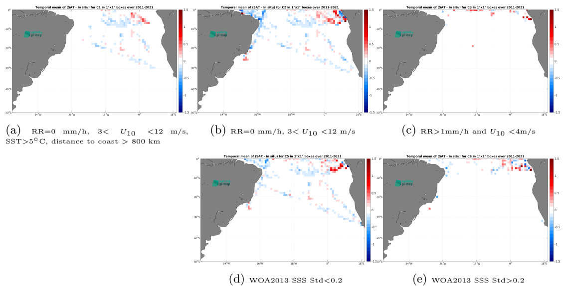
Figure 12: Temporal mean gridded over spatial boxes of size 1^\circ \times 1^\circ of \Delta SSS (SMOS SSS L4 v2 - Daily (BEC) - TSG (GOSUD-Research-vessel)) for 5 different subdatasets corresponding to:RR=0 mm/h, 3 < U_{10} < 12 m/s, SST>5°C, distance to coast > 800 km (a), RR=0 mm/h, 3 < U_{10} < 12 m/s (b), RR>1mm/h and U_{10} < 4 m/s (c), WOA2013 SSS Std<0.2 (d), WOA2013 SSS Std>0.2 (e).
