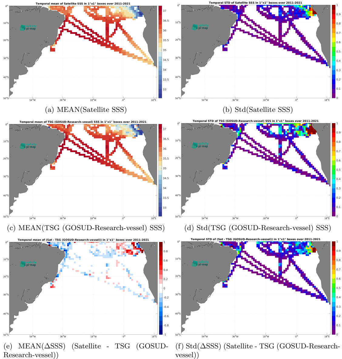
Figure 6: Temporal mean (left) and Std (right) of SSS from SMOS SSS L4 v2 - Daily (BEC) (top), TSG (GOSUD-Research-vessel) (middle), and of \Delta SSS (Satellite - TSG (GOSUD-Research-vessel)). Only match-up pairs are used to generate these maps.
