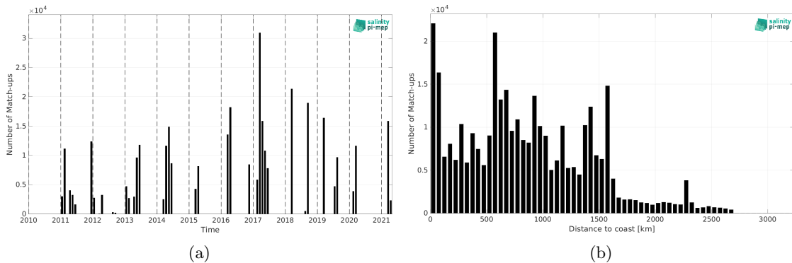
Figure 1: Number of match-ups between TSG (GOSUD-Research-vessel) and SMOS SSS L4 v2 - Daily (BEC) SSS as a function of time (a) and as function of the distance to coast (b) over the South Atlantic Ocean Pi-MEP region and for the full satellite product period.
