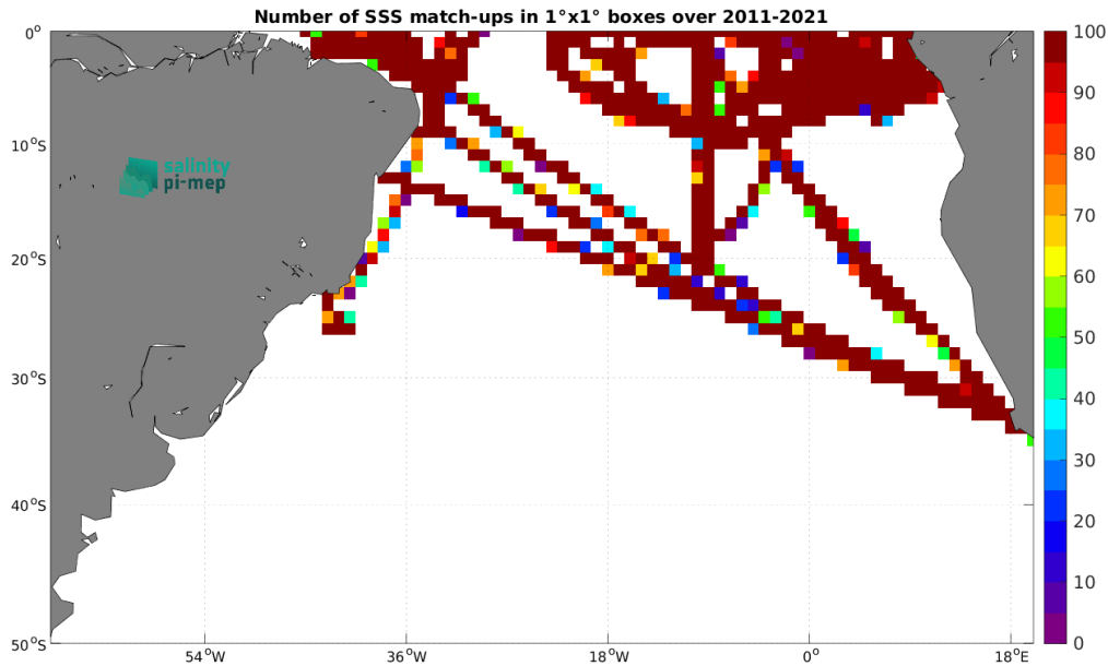
Figure 4: Number of SSS match-ups between TSG (GOSUD-Research-vessel) SSS and the SMOS SSS L4 v2 - Daily (BEC) SSS product for the South Atlantic Ocean Pi-MEP region over 1^\circ \times 1^\circ boxes and for the full satellite product period.
