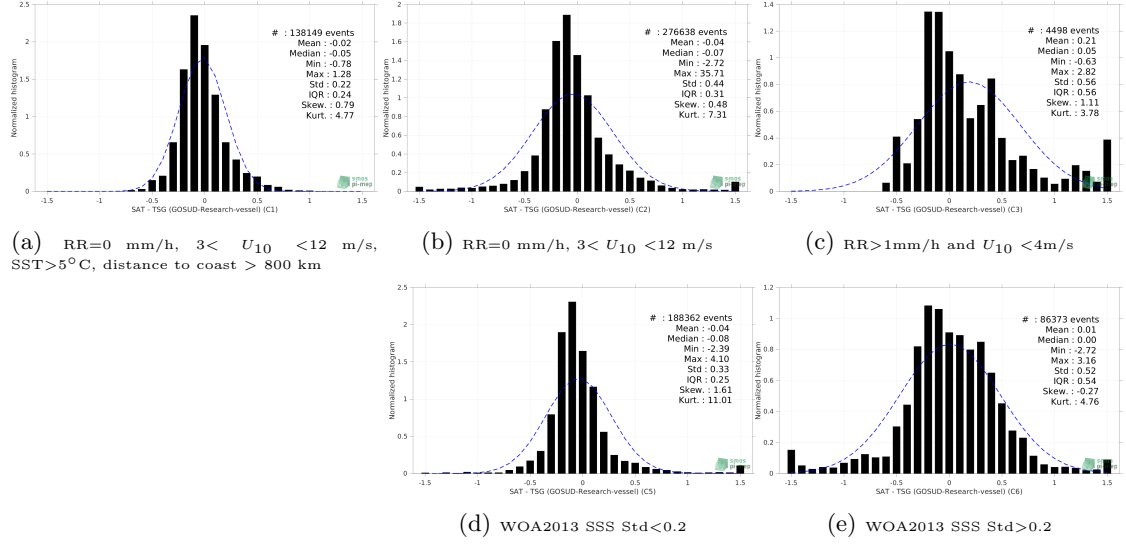
Figure 13: Normalized histogram of \Delta SSS (SMOS SSS L4 v2 - Daily (BEC) - TSG (GOSUD-Research-vessel)) for 5 different subdatasets corresponding to: RR=0 mm/h, 3 < U_{10} < 12 m/s, SST>5°C, distance to coast > 800 km (a), RR=0 mm/h, 3 < U_{10} < 12 m/s (b), RR>1mm/h and U_{10} < 4 m/s (c), WOA2013 SSS Std<0.2 (d), WOA2013 SSS Std>0.2 (e).
