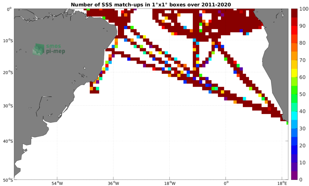
Figure 4: Number of SSS match-ups between TSG (GOSUD-Research-vessel) SSS and the SMOS SSS L4 v2 - Daily (BEC) SSS product for the South Atlantic Ocean Pi-MEP region over 1^{\circ} \times 1^{\circ} boxes and for the full satellite product period.
