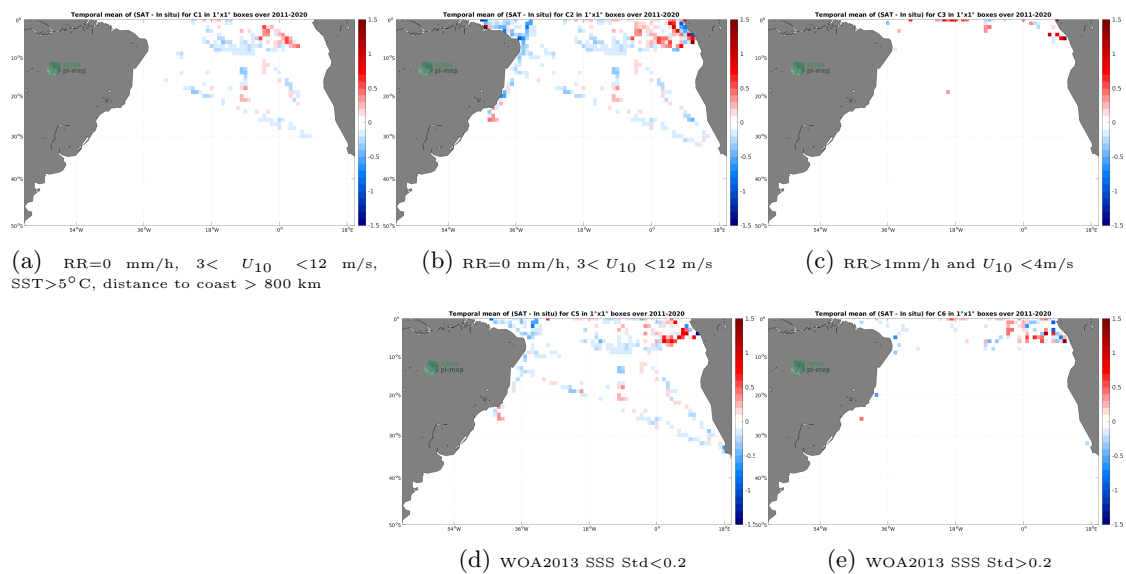
Figure 12: Temporal mean gridded over spatial boxes of size 1^\circ \times 1^\circ of \Delta\text{SSS} (SMOS SSS L4 v2 - Daily (BEC) - TSG (GOSUD-Research-vessel)) for 5 different subdatasets corresponding to:RR=0 mm/h, 3 < U_{10} < 12 m/s, SST>5°C, distance to coast > 800 km (a), RR=0 mm/h, 3 < U_{10} < 12 m/s (b), RR>1mm/h and U_{10} < 4 m/s (c), WOA2013 SSS Std<0.2 (d), WOA2013 SSS Std>0.2 (e).
