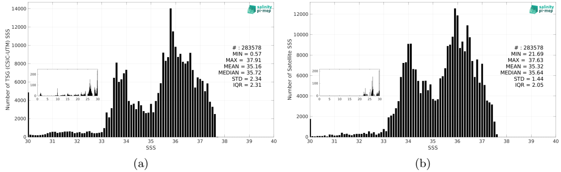
Figure 3: Histograms of SSS from TSG (CSIC-UTM) (a) and SMOS SSS L4 v2 - Daily (BEC) (b) considering all match-up pairs per bins of 0.1 over the South Atlantic Ocean Pi-MEP region and for the full satellite product period.
