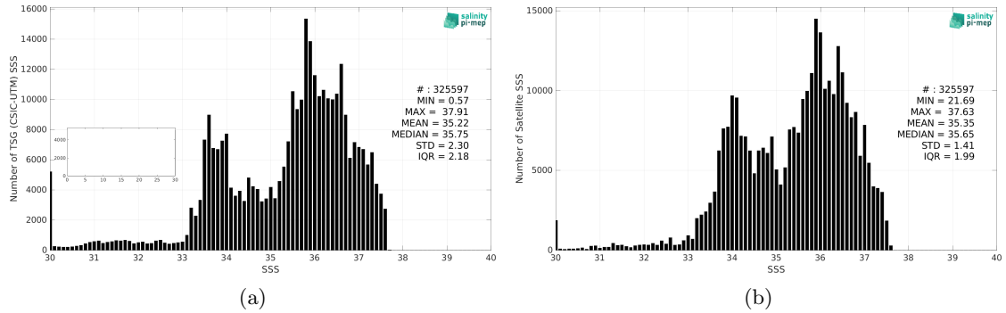
Figure 2: Histograms of SSS from TSG (CSIC-UTM) (a) and SMOS SSS L4 v2 - Daily (BEC) (b) considering all match-up pairs per bins of 0.1 over the South Atlantic Ocean Pi-MEP region and for the full satellite product period.
