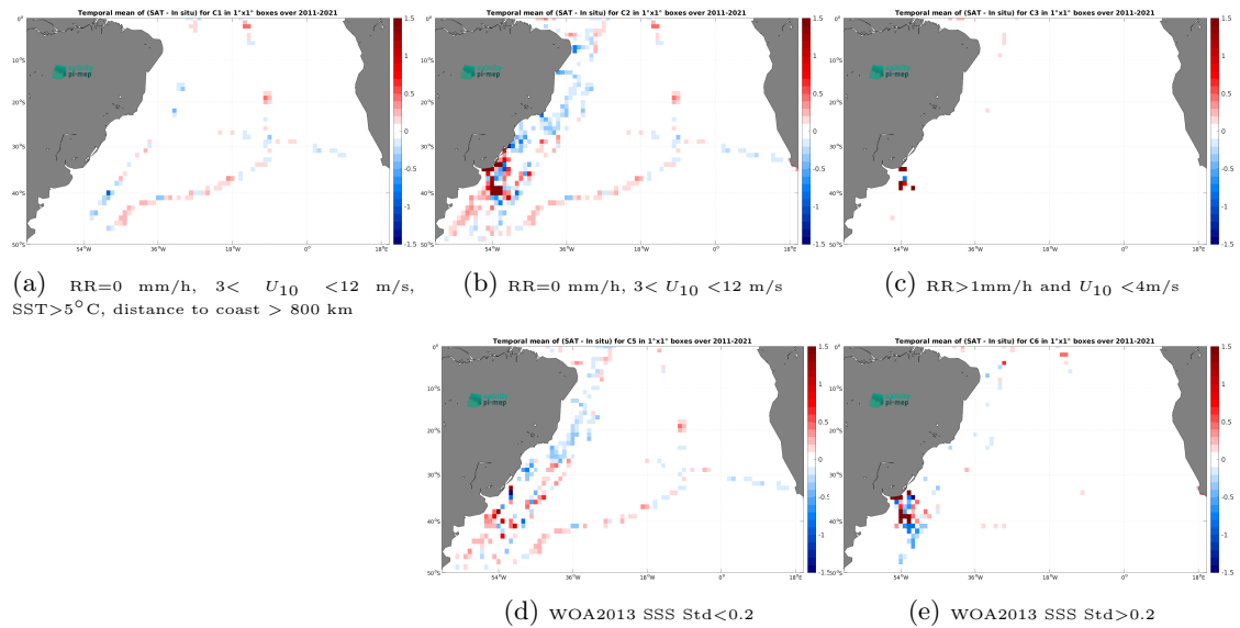
Figure 12: Temporal mean gridded over spatial boxes of size 1^\circ \times 1^\circ of \Delta SSS (SMOS SSS L4 v2 - Daily (BEC) - TSG (CSIC-UTM)) for 5 different subdatasets corresponding to:RR=0 mm/h, 3 < U_{10} < 12 m/s, SST >5^\circ\text{C} , distance to coast > 800 km (a), RR=0 mm/h, 3 < U_{10} < 12 m/s (b), RR >1 mm/h and U_{10} < 4 m/s (c), WOA2013 SSS Std <0.2 (d), WOA2013 SSS Std >0.2 (e).
