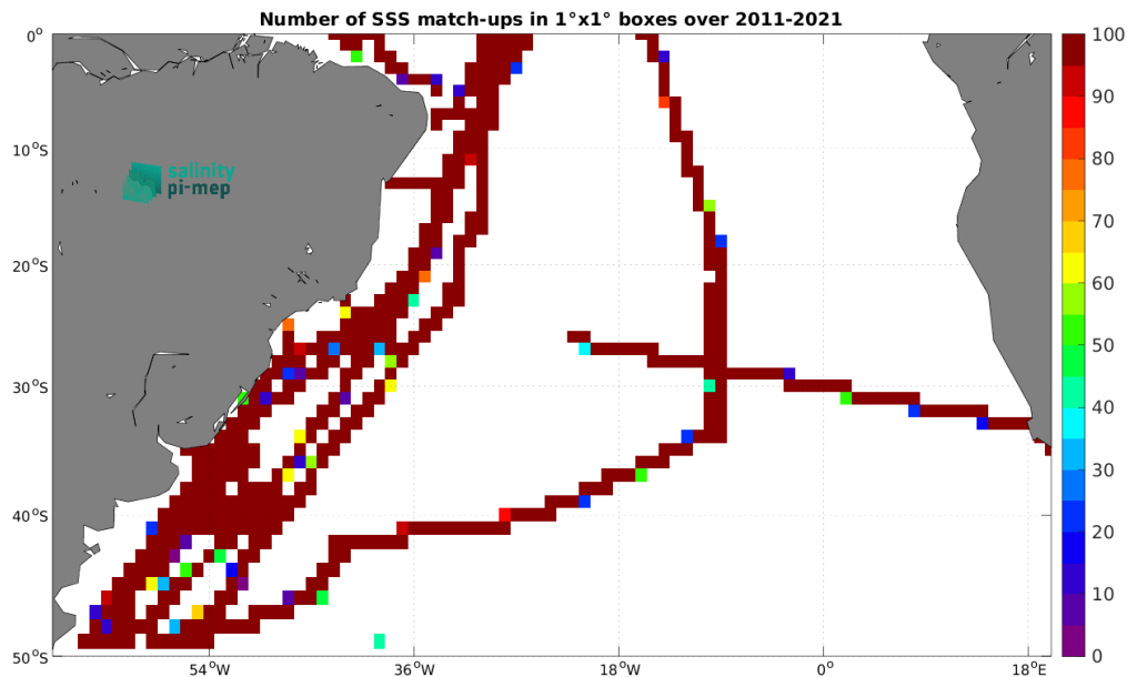
Figure 4: Number of SSS match-ups between TSG (CSIC-UTM) SSS and the SMOS SSS L4 v2 - Daily (BEC) SSS product for the South Atlantic Ocean Pi-MEP region over 1^\circ \times 1^\circ boxes and for the full satellite product period.
