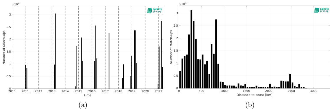
Figure 1: Number of match-ups between TSG (CSIC-UTM) and SMOS SSS L4 v2 - Daily (BEC) SSS as a function of time (a) and as function of the distance to coast (b) over the South Atlantic Ocean Pi-MEP region and for the full satellite product period.
