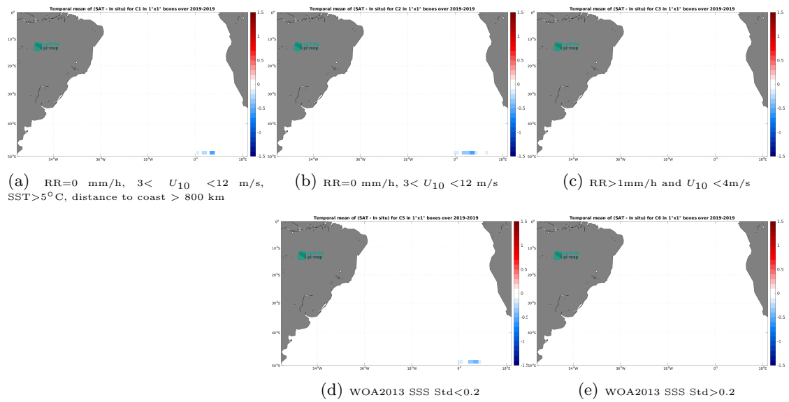
Figure 14: Temporal mean gridded over spatial boxes of size 1^\circ \times 1^\circ of \Delta SSS (SMOS SSS L4 v2 - Daily (BEC) - Saildrone) for 5 different subdatasets corresponding to:RR=0 mm/h, 3 < U_{10} < 12 m/s, SST>5°C, distance to coast > 800 km (a), RR=0 mm/h, 3 < U_{10} < 12 m/s (b), RR>1mm/h and U_{10} < 4 m/s (c), WOA2013 SSS Std<0.2 (d), WOA2013 SSS Std>0.2 (e).
