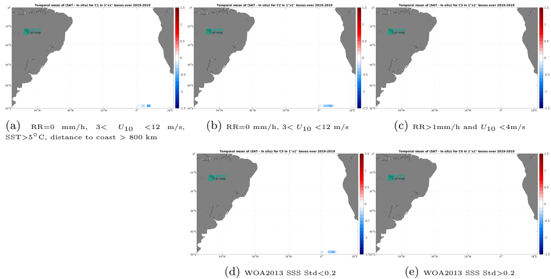
Figure 12: Temporal mean gridded over spatial boxes of size 1^{\circ}\times 1^{\circ} of \Delta\text{SSS} (SMOS SSS L4 v2 - Daily (BEC) - Sairdrone) for 5 different subdatasets corresponding to:RR=0 mm/h, 3 < U_{10} < 12 m/s, SST >5^{\circ}\text{C} , distance to coast > 800 km (a), RR=0 mm/h, 3 < U_{10} < 12 m/s (b), RR >1 mm/h and U_{10} < 4 m/s (c), WOA2013 SSS Std <0.2 (d), WOA2013 SSS Std >0.2 (e).
