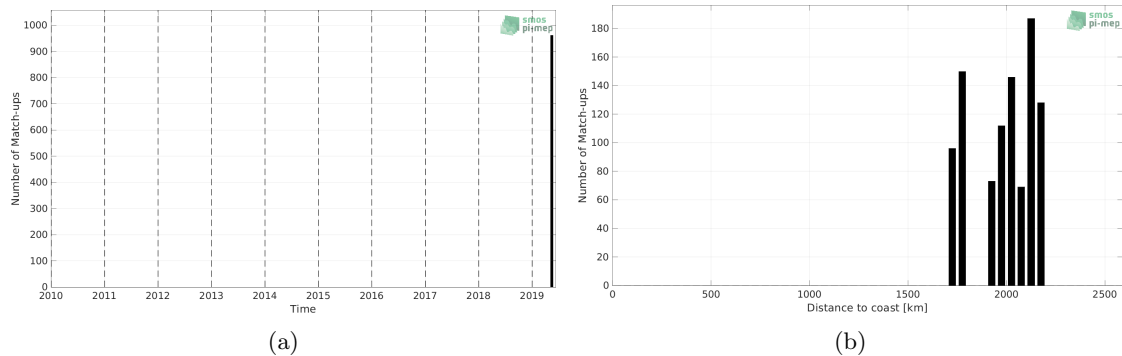
Figure 1: Number of match-ups between Saildrone and SMOS SSS L4 v2 - Daily (BEC) SSS as a function of time (a) and as function of the distance to coast (b) over the South Atlantic Ocean Pi-MEP region and for the full satellite product period.
