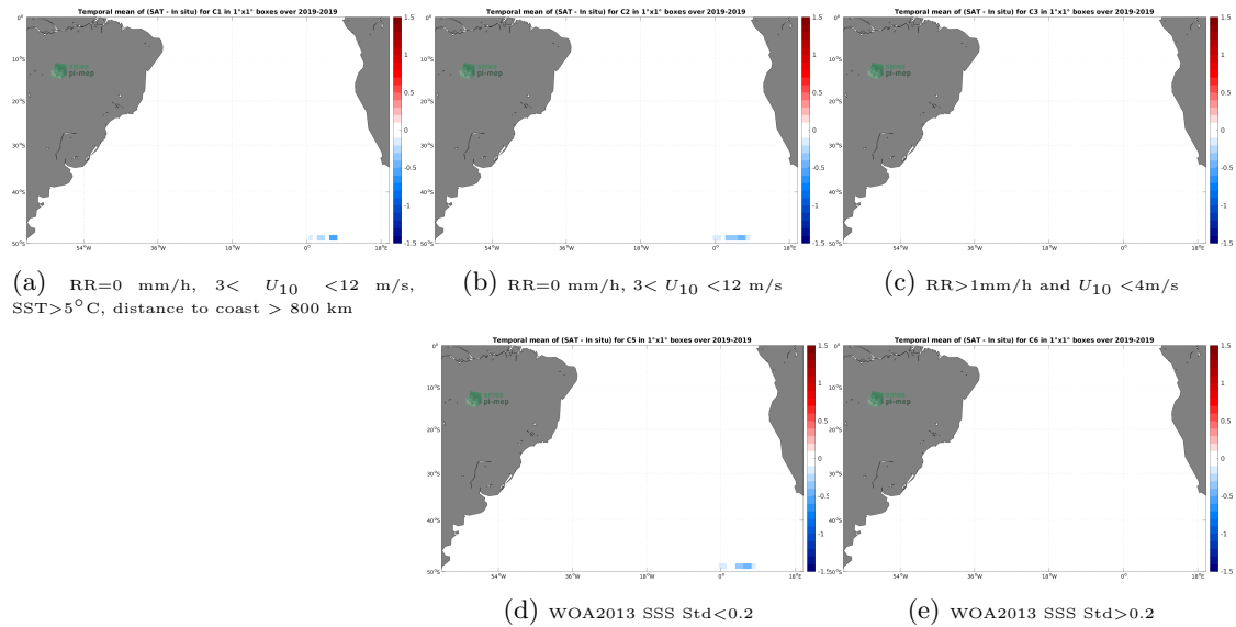
Figure 12: Temporal mean gridded over spatial boxes of size 1^{\circ}\times 1^{\circ} of \Delta\text{SSS} (SMOS SSS L4 v2 - Daily (BEC) - Saiddrone) for 5 different subdatasets corresponding to:RR=0 mm/h, 3 < U_{10} < 12 m/s, SST >5^{\circ}\text{C} , distance to coast > 800 km (a), RR=0 mm/h, 3 < U_{10} < 12 m/s (b), RR >1 mm/h and U_{10} < 4 m/s (c), WOA2013 SSS Std <0.2 (d), WOA2013 SSS Std >0.2 (e).
