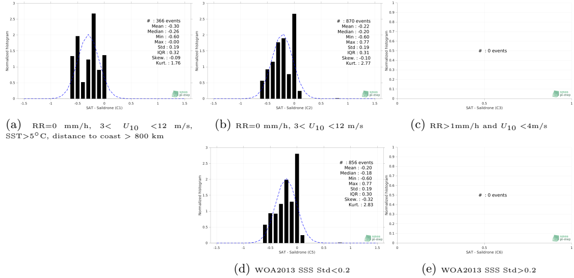
Figure 13: Normalized histogram of \Delta SSS (SMOS SSS L4 v2 - Daily (BEC) - Saildrone) for 5 different subdatasets corresponding to: RR=0 mm/h, 3 < U_{10} < 12 m/s, SST > 5°C, distance to coast > 800 km (a), RR=0 mm/h, 3 < U_{10} < 12 m/s (b), RR > 1mm/h and U_{10} < 4 m/s (c), WOA2013 SSS Std < 0.2 (d), WOA2013 SSS Std > 0.2 (e).
