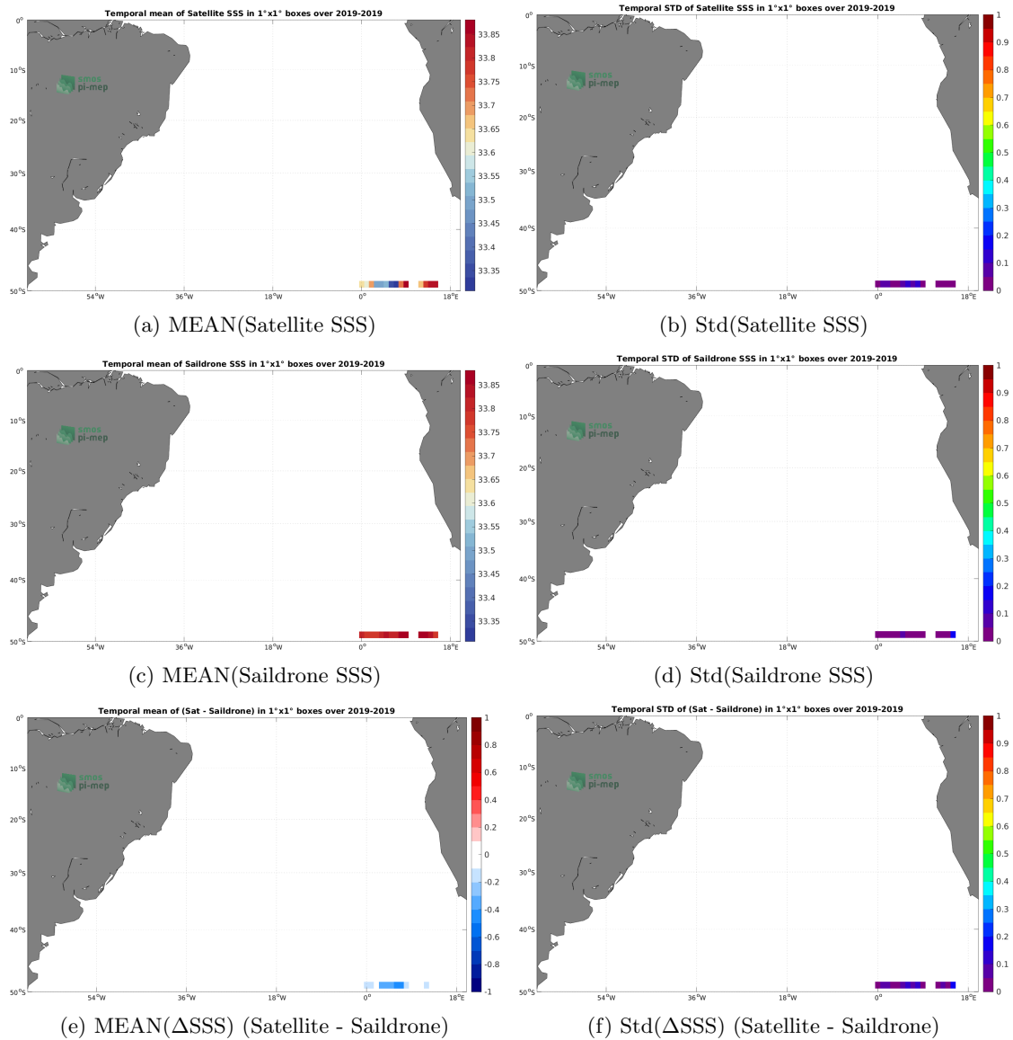
Figure 6: Temporal mean (left) and Std (right) of SSS from SMOS SSS L4 v2 - Daily (BEC) (top), Saildrone (middle), and of \Delta SSS (Satellite - Saildrone). Only match-up pairs are used to generate these maps.
