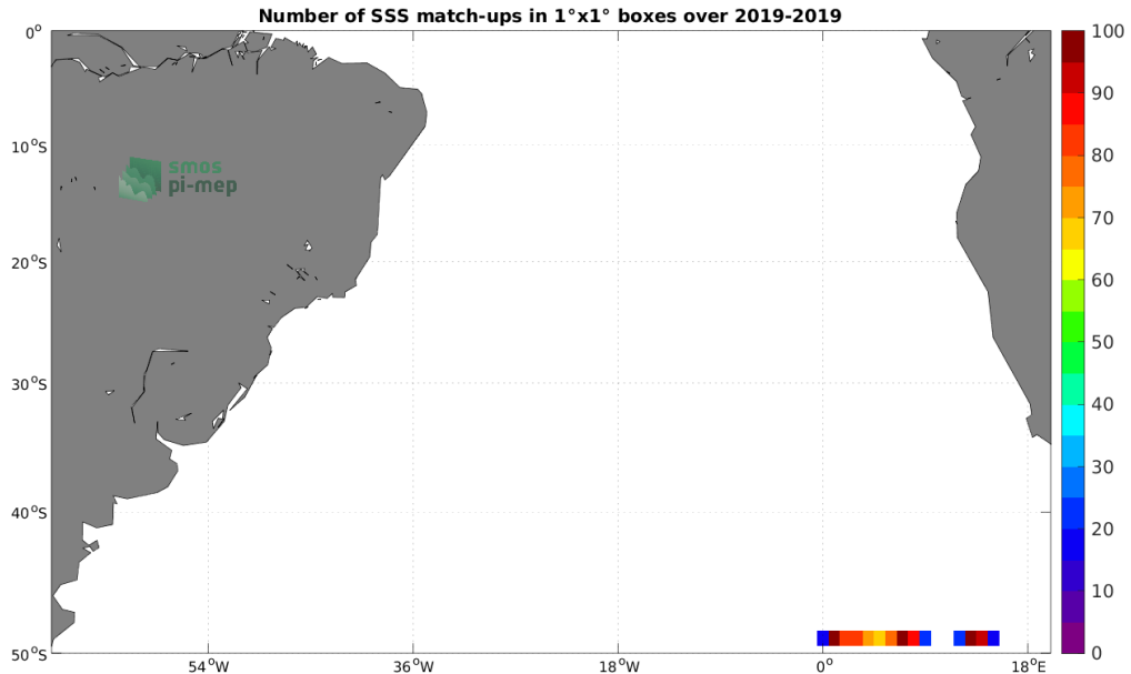
Figure 4: Number of SSS match-ups between Saildrone SSS and the SMOS SSS L4 v2 - Daily (BEC) SSS product for the South Atlantic Ocean Pi-MEP region over 1^\circ \times 1^\circ boxes and for the full satellite product period.
