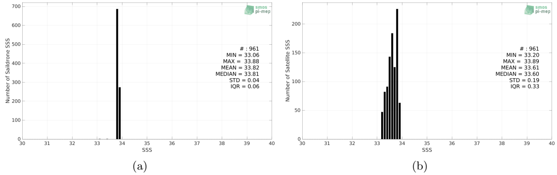
Figure 2: Histograms of SSS from Saildrone (a) and SMOS SSS L4 v2 - Daily (BEC) (b) considering all match-up pairs per bins of 0.1 over the South Atlantic Ocean Pi-MEP region and for the full satellite product period.
