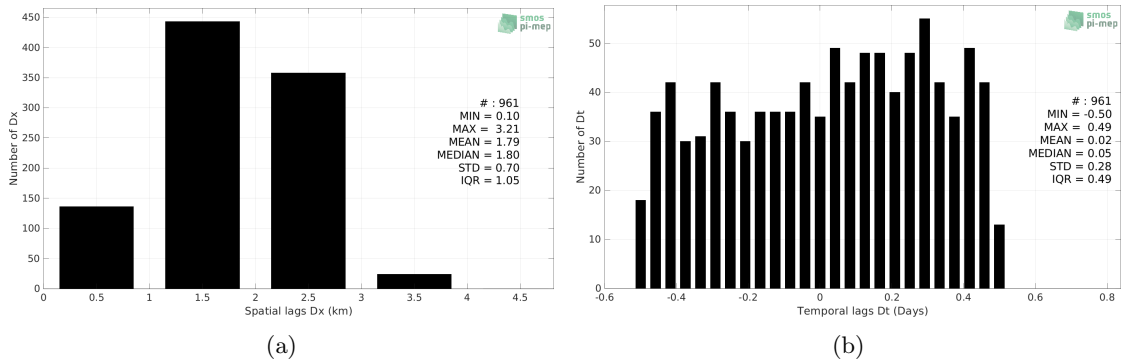
Figure 5: Histograms of the spatial (a) and temporal (b) lags between the location/time of the Saildrone measurement and the date of the corresponding SMOS SSS L4 v2 - Daily (BEC) SSS pixel.
