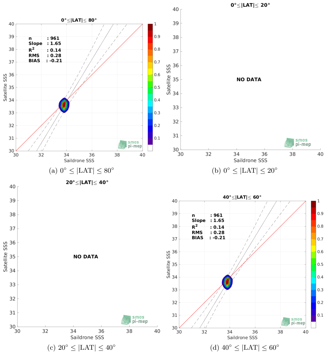
Figure 9: Contour maps of the concentration of SMOS SSS L4 v2 - Daily (BEC) SSS (y-axis) versus Saildrone SSS (x-axis) at match-up pairs for different latitude bands. For each plot, the red line shows x=y . The black thin and dashed lines indicate a linear fit through the data cloud and the \pm 95\% confidence levels, respectively. The number match-up pairs n , the slope and R^2 coefficient of the linear fit, the root mean square (RMS) and the mean bias between satellite and in situ data are indicated for each latitude band in each plots.
