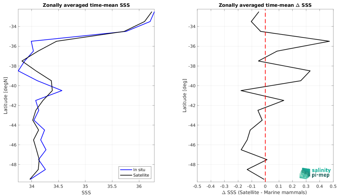
Figure 8: Left panel: Zonal mean SSS from SMOS SSS L4 v2 - Daily (BEC) satellite product (black) and from Marine mammals (blue). Right panel: Zonal mean of \Delta SSS (Satellite - Marine mammals) for all the collected Pi-MEP match-up pairs estimated over the full satellite product period.
