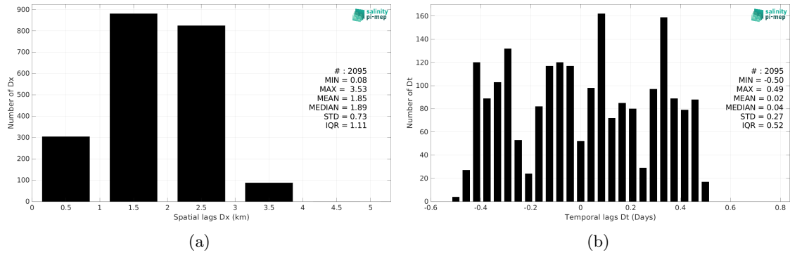
Figure 5: Histograms of the spatial (a) and temporal (b) lags between the location/time of the Marine mammals measurement and the date of the corresponding SMOS SSS L4 v2 - Daily (BEC) SSS pixel.
