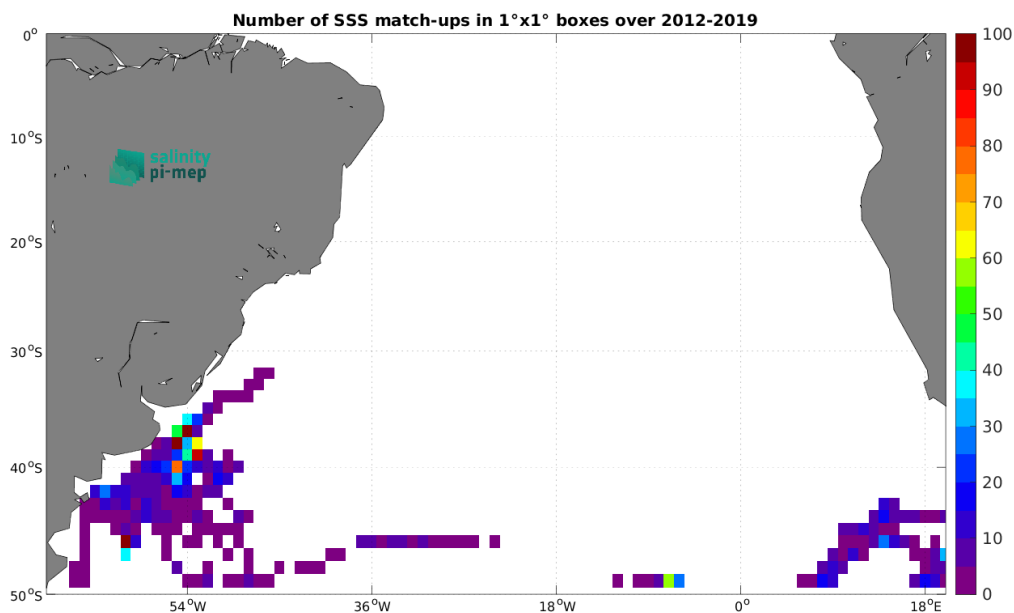
Figure 4: Number of SSS match-ups between Marine mammals SSS and the SMOS SSS L4 v2 - Daily (BEC) SSS product for the South Atlantic Ocean Pi-MEP region over 1^\circ \times 1^\circ boxes and for the full satellite product period.
