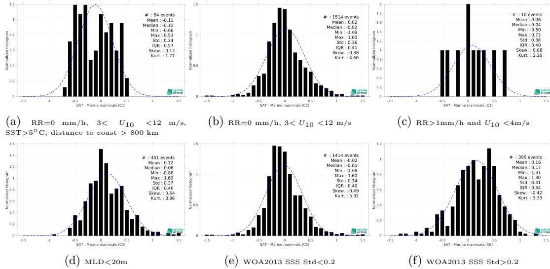
Figure 13: Normalized histogram of \Delta SSS (SMOS SSS L4 v2 - Daily (BEC) - Marine mammals) for 6 different subdatasets corresponding to: RR=0 mm/h, 3 < U_{10} < 12 m/s, SST>5°C, distance to coast > 800 km (a), RR=0 mm/h, 3 < U_{10} < 12 m/s (b), RR>1mm/h and U_{10} < 4 m/s (c), MLD<20m (d), WOA2013 SSS Std<0.2 (e), WOA2013 SSS Std>0.2 (f).
