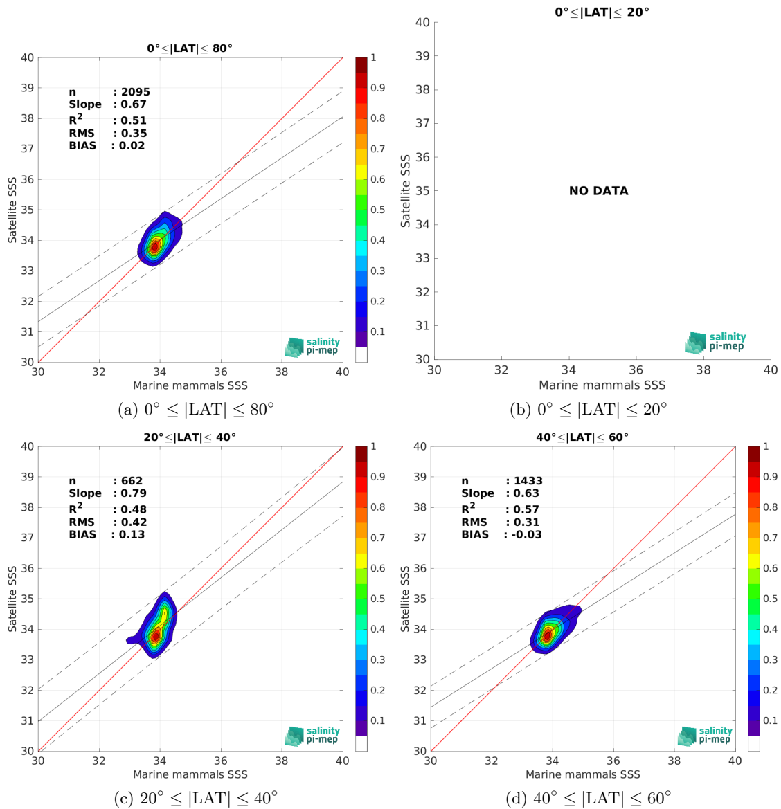
Figure 9: Contour maps of the concentration of SMOS SSS L4 v2 - Daily (BEC) SSS (y-axis) versus Marine mammals SSS (x-axis) at match-up pairs for different latitude bands. For each plot, the red line shows x=y . The black thin and dashed lines indicate a linear fit through the data cloud and the \pm 95\% confidence levels, respectively. The number match-up pairs n , the slope and R^2 coefficient of the linear fit, the root mean square (RMS) and the mean bias between satellite and in situ data are indicated for each latitude band in each plots.
