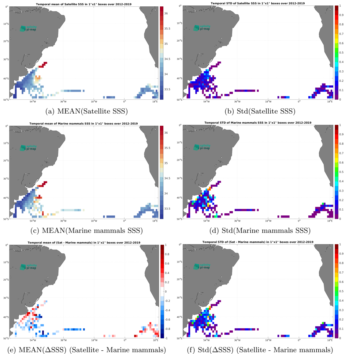
Figure 6: Temporal mean (left) and Std (right) of SSS from SMOS SSS L4 v2 - Daily (BEC) (top), Marine mammals (middle), and of \Delta SSS (Satellite - Marine mammals). Only match-up pairs are used to generate these maps.
