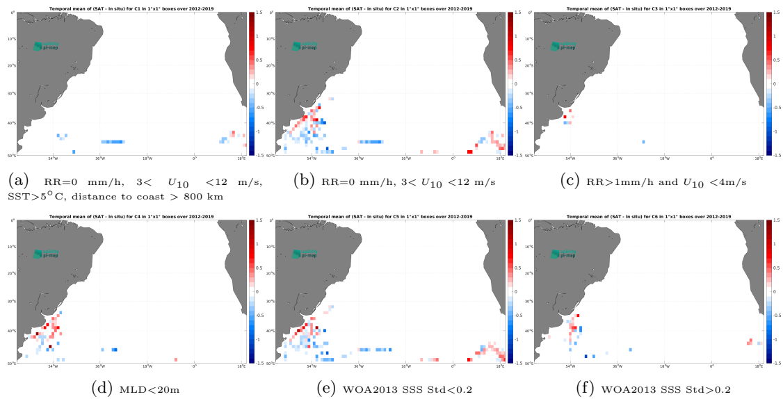
Figure 12: Temporal mean gridded over spatial boxes of size 1^\circ \times 1^\circ of \Delta SSS (SMOS SSS L4 v2 - Daily (BEC) - Marine mammals) for 6 different subdatasets corresponding to:RR=0 mm/h, 3 < U_{10} < 12 m/s, SST > 5^\circ\text{C} , distance to coast > 800 km (a), RR=0 mm/h, 3 < U_{10} < 12 m/s (b), RR > 1 mm/h and U_{10} < 4 m/s (c),MLD < 20 m (d),WOA2013 SSS Std < 0.2 (e),WOA2013 SSS Std > 0.2 (f).
