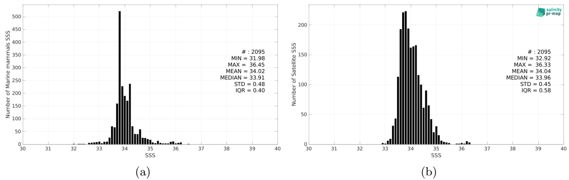
Figure 2: Histograms of SSS from Marine mammals (a) and SMOS SSS L4 v2 - Daily (BEC) (b) considering all match-up pairs per bins of 0.1 over the South Atlantic Ocean Pi-MEP region and for the full satellite product period.
