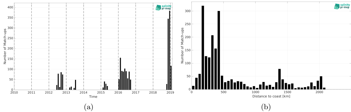
Figure 1: Number of match-ups between Marine mammals and SMOS SSS L4 v2 - Daily (BEC) SSS as a function of time (a) and as function of the distance to coast (b) over the South Atlantic Ocean Pi-MEP region and for the full satellite product period.
