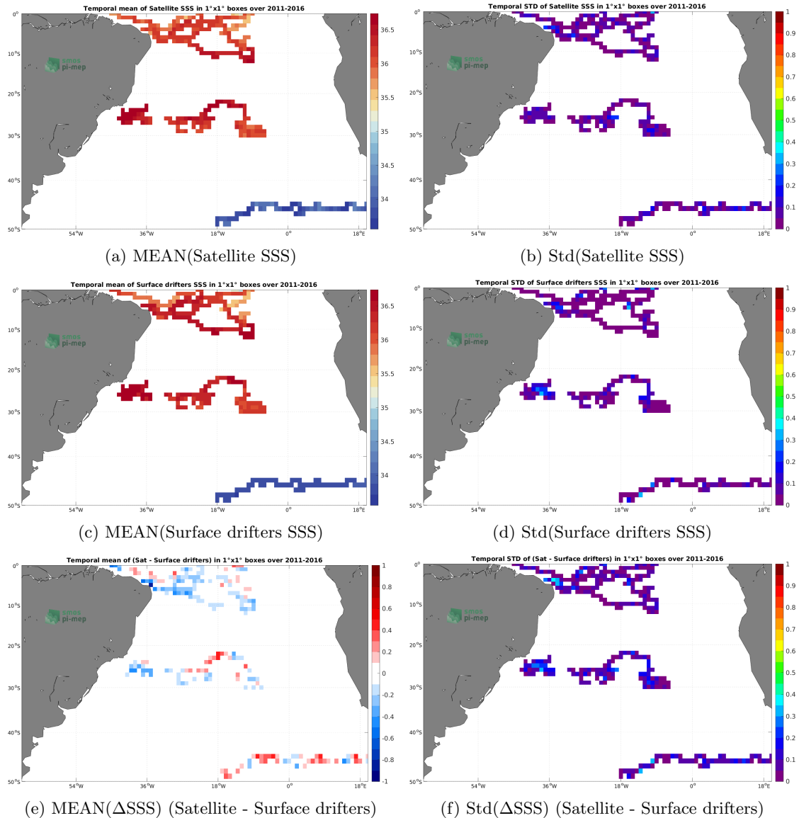
Figure 5: Temporal mean (left) and Std (right) of SSS from SMOS SSS L4 v2 - Daily (BEC) (top), Surface drifters (middle), and of \Delta SSS (Satellite - Surface drifters). Only match-up pairs are used to generate these maps.
