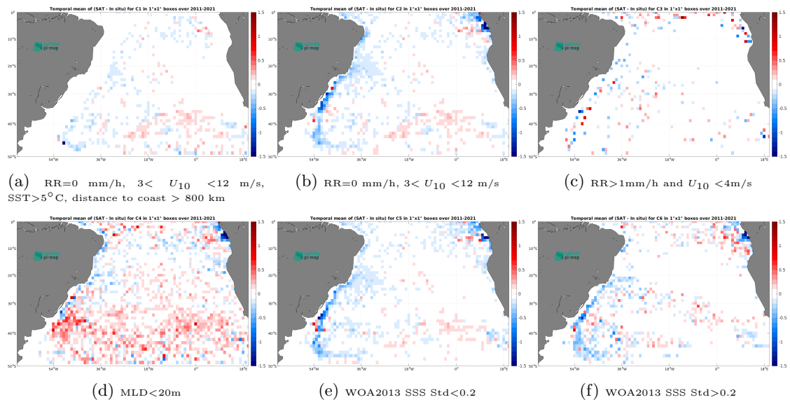
Figure 12: Temporal mean gridded over spatial boxes of size 1^\circ \times 1^\circ of \Delta SSS (SMOS SSS L4 v2 - Daily (BEC) - Argo) for 6 different subdatasets corresponding to:RR=0 mm/h, 3 < U_{10} < 12 m/s, SST >5^\circ C, distance to coast > 800 km (a), RR=0 mm/h, 3 < U_{10} < 12 m/s (b), RR >1 mm/h and U_{10} < 4 m/s (c),MLD <20 m (d),WOA2013 SSS Std <0.2 (e),WOA2013 SSS Std >0.2 (f).
