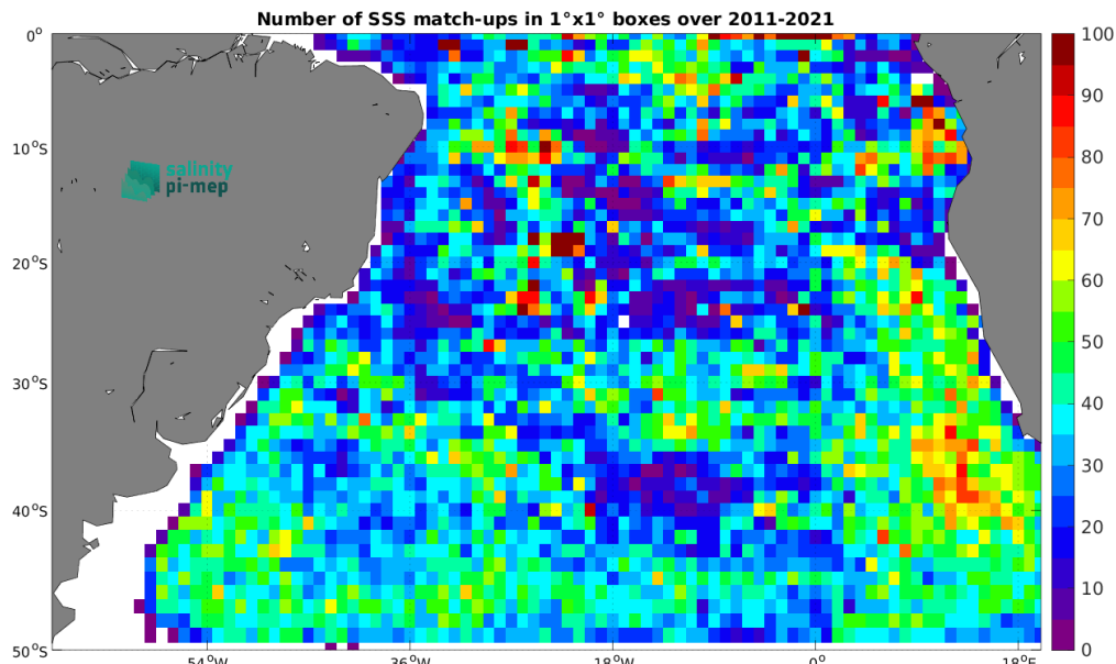
Figure 4: Number of SSS match-ups between Argo SSS and the SMOS SSS L4 v2 - Daily (BEC) SSS product for the South Atlantic Ocean Pi-MEP region over 1^\circ \times 1^\circ boxes and for the full satellite product period.
