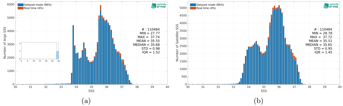
Figure 2: Histograms of SSS from Argo (a) and SMOS SSS L4 v2 - Daily (BEC) (b) considering all match-up pairs per bins of 0.1 over the South Atlantic Ocean Pi-MEP region and for the full satellite product period.
