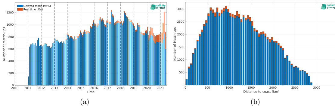
Figure 1: Number of match-ups between Argo and SMOS SSS L4 v2 - Daily (BEC) SSS as a function of time (a) and as function of the distance to coast (b) over the South Atlantic Ocean Pi-MEP region and for the full satellite product period.
