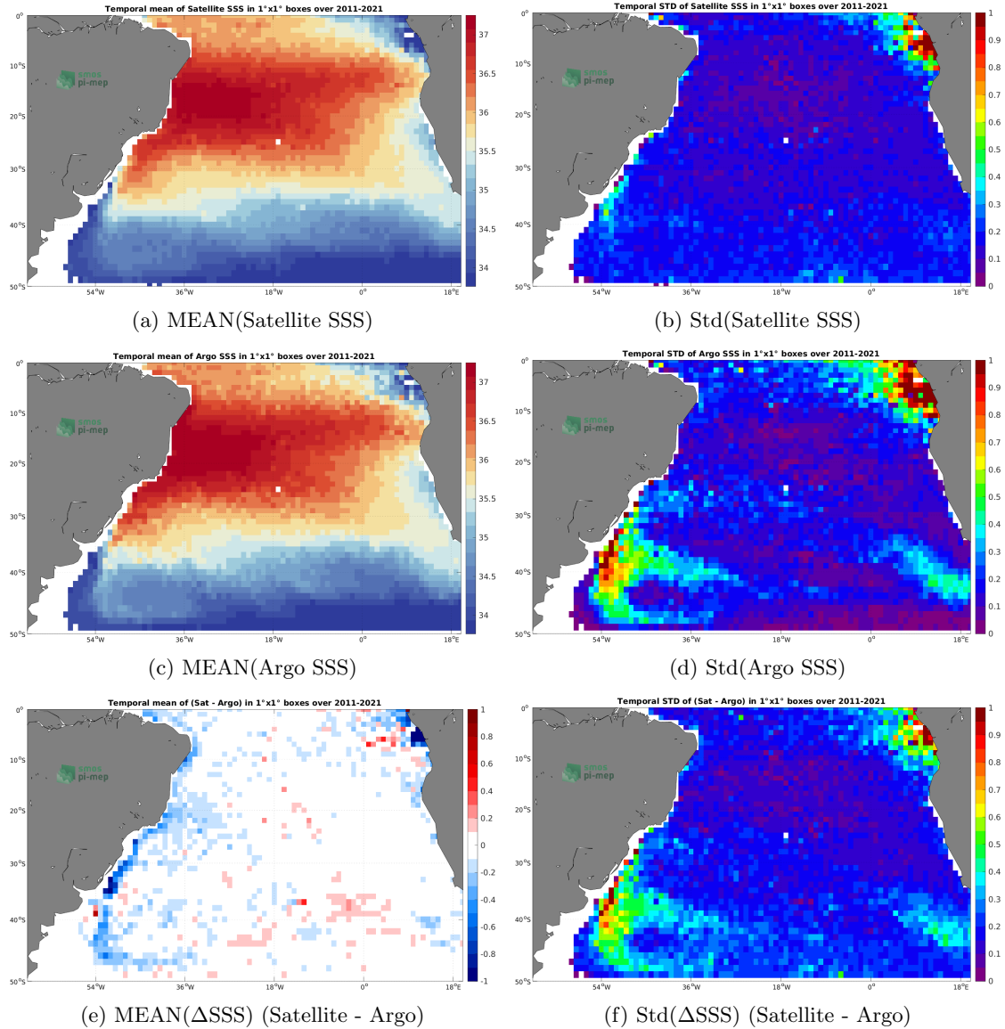
Figure 6: Temporal mean (left) and Std (right) of SSS from SMOS SSS L4 v2 - Daily (BEC) (top), Argo (middle), and of \Delta SSS (Satellite - Argo). Only match-up pairs are used to generate these maps.
