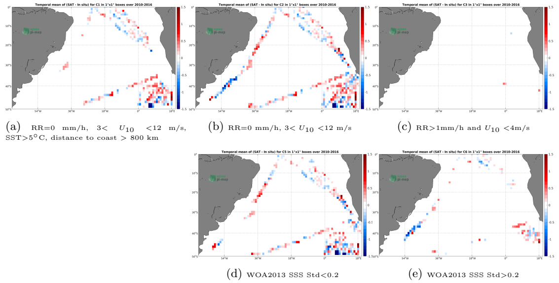
Figure 12: Temporal mean gridded over spatial boxes of size 1^\circ \times 1^\circ of \Delta SSS (SMOS SSS L3 v3 Monthly (ICDC) - TSG (Polarstern)) for 5 different subdatasets corresponding to: RR=0 mm/h, 3 < U_{10} < 12 m/s, SST > 5^\circ C , distance to coast > 800 km (a), RR=0 mm/h, 3 < U_{10} < 12 m/s (b), RR > 1 mm/h and U_{10} < 4 m/s (c), WOA2013 SSS Std < 0.2 (d), WOA2013 SSS Std > 0.2 (e).
