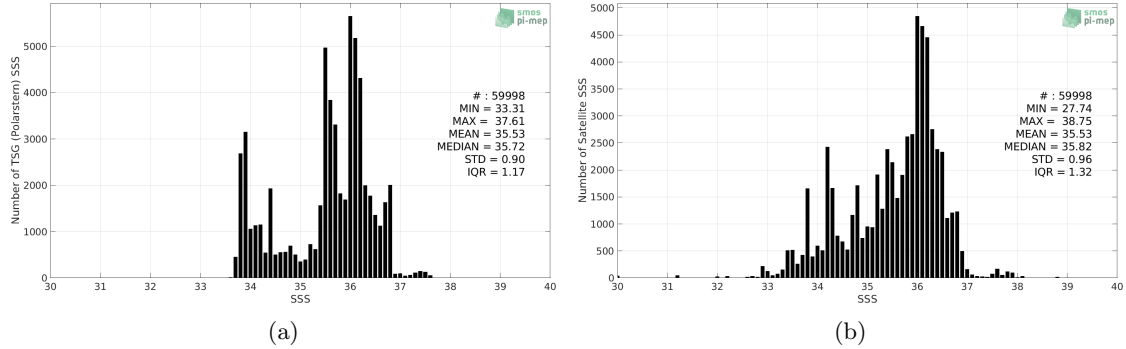
Figure 2: Histograms of SSS from TSG (Polarstern) (a) and SMOS SSS L3 v3 Monthly (ICDC) (b) considering all match-up pairs per bins of 0.1 over the South Atlantic Ocean Pi-MEP region and for the full satellite product period.
