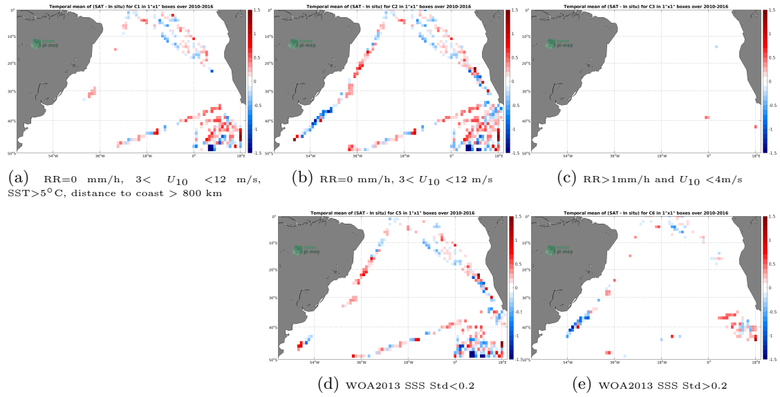
Figure 12: Temporal mean gridded over spatial boxes of size 1^\circ \times 1^\circ of \Delta SSS (SMOS SSS L3 v3 Monthly (ICDC) - TSG (Polarstern)) for 5 different subdatasets corresponding to: RR=0 mm/h, 3 < U_{10} < 12 m/s, SST > 5^\circ\text{C} , distance to coast > 800 km (a), RR=0 mm/h, 3 < U_{10} < 12 m/s (b), RR > 1 mm/h and U_{10} < 4 m/s (c), WOA2013 SSS Std < 0.2 (d), WOA2013 SSS Std > 0.2 (e).
