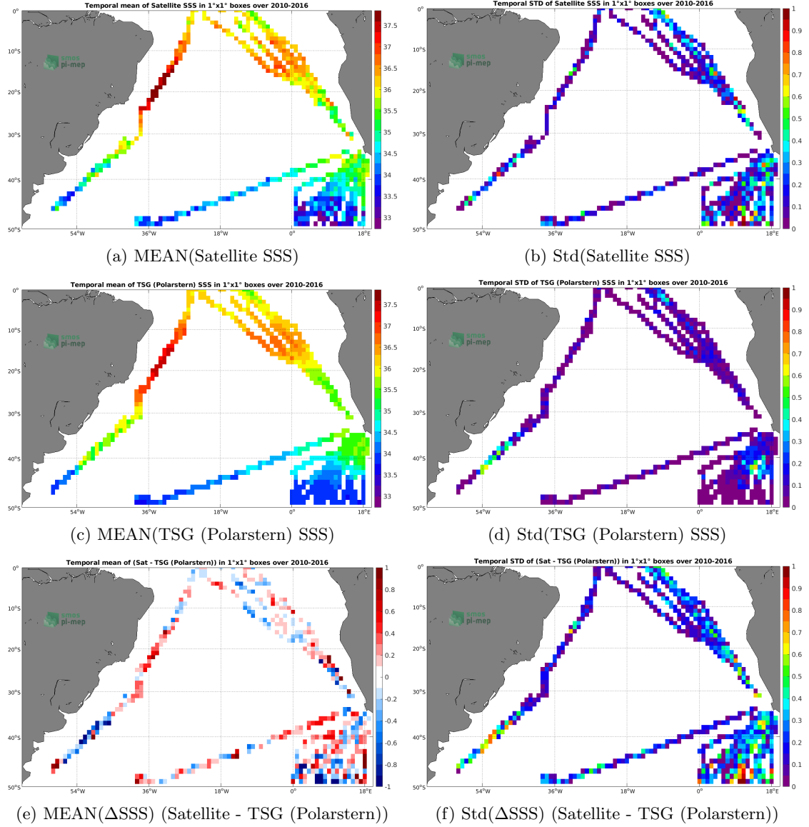
Figure 6: Temporal mean (left) and Std (right) of SSS from SMOS SSS L3 v3 Monthly (ICDC) (top), TSG (Polarstern) (middle), and of \Delta SSS (Satellite - TSG (Polarstern)). Only match-up pairs are used to generate these maps.
