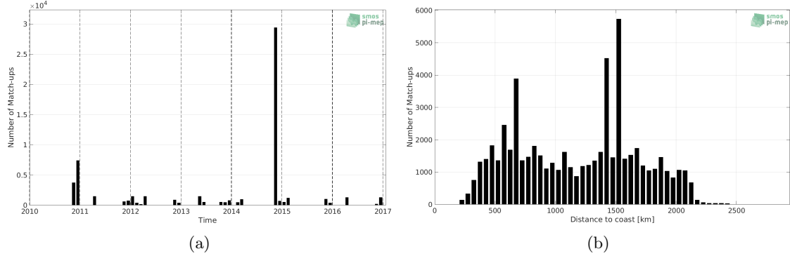
Figure 1: Number of match-ups between TSG (Polarstern) and SMOS SSS L3 v3 Monthly (ICDC) SSS as a function of time (a) and as function of the distance to coast (b) over the South Atlantic Ocean Pi-MEP region and for the full satellite product period.
