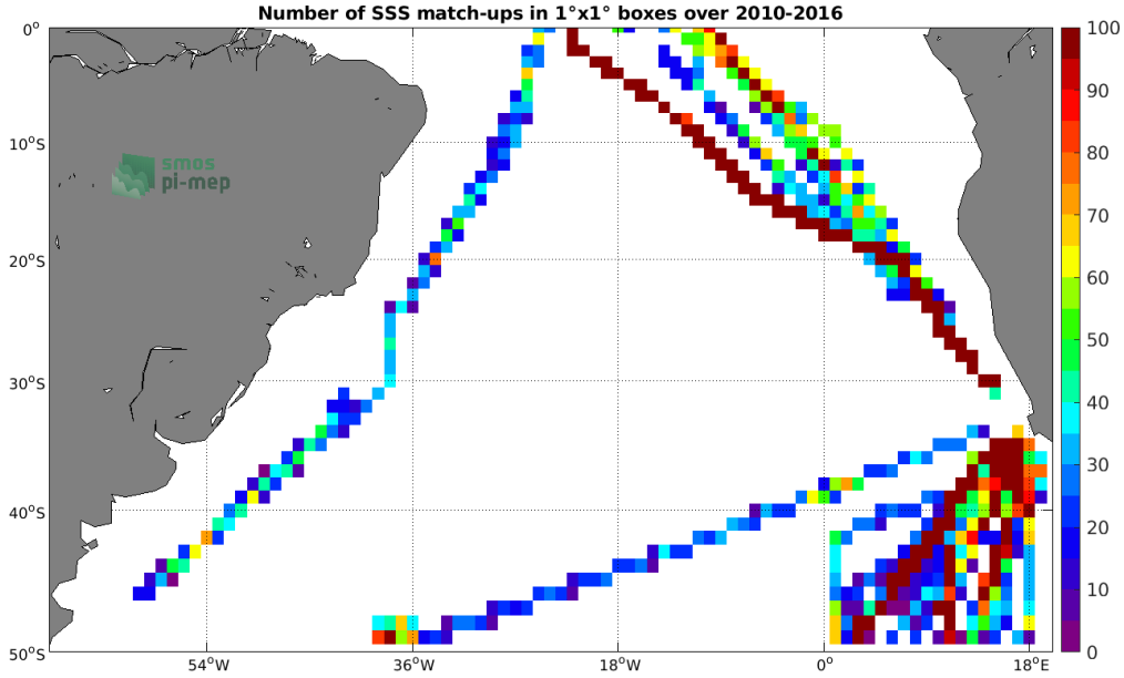
Figure 4: Number of SSS match-ups between TSG (Polarstern) SSS and the SMOS SSS L3 v3 Monthly (ICDC) SSS product for the South Atlantic Ocean Pi-MEP region over 1^\circ \times 1^\circ boxes and for the full satellite product period.
