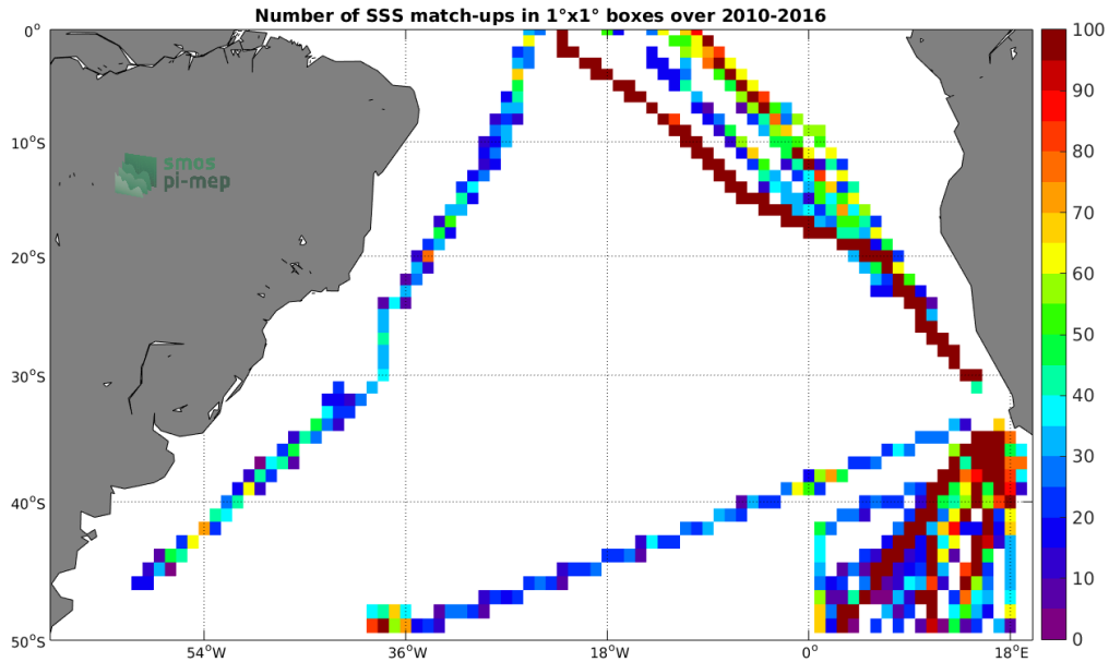
Figure 4: Number of SSS match-ups between TSG-POLARSTERN SSS and the SMOS-L3-ICDC-V3-MONTHLY-0.5DEG SSS product for the South Atlantic Ocean Pi-MEP region over 1^\circ \times 1^\circ boxes and for the full satellite product period.
