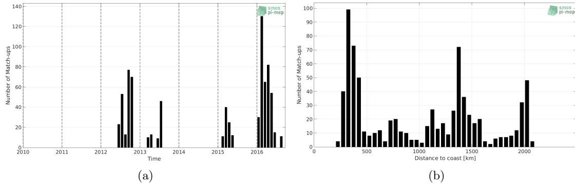
Figure 1: Number of match-ups between Marine mammals and SMOS SSS L3 v3 Monthly (ICDC) SSS as a function of time (a) and as function of the distance to coast (b) over the South Atlantic Ocean Pi-MEP region and for the full satellite product period.
