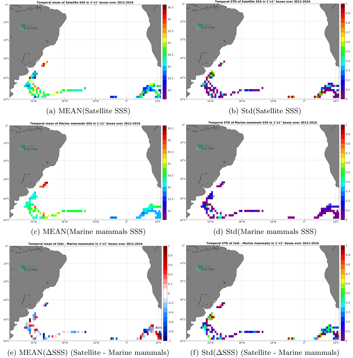
Figure 6: Temporal mean (left) and Std (right) of SSS from SMOS SSS L3 v3 Monthly (ICDC) (top), Marine mammals (middle), and of \Delta SSS (Satellite - Marine mammals). Only match-up pairs are used to generate these maps.
