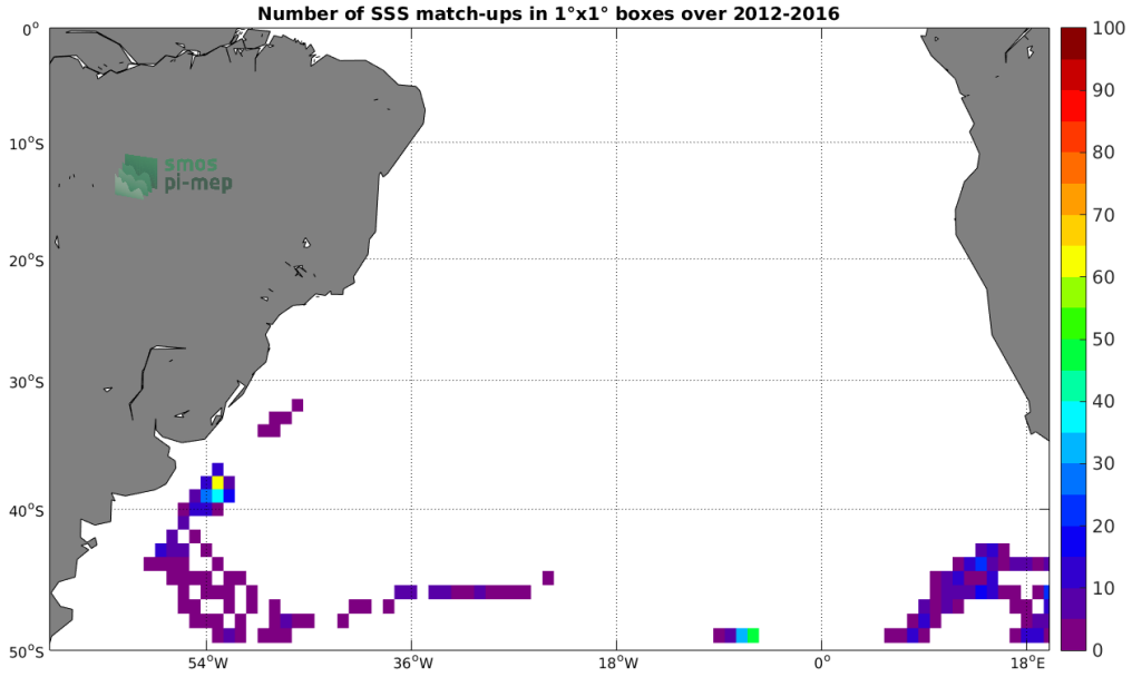
Figure 4: Number of SSS match-ups between Marine mammals SSS and the SMOS SSS L3 v3 Monthly (ICDC) SSS product for the South Atlantic Ocean Pi-MEP region over 1^\circ \times 1^\circ boxes and for the full satellite product period.
