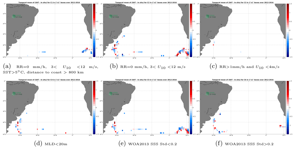
Figure 12: Temporal mean gridded over spatial boxes of size 1^\circ \times 1^\circ of \Delta SSS (SMOS SSS L3 v3 Monthly (ICDC) - Marine mammals) for 6 different subdatasets corresponding to: RR=0 mm/h, 3 < U_{10} < 12 m/s, SST > 5^\circ\text{C} , distance to coast > 800 km (a), RR=0 mm/h, 3 < U_{10} < 12 m/s (b), RR > 1 mm/h and U_{10} < 4 m/s (c), MLD < 20 m (d), WOA2013 SSS Std < 0.2 (e), WOA2013 SSS Std > 0.2 (f).
