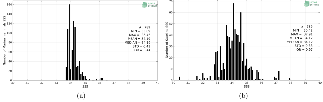
Figure 2: Histograms of SSS from Marine mammals (a) and SMOS SSS L3 v3 Monthly (ICDC) (b) considering all match-up pairs per bins of 0.1 over the South Atlantic Ocean Pi-MEP region and for the full satellite product period.
