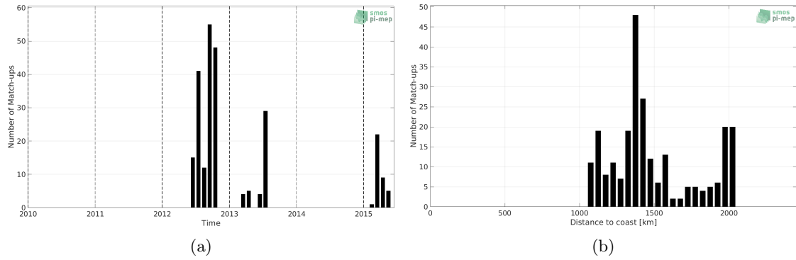
Figure 1: Number of match-ups between Sea mammals and SMOS SSS L3 v3 Monthly (ICDC) SSS as a function of time (a) and as function of the distance to coast (b) over the South Atlantic Ocean Pi-MEP region and for the full satellite product period.
