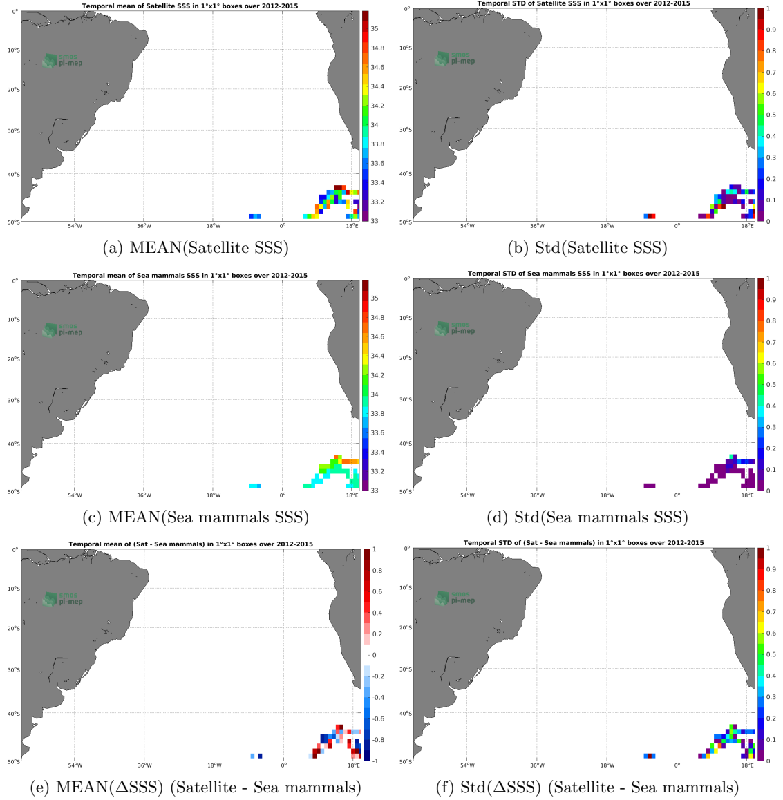
Figure 6: Temporal mean (left) and Std (right) of SSS from SMOS SSS L3 v3 Monthly (ICDC) (top), Sea mammals (middle), and of \Delta SSS (Satellite - Sea mammals). Only match-up pairs are used to generate these maps.
