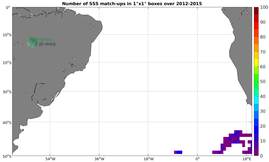
Figure 4: Number of SSS match-ups between Sea mammals SSS and the SMOS SSS L3 v3 Monthly (ICDC) SSS product for the South Atlantic Ocean Pi-MEP region over 1^\circ \times 1^\circ boxes and for the full satellite product period.
