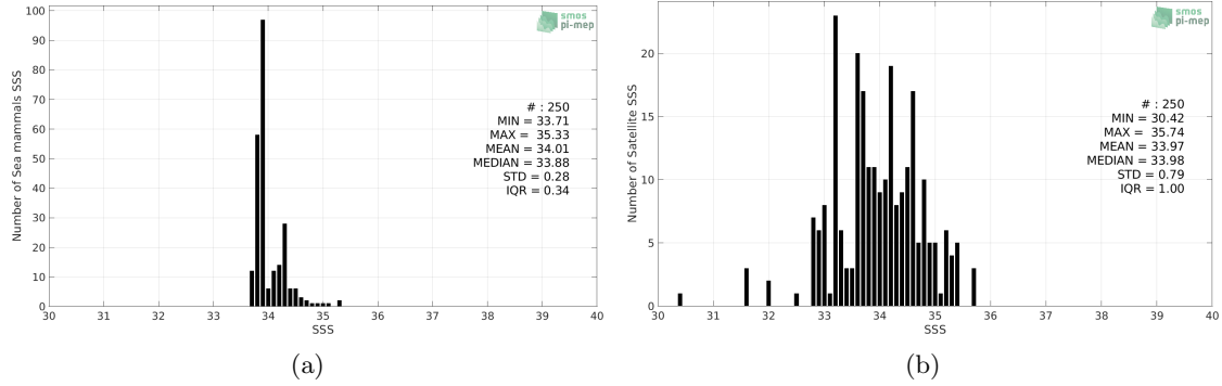
Figure 2: Histograms of SSS from Sea mammals (a) and SMOS SSS L3 v3 Monthly (ICDC) (b) considering all match-up pairs per bins of 0.1 over the South Atlantic Ocean Pi-MEP region and for the full satellite product period.
