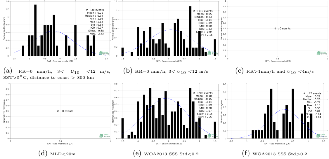
Figure 13: Normalized histogram of \Delta\text{SSS} (SMOS SSS L3 v3 Monthly (ICDC) - Sea mammals) for 6 different subdatasets corresponding to: RR=0 mm/h, 3 < U_{10} < 12 m/s, SST > 5^\circ\text{C} , distance to coast > 800 km (a), RR=0 mm/h, 3 < U_{10} < 12 m/s (b), RR > 1\text{mm/h} and U_{10} < 4\text{m/s} (c), MLD < 20\text{m} (d), WOA2013 SSS Std < 0.2 (e), WOA2013 SSS Std > 0.2 (f).
