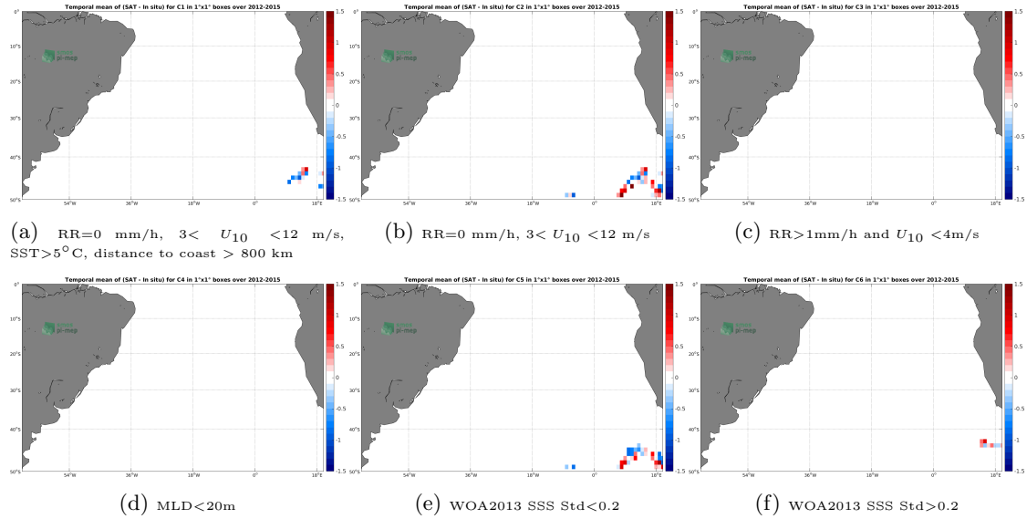
Figure 12: Temporal mean gridded over spatial boxes of size 1^{\circ}\times 1^{\circ} of \Delta\text{SSS} (SMOS-L3-ICDC-V3-MONTHLY-0.5DEG - Sea mammals) for 6 different subdatasets corresponding to:RR=0 mm/h, 3 < U_{10} < 12 m/s, SST >5^{\circ}\text{C} , distance to coast > 800 km (a), RR=0 mm/h, 3 < U_{10} < 12 m/s (b), RR >1 mm/h and U_{10} < 4 m/s (c),MLD <20 m (d),WOA2013 SSS Std <0.2 (e),WOA2013 SSS Std >0.2 (f).
