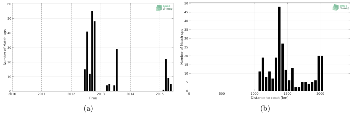
Figure 1: Number of match-ups between Sea mammals and SMOS-L3-ICDC-V3-MONTHLY-0.5DEG SSS as a function of time (a) and as function of the distance to coast (b) over the South Atlantic Ocean Pi-MEP region and for the full satellite product period.
