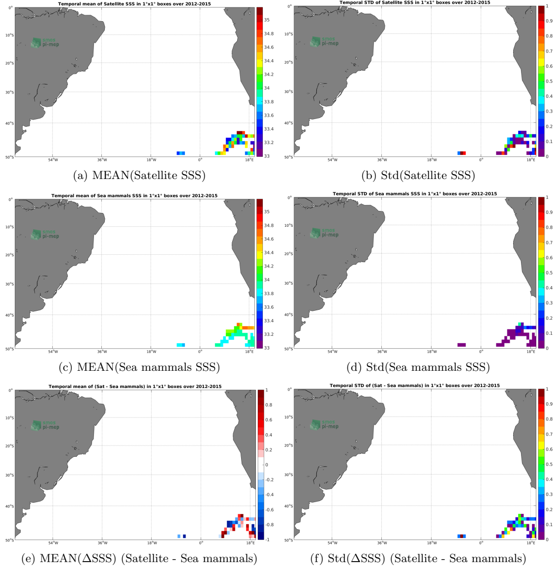
Figure 6: Temporal mean (left) and Std (right) of SSS from SMOS-L3-ICDC-V3-MONTHLY-0.5DEG (top), Sea mammals (middle), and of \Delta SSS (Satellite - Sea mammals). Only match-up pairs are used to generate these maps.
