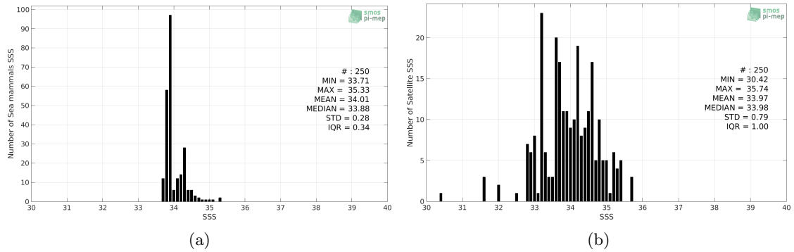
Figure 2: Histograms of SSS from Sea mammals (a) and SMOS-L3-ICDC-V3-MONTHLY-0.5DEG (b) considering all match-up pairs per bins of 0.1 over the South Atlantic Ocean Pi-MEP region and for the full satellite product period.
