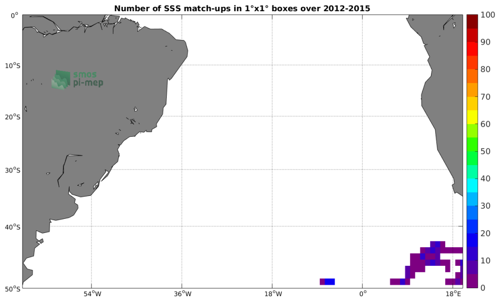
Figure 4: Number of SSS match-ups between Sea mammals SSS and the SMOS-L3-ICDC-V3-MONTHLY-0.5DEG SSS product for the South Atlantic Ocean Pi-MEP region over 1°x1° boxes and for the full satellite product period.
