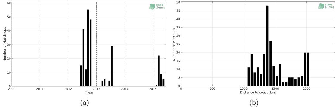
Figure 1: Number of match-ups between Sea mammals and SMOS-L3-ICDC-V3-MONTHLY-0.5DEG SSS as a function of time (a) and as function of the distance to coast (b) over the South Atlantic Ocean Pi-MEP region and for the full satellite product period.
