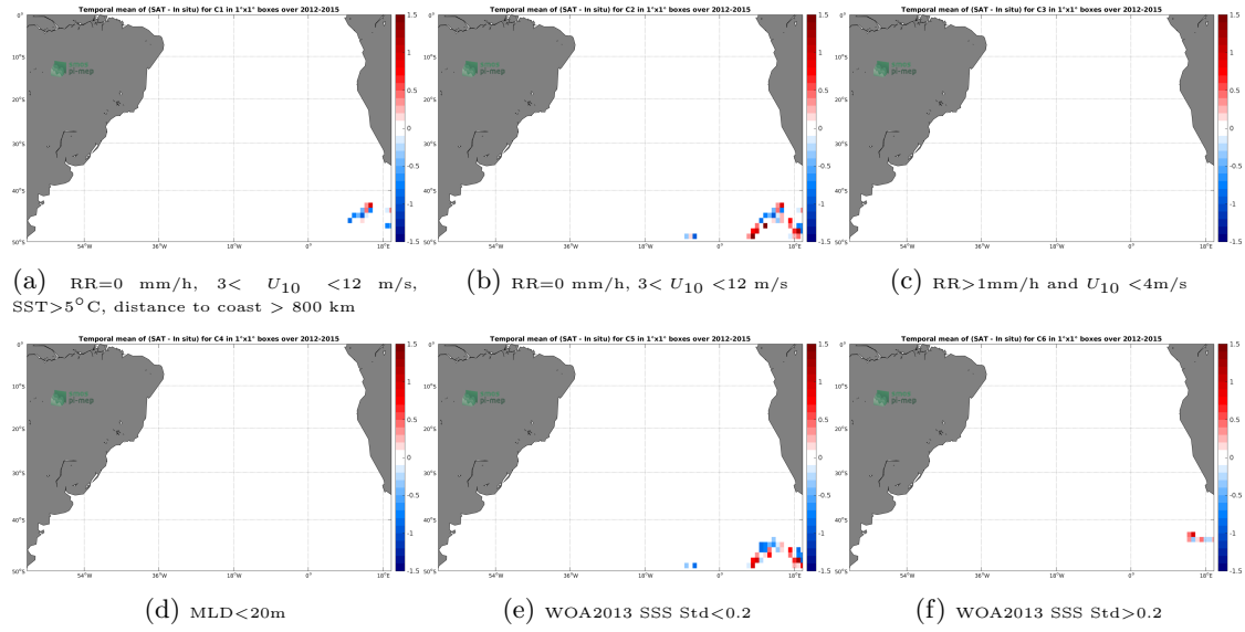
Figure 12: Temporal mean gridded over spatial boxes of size 1^\circ \times 1^\circ of \Delta SSS (SMOS-L3-ICDC-V3-MONTHLY-0.5DEG - Sea mammals) for 6 different subdatasets corresponding to: RR=0 mm/h, 3 < U_{10} < 12 m/s, SST > 5^\circ C , distance to coast > 800 km (a), RR=0 mm/h, 3 < U_{10} < 12 m/s (b), RR > 1 mm/h and U_{10} < 4 m/s (c), MLD < 20 m (d), WOA2013 SSS Std < 0.2 (e), WOA2013 SSS Std > 0.2 (f).
