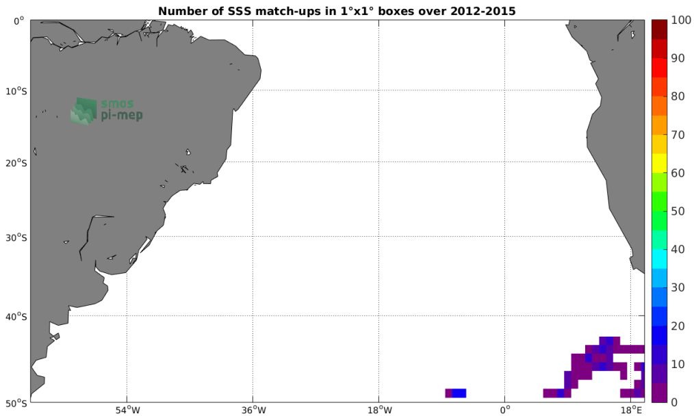
Figure 4: Number of SSS match-ups between Sea mammals SSS and the SMOS-L3-ICDC-V3-MONTHLY-0.5DEG SSS product for the South Atlantic Ocean Pi-MEP region over 1^\circ \times 1^\circ boxes and for the full satellite product period.
