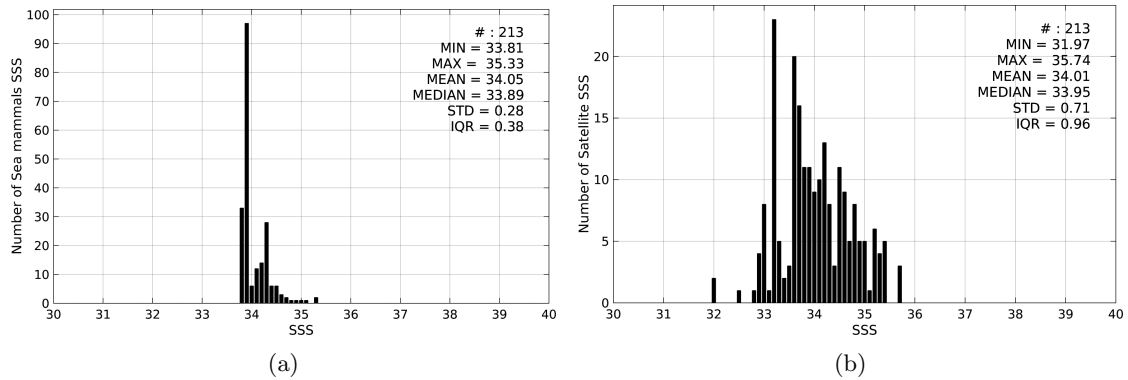
Figure 2: Histograms of SSS from Sea mammals (a) and SMOS-L3-ICDC-V3-MONTHLY-0.5DEG (b) considering all match-up pairs per bins of 0.1 over the South Atlantic Ocean Pi-MEP region and for the full satellite product period.
