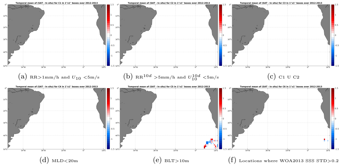
Figure 12: Temporal mean gridded over spatial boxes of size 1^\circ \times 1^\circ of \Delta SSS (SMOS-L3-ICDC-V3-MONTHLY-0.5DEG - Sea mammals) for 6 different subdatasets corresponding to: RR > 1\text{mm/h} and U_{10} < 5\text{m/s} (a), RR^{10d} > 5\text{mm/h} and U_{10}^{10d} < 5\text{m/s} (b), C1 \cup C2 (c), MLD < 20\text{m} (d), BLT > 10\text{m} (e), Locations where WOA2013 SSS STD > 0.2 (f).
