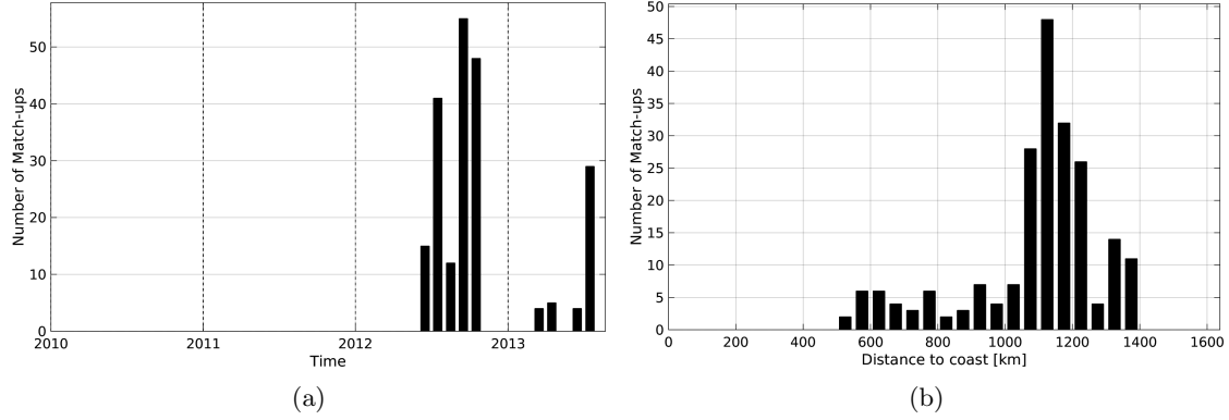
Figure 1: Number of match-ups between Sea mammals and SMOS-L3-ICDC-V3-MONTHLY-0.5DEG SSS as a function of time (a) and as function of the distance to coast (b) over the South Atlantic Ocean Pi-MEP region and for the full satellite product period.
