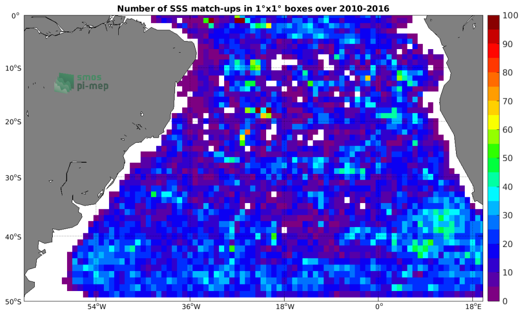
Figure 4: Number of SSS match-ups between Argo SSS and the SMOS SSS L3 v3 Monthly (ICDC) SSS product for the South Atlantic Ocean Pi-MEP region over 1°x1° boxes and for the full satellite product period.
