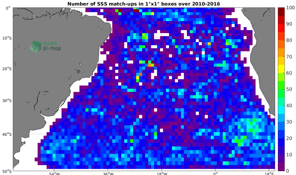
Figure 4: Number of SSS match-ups between Argo SSS and the SMOS-L3-ICDC-V3-MONTHLY-0.5DEG SSS product for the South Atlantic Ocean Pi-MEP region over 1°x1° boxes and for the full satellite product period.
