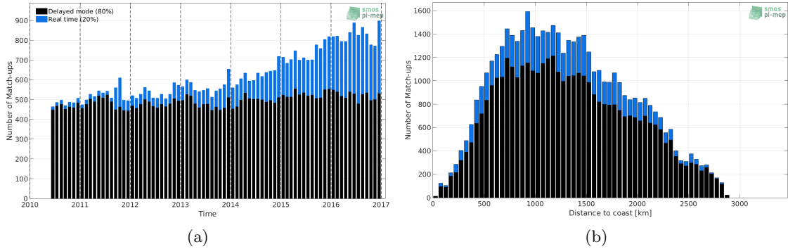
Figure 1: Number of match-ups between Argo and SMOS-L3-ICDC-V3-MONTHLY-0.5DEG SSS as a function of time (a) and as function of the distance to coast (b) over the South Atlantic Ocean Pi-MEP region and for the full satellite product period.
