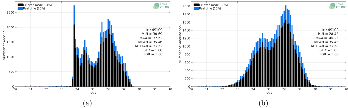
Figure 2: Histograms of SSS from Argo (a) and SMOS-L3-ICDC-V3-MONTHLY-0.5DEG (b) considering all match-up pairs per bins of 0.1 over the South Atlantic Ocean Pi-MEP region and for the full satellite product period.
