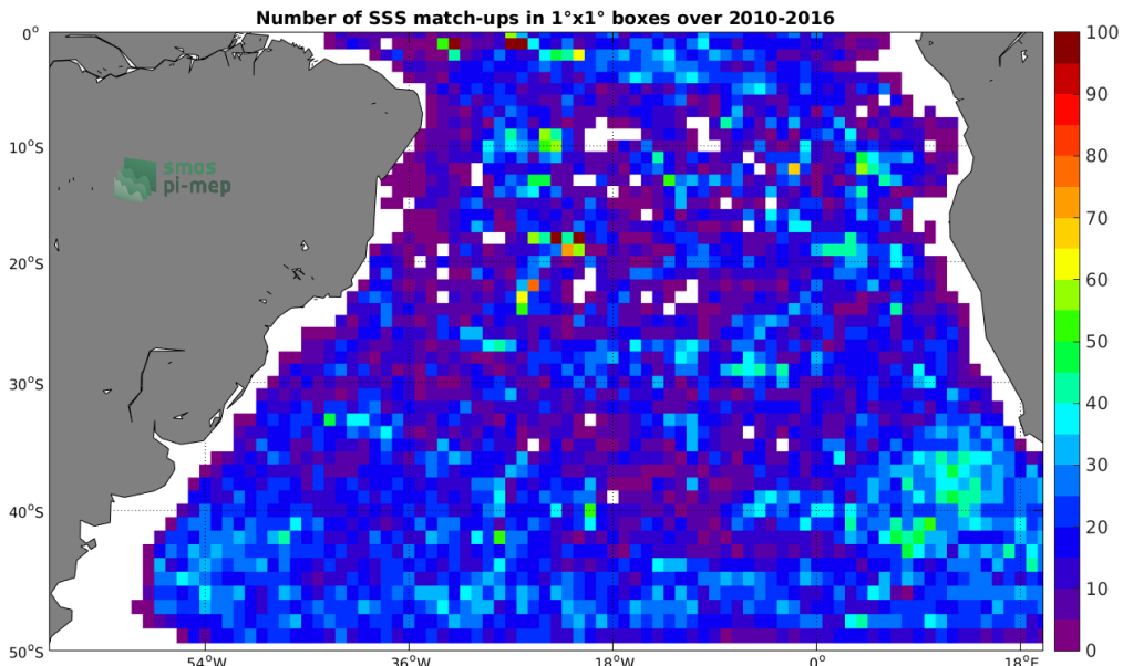
Figure 4: Number of SSS match-ups between Argo SSS and the SMOS-L3-ICDC-V3-MONTHLY-0.5DEG SSS product for the South Atlantic Ocean Pi-MEP region over 1^\circ \times 1^\circ boxes and for the full satellite product period.
