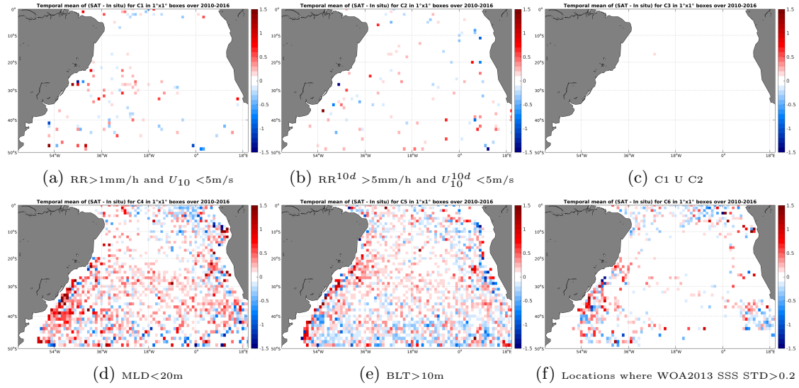
Figure 12: Temporal mean gridded over spatial boxes of size 1^\circ \times 1^\circ of \Delta SSS (SMOS-L3-ICDC-V3-MONTHLY-0.5DEG - Argo) for 6 different subdatasets corresponding to: RR > 1\text{mm/h} and U_{10} < 5\text{m/s} (a), RR^{10d} > 5\text{mm/h} and U_{10}^{10d} < 5\text{m/s} (b), C1 U C2 (c), MLD < 20\text{m} (d), BLT > 10\text{m} (e), Locations where WOA2013 SSS STD > 0.2 (f).
