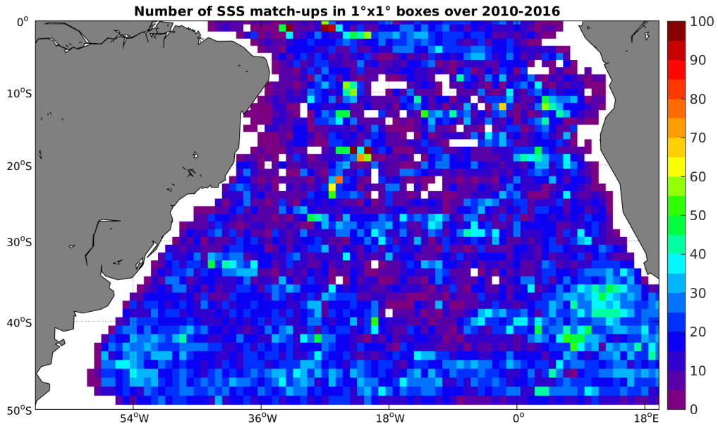
Figure 4: Number of SSS match-ups between Argo SSS and the SMOS-L3-ICDC-V3-MONTHLY-0.5DEG SSS product for the South Atlantic Ocean Pi-MEP region over 1^\circ \times 1^\circ boxes and for the full satellite product period.
