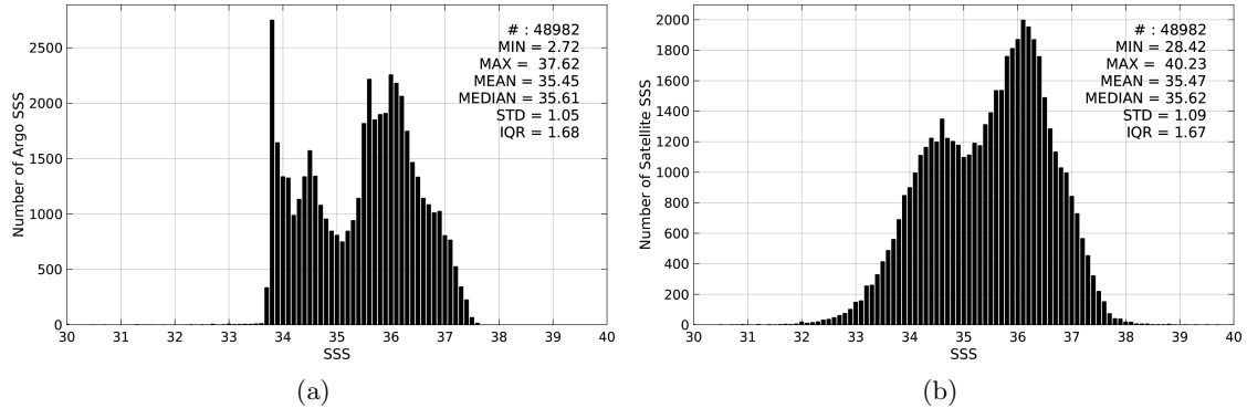
Figure 2: Histograms of SSS from Argo (a) and SMOS-L3-ICDC-V3-MONTHLY-0.5DEG (b) considering all match-up pairs per bins of 0.1 over the South Atlantic Ocean Pi-MEP region and for the full satellite product period.
