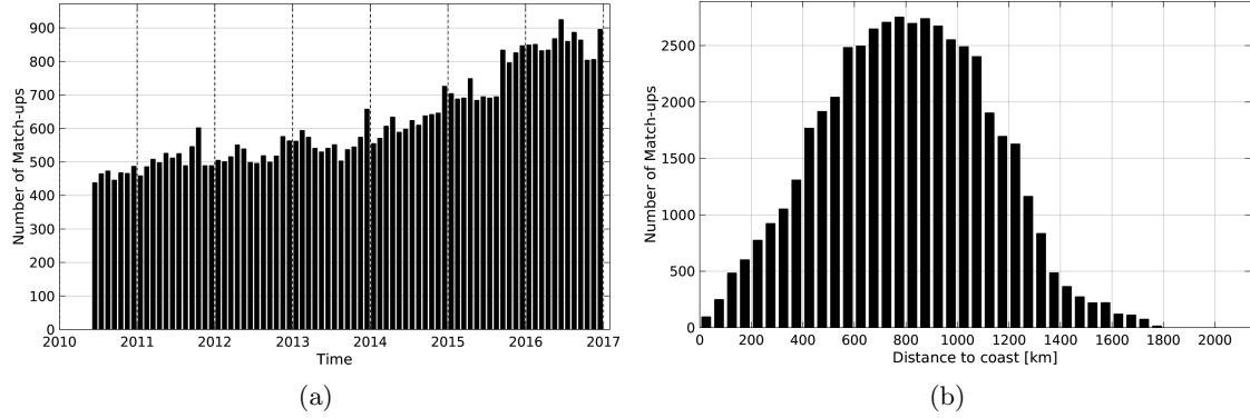
Figure 1: Number of match-ups between Argo and SMOS-L3-ICDC-V3-MONTHLY-0.5DEG SSS as a function of time (a) and as function of the distance to coast (b) over the South Atlantic Ocean Pi-MEP region and for the full satellite product period.
