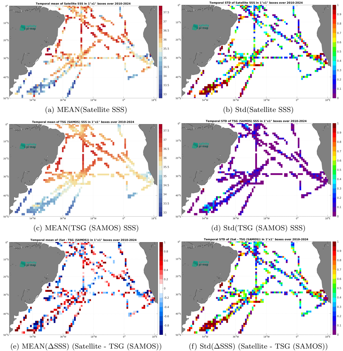
Figure 7: Temporal mean (left) and Std (right) of SSS from SMOS SSS L2Q v331 - With FLAG (CMEMS-CATDS-CPDC) (top), TSG (SAMOS) (middle), and of \Delta SSS (Satellite - TSG (SAMOS)). Only match-up pairs are used to generate these maps.
