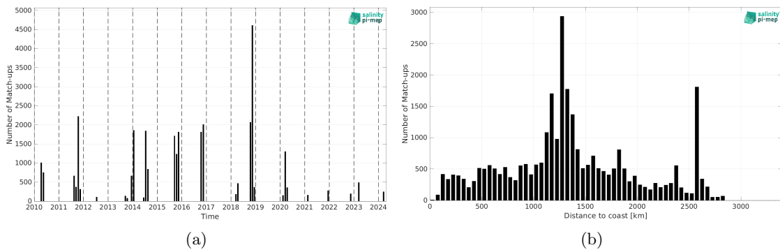
Figure 2: Number of match-ups between TSG (SAMOS) and SMOS SSS L2Q v331 - With FLAG (CMEMS-CATDS-CPDC) SSS as a function of time (a) and as function of the distance to coast (b) over the South Atlantic Ocean Pi-MEP region and for the full satellite product period.
