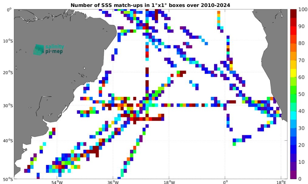
Figure 5: Number of SSS match-ups between TSG (SAMOS) SSS and the SMOS SSS L2Q v331 - With FLAG (CMEMS-CATDS-CPDC) SSS product for the South Atlantic Ocean Pi-MEP region over 1^\circ \times 1^\circ boxes and for the full satellite product period.
