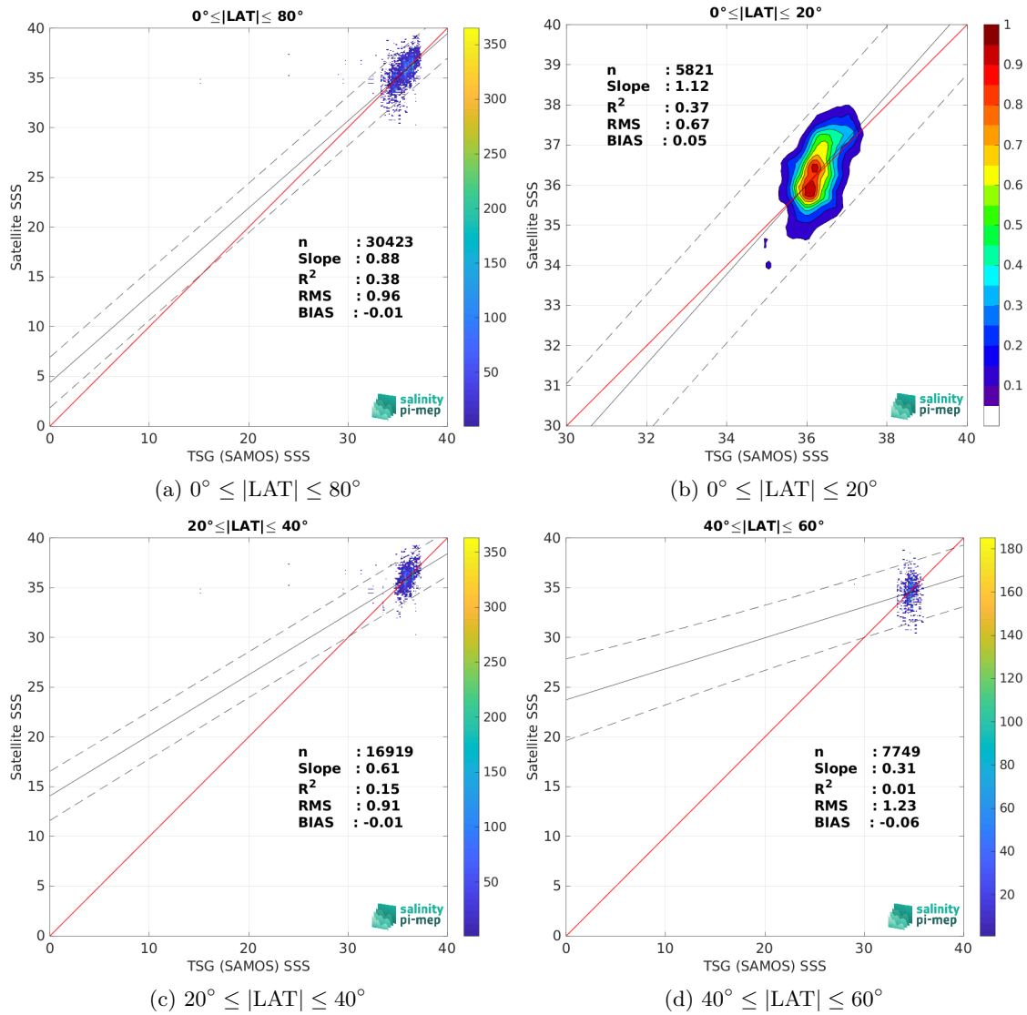
Figure 10: Contour maps of the concentration of SMOS SSS L2Q v331 - With FLAG (CMEMS-CATDS-CPDC) SSS (y-axis) versus TSG (SAMOS) SSS (x-axis) at match-up pairs for different latitude bands. For each plot, the red line shows x=y . The black thin and dashed lines indicate a linear fit through the data cloud and the \pm 95\% confidence levels, respectively. The number of match-up pairs n , the slope and R^2 coefficient of the linear fit, the root mean square (RMS) and the mean bias between satellite and in situ data are indicated for each latitude band in each plot.
