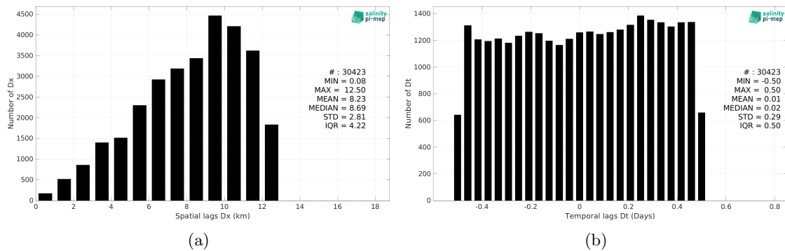
Figure 6: Histograms of the spatial (a) and temporal (b) lags between the location/time of the TSG (SAMOS) measurement and the date of the corresponding SMOS SSS L2Q v331 - With FLAG (CMEMS-CATDS-CPDC) SSS pixel.
