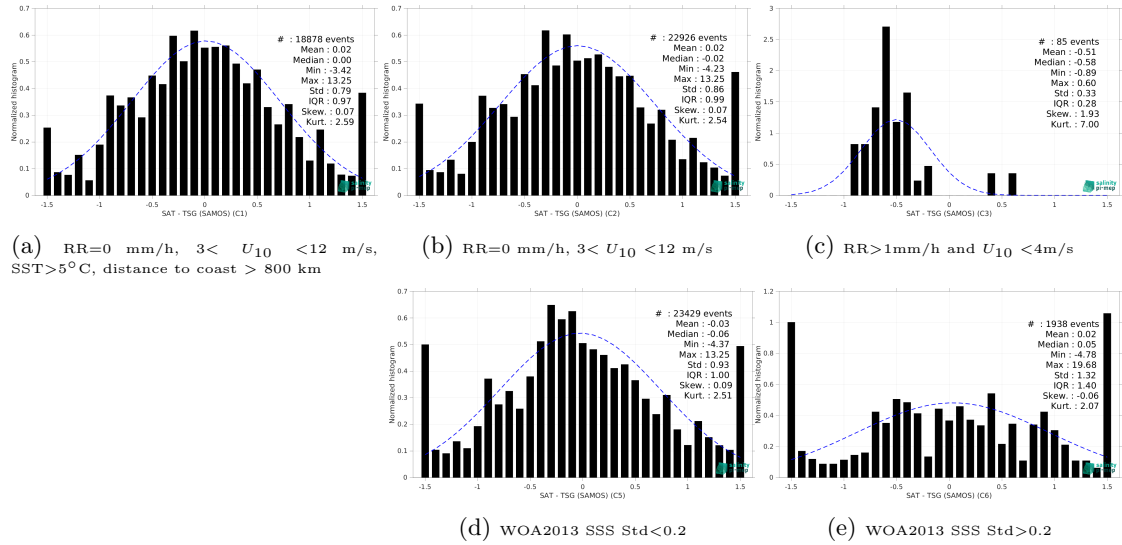
Figure 15: Normalized histogram of \Delta SSS (SMOS SSS L2Q v331 - With FLAG (CMEMS-CATDS-CPDC) - TSG (SAMOS)) for 5 different subdatasets corresponding to: RR=0 mm/h, 3 < U_{10} < 12 m/s, SST>5°C, distance to coast > 800 km (a), RR=0 mm/h, 3 < U_{10} < 12 m/s (b), RR>1mm/h and U_{10} < 4 m/s (c), WOA2013 SSS Std<0.2 (d), WOA2013 SSS Std>0.2 (e).
