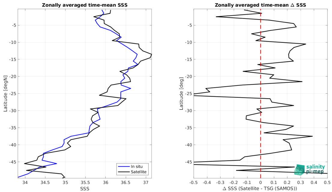
Figure 9: Left panel: Zonal mean SSS from SMOS SSS L2Q v331 - With FLAG (CMEMS-CATDS-CPDC) satellite product (black) and from TSG (SAMOS) (blue). Right panel: Zonal mean of \Delta SSS (Satellite - TSG (SAMOS)) for all the collected Pi-MEP match-up pairs estimated over the full satellite product period.
