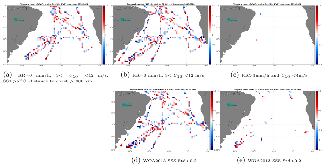
Figure 14: Temporal mean gridded over spatial boxes of size 1^\circ \times 1^\circ of \Delta SSS (SMOS SSS L2Q v331 - With FLAG (CMEMS-CATDS-CPDC) - TSG (SAMOS)) for 5 different subdatasets corresponding to:RR=0 mm/h, 3 < U_{10} < 12 m/s, SST >5^\circ\text{C} , distance to coast > 800 km (a), RR=0 mm/h, 3 < U_{10} < 12 m/s (b), RR >1 mm/h and U_{10} < 4 m/s (c), WOA2013 SSS Std <0.2 (d), WOA2013 SSS Std >0.2 (e).
