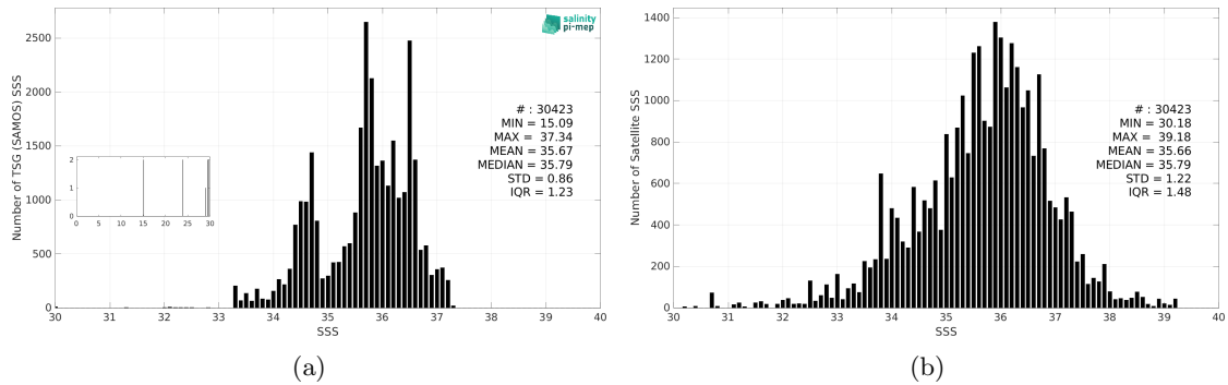
Figure 3: Histograms of SSS from TSG (SAMOS) (a) and SMOS SSS L2Q v331 - With FLAG (CMEMS-CATDS-CPDC) (b) considering all match-up pairs per bins of 0.1 over the South Atlantic Ocean Pi-MEP region and for the full satellite product period.
