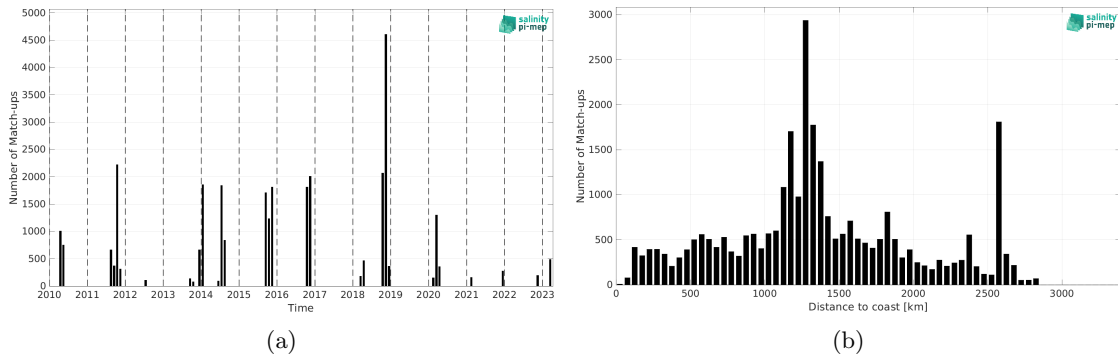
Figure 1: Number of match-ups between TSG (SAMOS) and SMOS SSS L2Q v331 - With FLAG (CMEMS-CATDS-CPDC) SSS as a function of time (a) and as function of the distance to coast (b) over the South Atlantic Ocean Pi-MEP region and for the full satellite product period.
