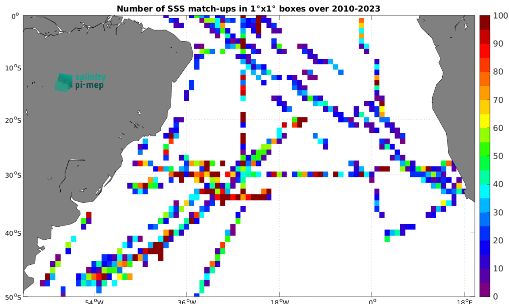
Figure 4: Number of SSS match-ups between TSG (SAMOS) SSS and the SMOS SSS L2Q v331 - With FLAG (CMEMS-CATDS-CPDC) SSS product for the South Atlantic Ocean Pi-MEP region over 1^\circ \times 1^\circ boxes and for the full satellite product period.
