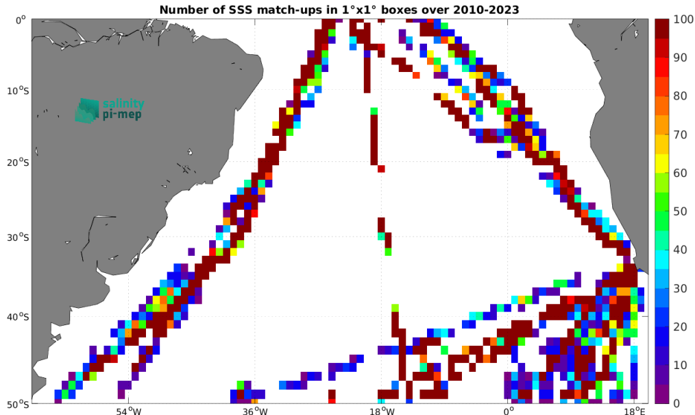
Figure 5: Number of SSS match-ups between TSG (Polarstern) SSS and the SMOS SSS L2Q v331 - With FLAG (CMEMS-CATDS-CPDC) SSS product for the South Atlantic Ocean Pi-MEP region over 1^\circ \times 1^\circ boxes and for the full satellite product period.
