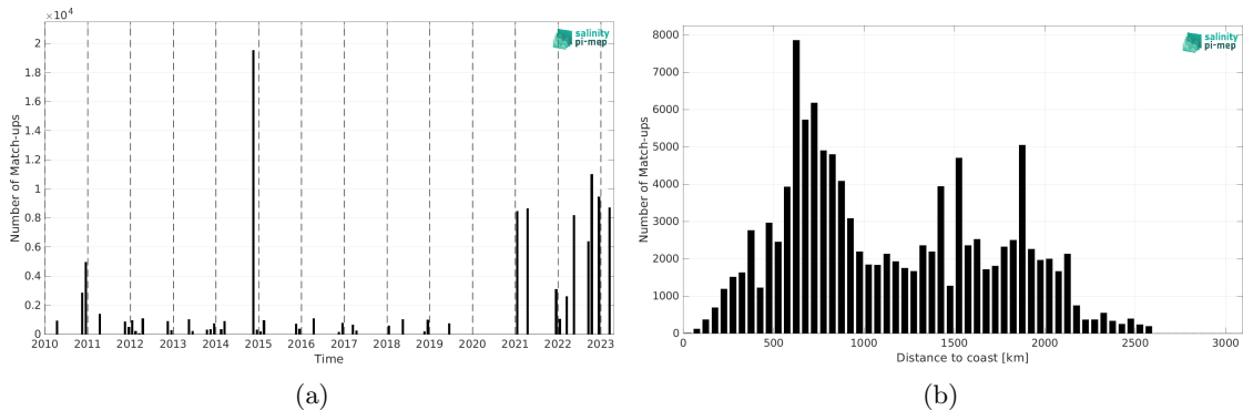
Figure 2: Number of match-ups between TSG (Polarstern) and SMOS SSS L2Q v331 - With FLAG (CMEMS-CATDS-CPDC) SSS as a function of time (a) and as function of the distance to coast (b) over the South Atlantic Ocean Pi-MEP region and for the full satellite product period.
