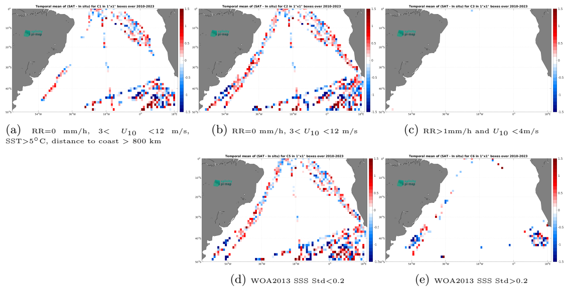
Figure 14: Temporal mean gridded over spatial boxes of size 1^\circ \times 1^\circ of \Delta SSS (SMOS SSS L2Q v331 - With FLAG (CMEMS-CATDS-CPDC) - TSG (Polarstern)) for 5 different subdatasets corresponding to:RR=0 mm/h, 3 < U_{10} < 12 m/s, SST>5°C, distance to coast > 800 km (a), RR=0 mm/h, 3 < U_{10} < 12 m/s (b), RR>1mm/h and U_{10} < 4 m/s (c), WOA2013 SSS Std<0.2 (d), WOA2013 SSS Std>0.2 (e).
