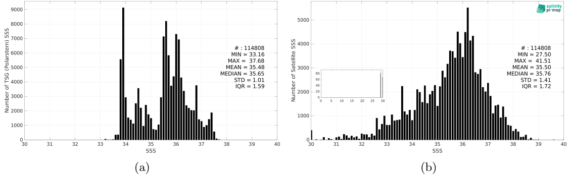
Figure 3: Histograms of SSS from TSG (Polarstern) (a) and SMOS SSS L2Q v331 - With FLAG (CMEMS-CATDS-CPDC) (b) considering all match-up pairs per bins of 0.1 over the South Atlantic Ocean Pi-MEP region and for the full satellite product period.
